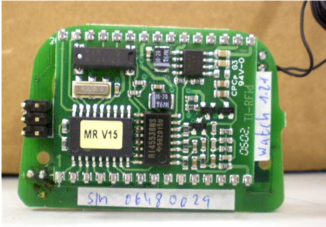
Photograph No.5 Watch ID RF card close view
