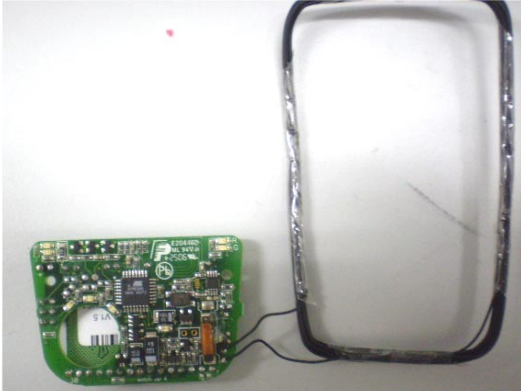
Photograph No.3 Watch ID main PCB with loop antenna front view
