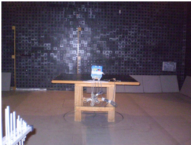
Photograph No.4 Setup for spurious emission measurements in the anechoic chamber from 30 to 1000 MHz, EUT: sensomatic with internal antenna
