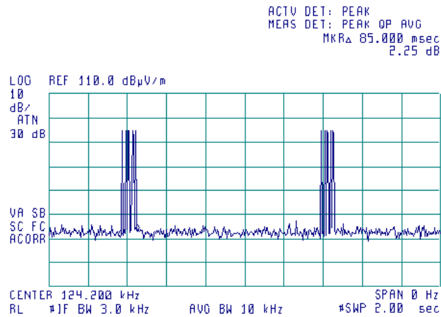
Plot 7.1.22 Transmission burst period
