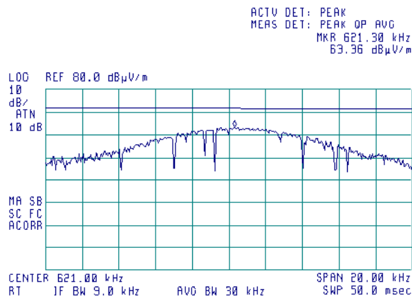
Plot 7.1.12 Radiated emission measurements at the sixth harmonic frequency
