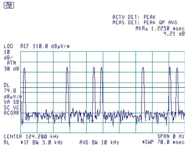
Plot 7.1.17 Transmission pulse duration
