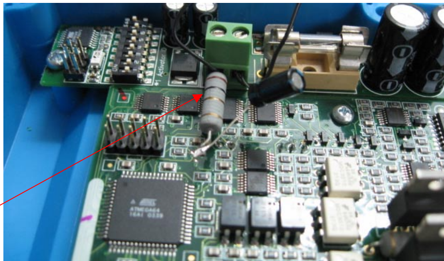
Photograph 7.2.2 Antenna assembly
