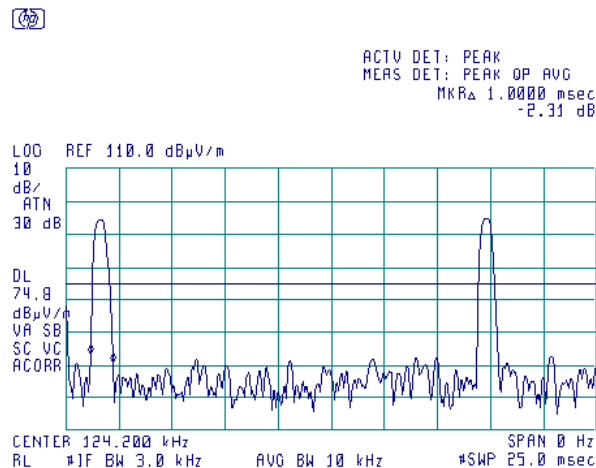
Plot 7.1.18 Transmission pulse duration
