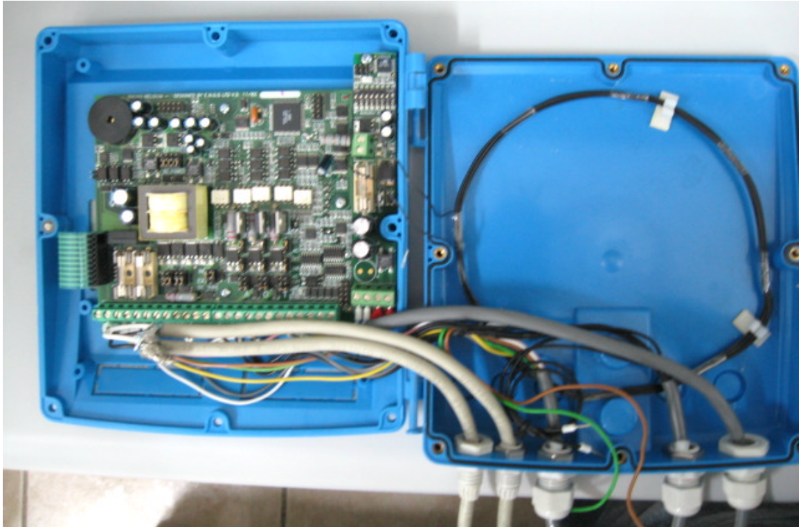
Photograph No.1 Sensomatic general internal view
