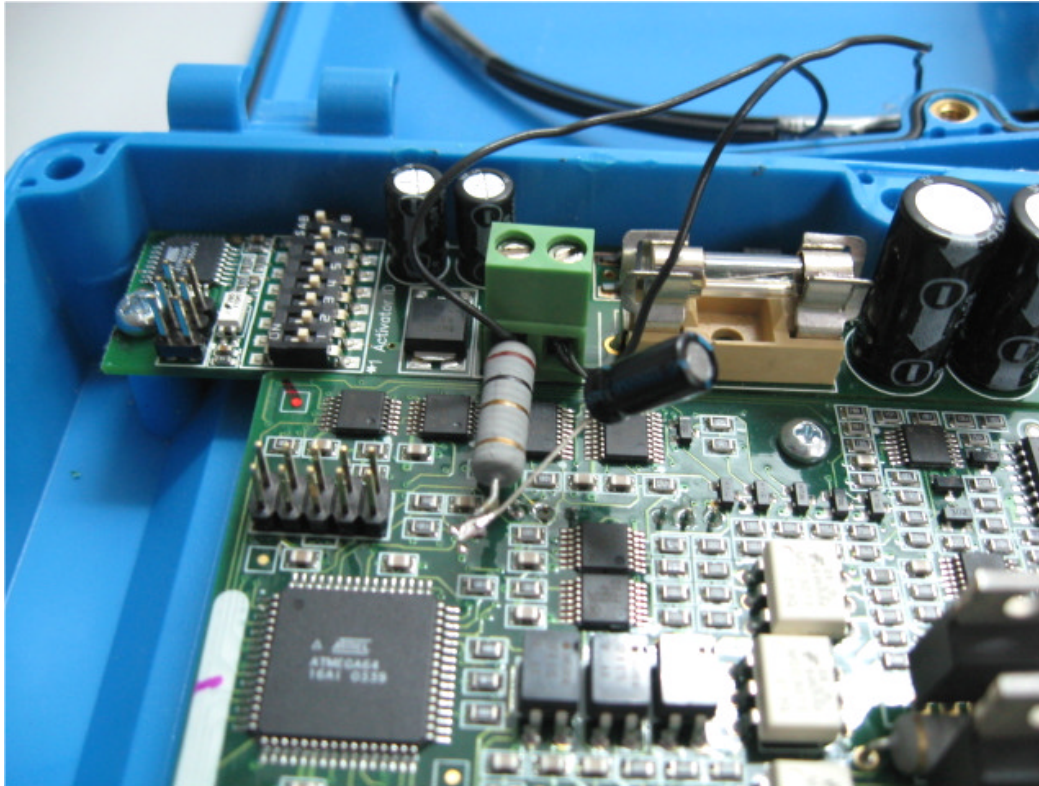
Photograph No.2 Sensomatic close internal view
