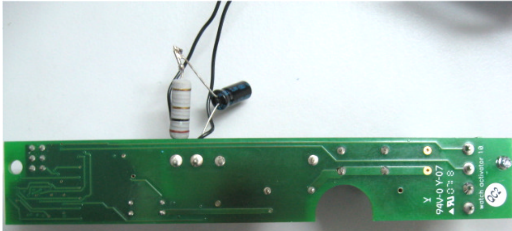
Photograph No.8 RF card second side view
