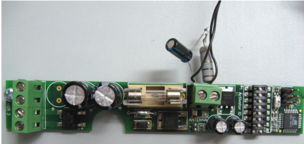
Photograph No.6 RF card front view
