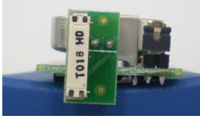
Photograph No.5 Tag second PCB view
