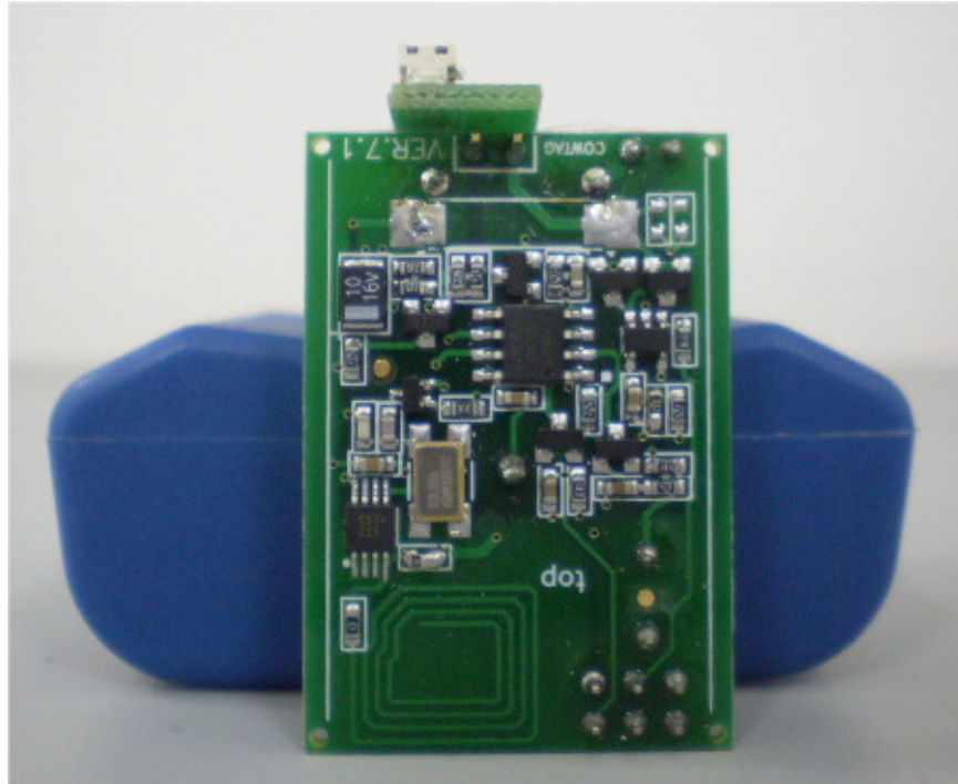
Photograph No.2 Tag PCB component side view
