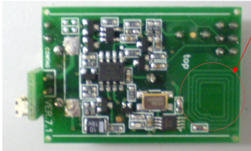
Photograph No.6 Tag PCB close view
