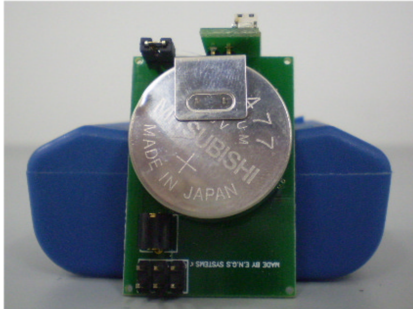
Photograph No.3 Tag PCB second side view
