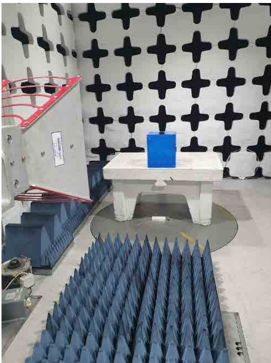
Radiated emissions test set up above 1GHz.
