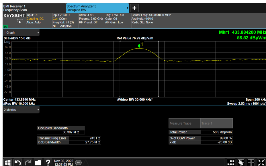
Plot # 10. Occupied bandwidth test result
