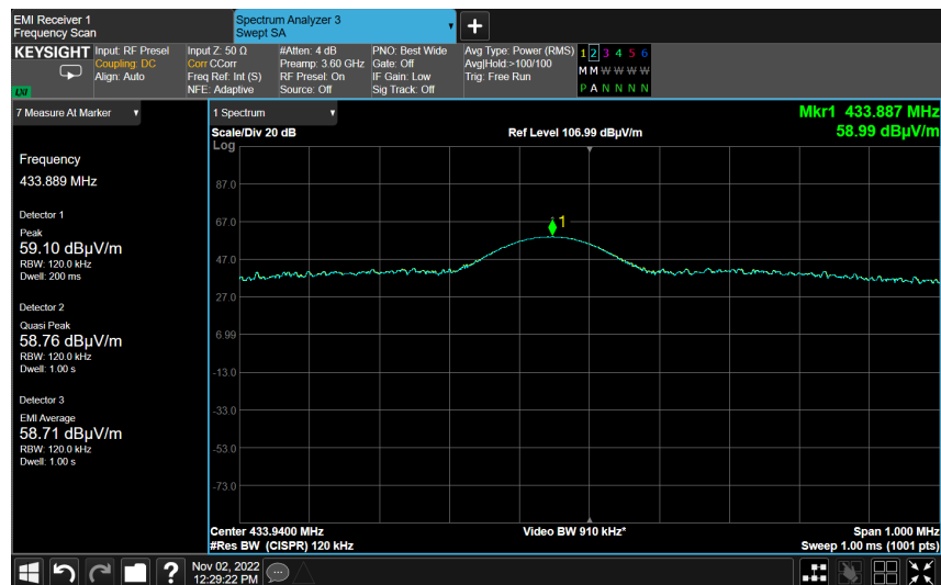
Plot # 1. Carrier frequency 433.92 MHz.
