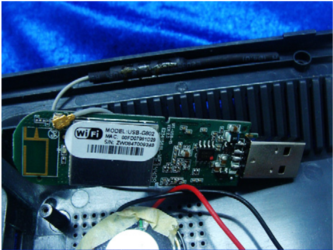
WLAN Card
