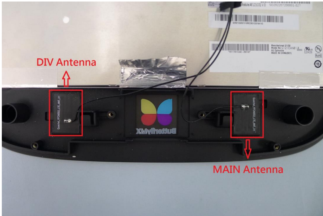
( 48 ) EUT Photo_BUTTERFLYMX.M12.1
