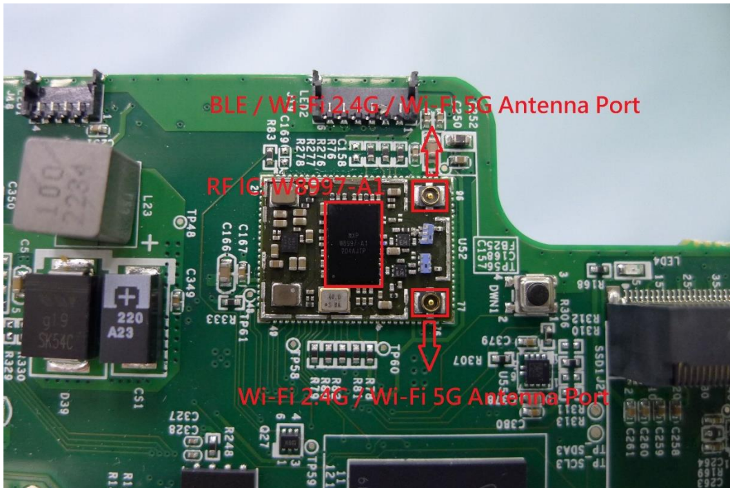
( 22 ) EUT Photo_BUTTERFLYMX.M12.1
