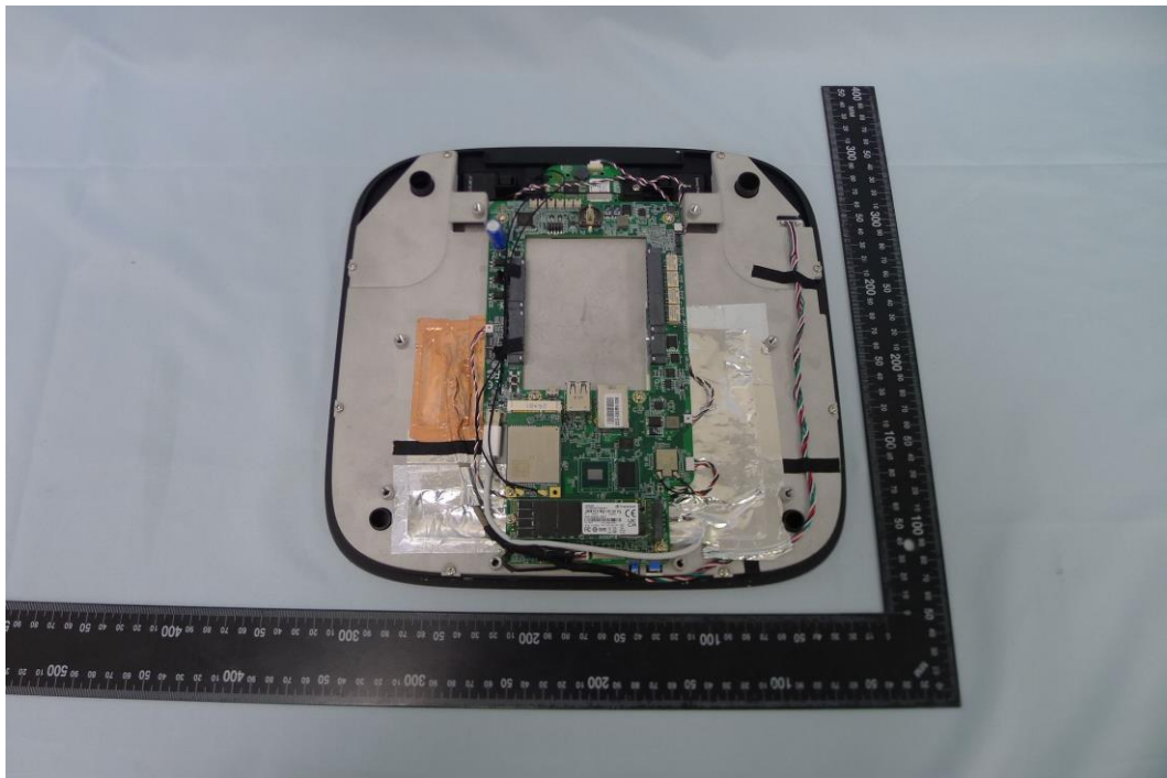
( 2 ) EUT Photo_BUTTERFLYMX.M12.1
