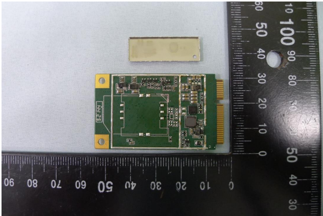
( 14 ) EUT Photo_BUTTERFLYMX.M12.1
