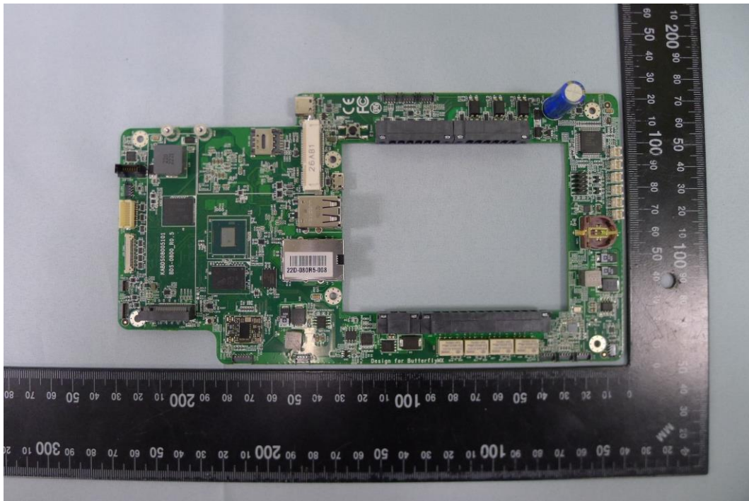
( 20 ) EUT Photo_BUTTERFLYMX.M12.1
