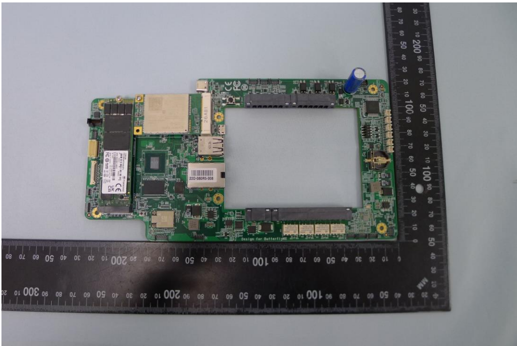
( 4 ) EUT Photo_BUTTERFLYMX.M12.1
