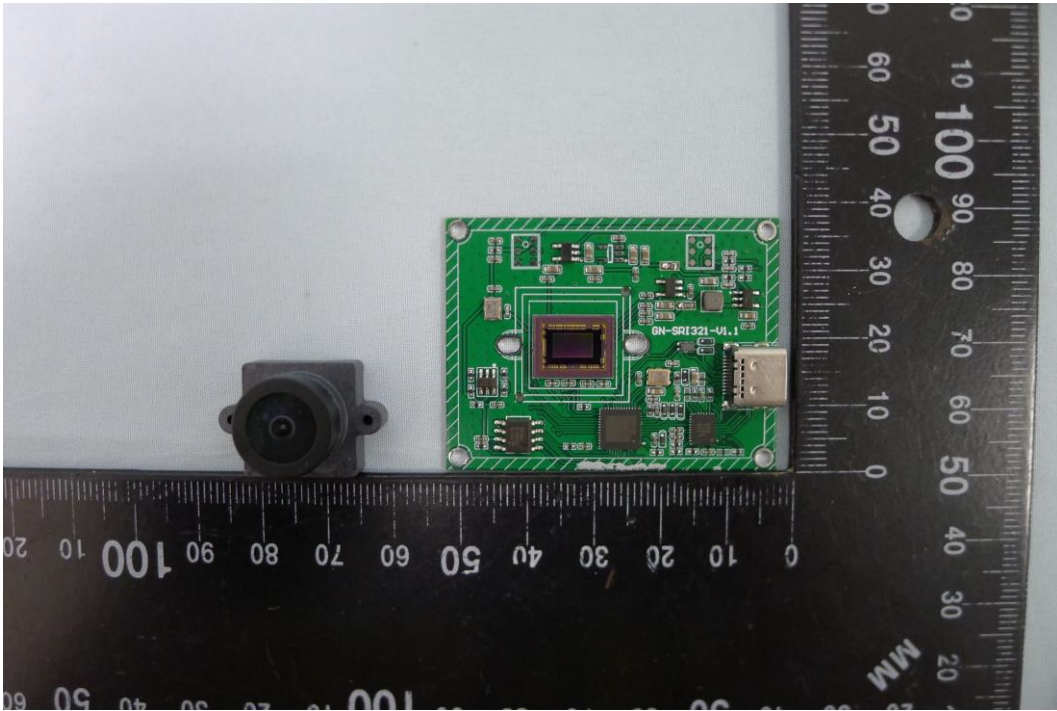
( 30 ) EUT Photo_BUTTERFLYMX.M12.1
