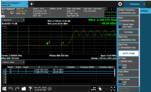
CH00 (2402MHz) 3-DH5(3Mbps)
