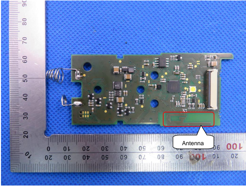
Fig.9 -main board view (type: HC42BL11S000100)
