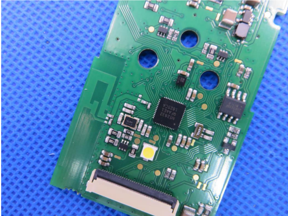
Fig.33 -main board view (type: HC42BL01S000100)
