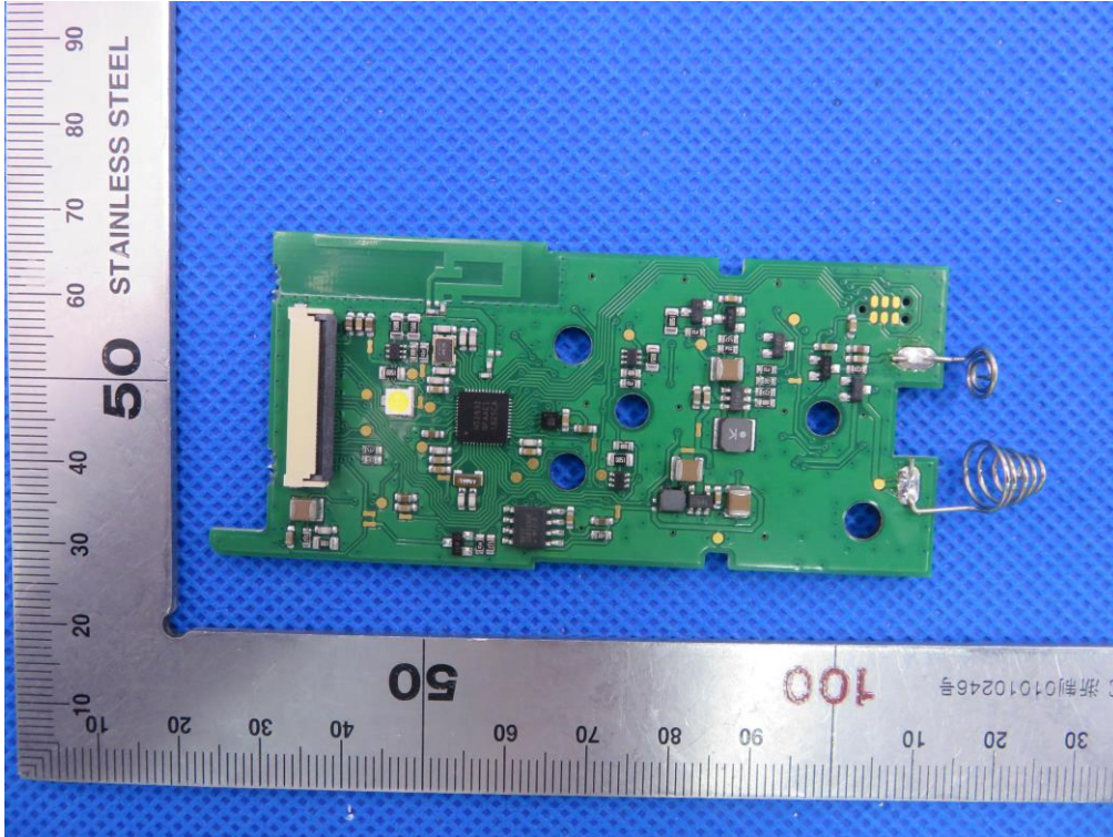
Fig.31 -main board view (type: HC42BL01S001000)
