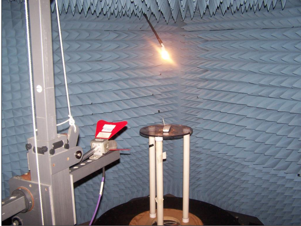
Photograph 3. Radiated Spurious Emissions, Test Setup, 1 GHz – 5 GHz
