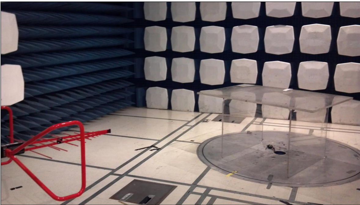
Photograph 2. Fundamental Field Strength & Harmonic Emission, Test Setup
