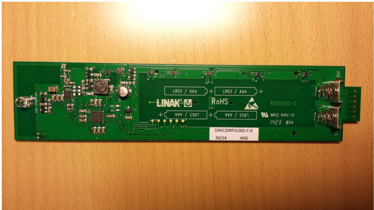
HC20 PCB
