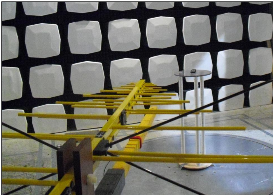
Photograph 2. Field Strength of Fundamental and Harmonics, Test Setup
