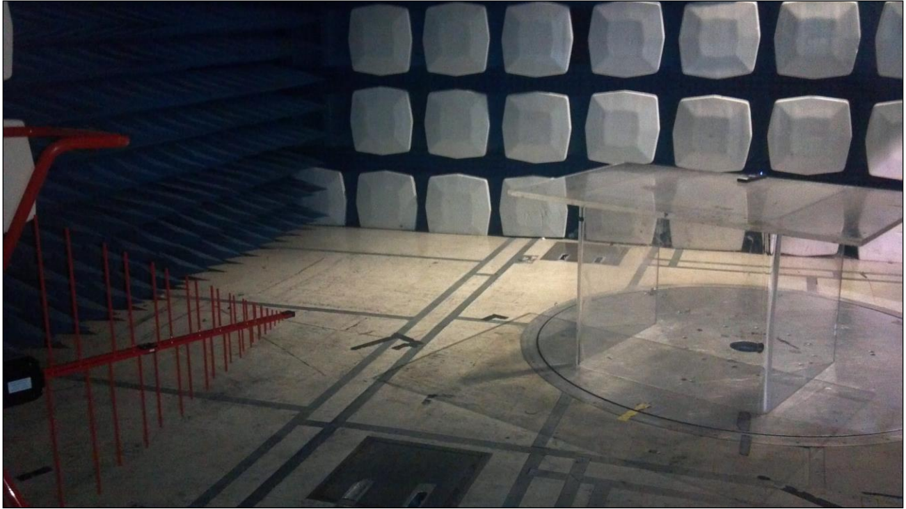
Photograph 1. Radiated Emission, Test Setup
