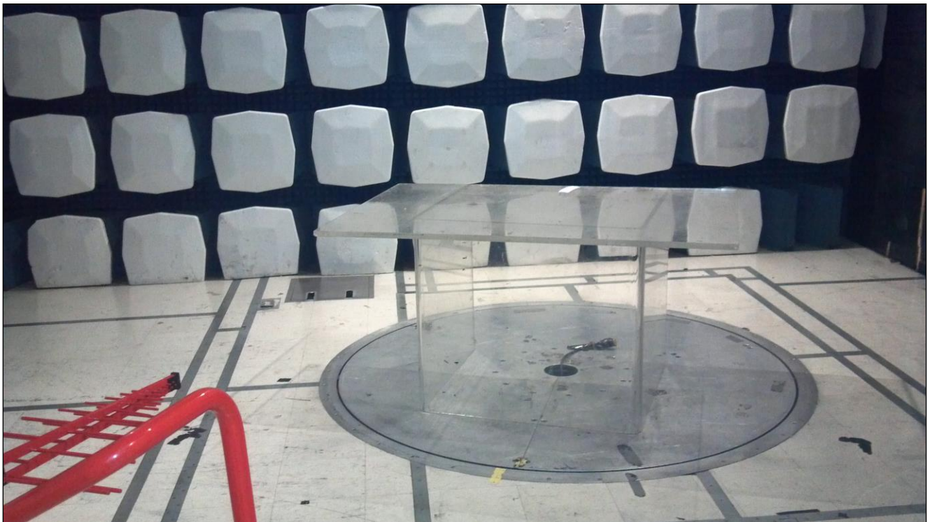
Photograph 2. Fundamental Field Strength, Harmonic/Spurious Emission 1-5GHz Test Setup
