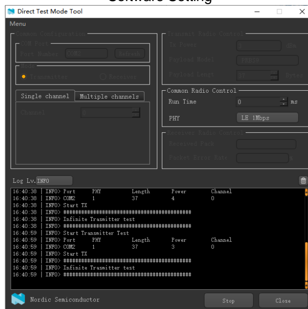
Software Setting
