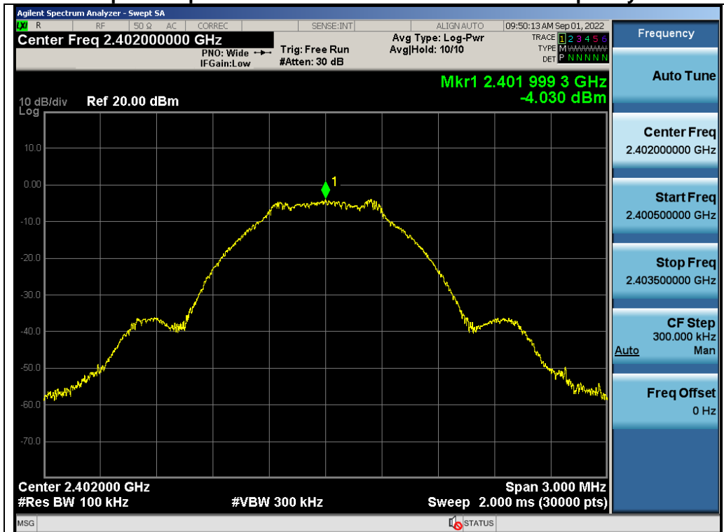
Test_Graph_BLE1M_ANT1_2402_1Mbps_Reference Level
