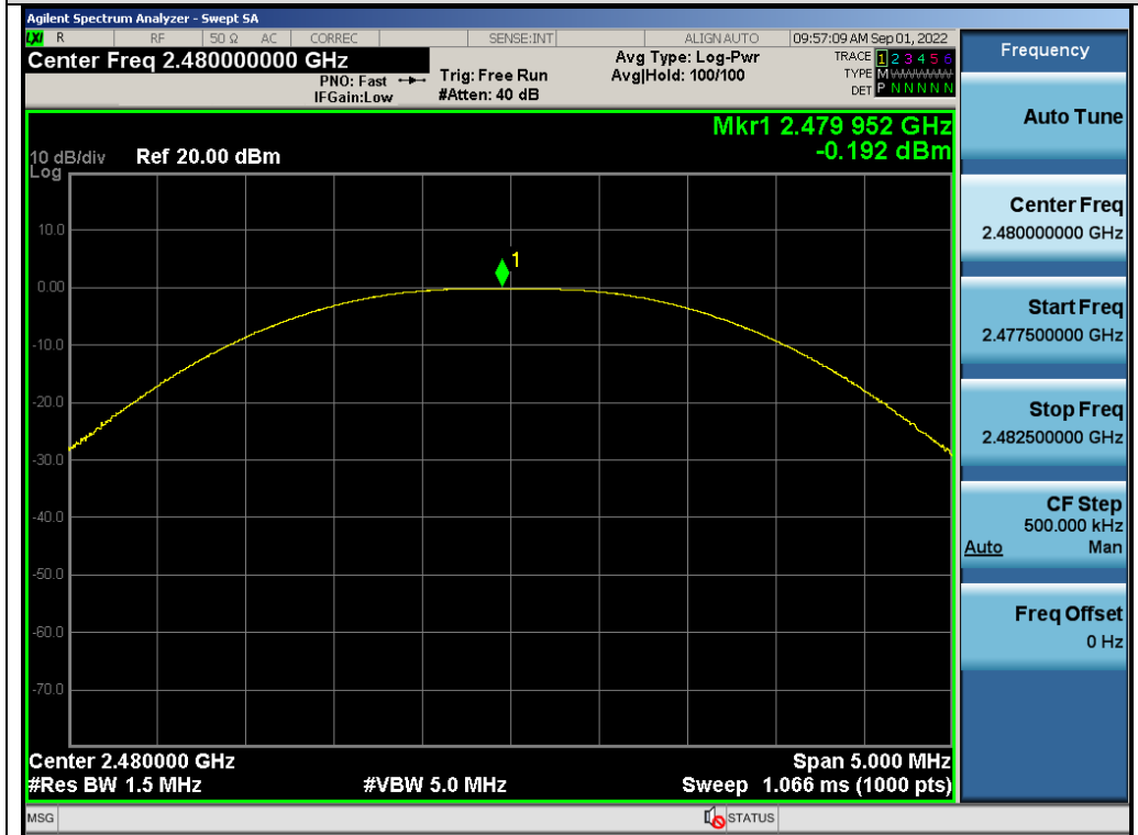
Test_Graph_BLE1M_ANT1_2480_1Mbps_Peak Power
