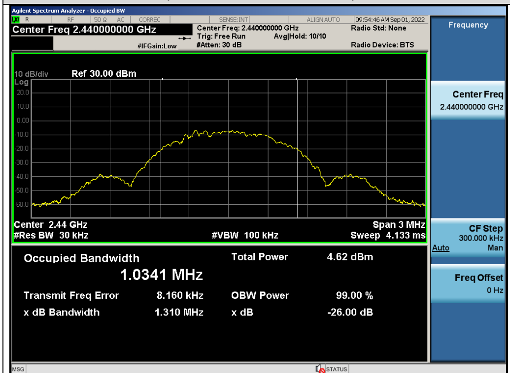
Test_Graph_BLE1M_ANT1_2440_1Mbps_OBW
