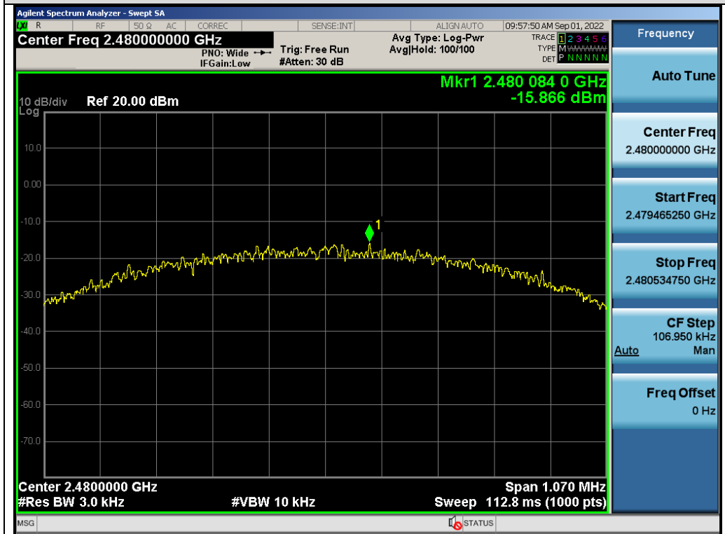
Test_Graph_BLE1M_ANT1_2480_1Mbps_PSD
