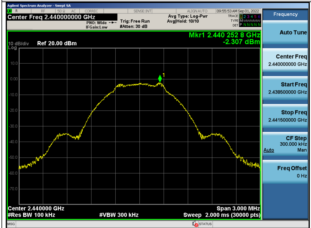
Test_Graph_BLE1M_ANT1_2440_1Mbps_Reference Level
