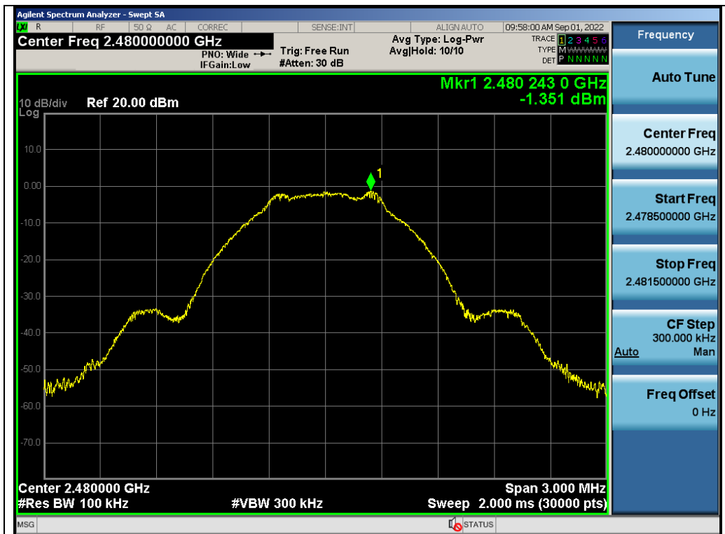
Test_Graph_BLE1M_ANT1_2480_1Mbps_Reference Level
