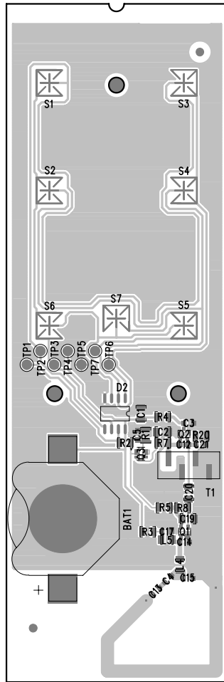
26 Top Overlay
