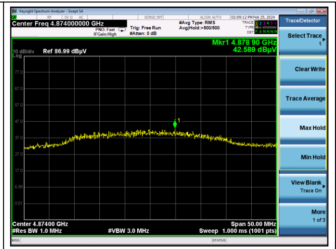
Middle channel 2 nd Spurious (Peak)
