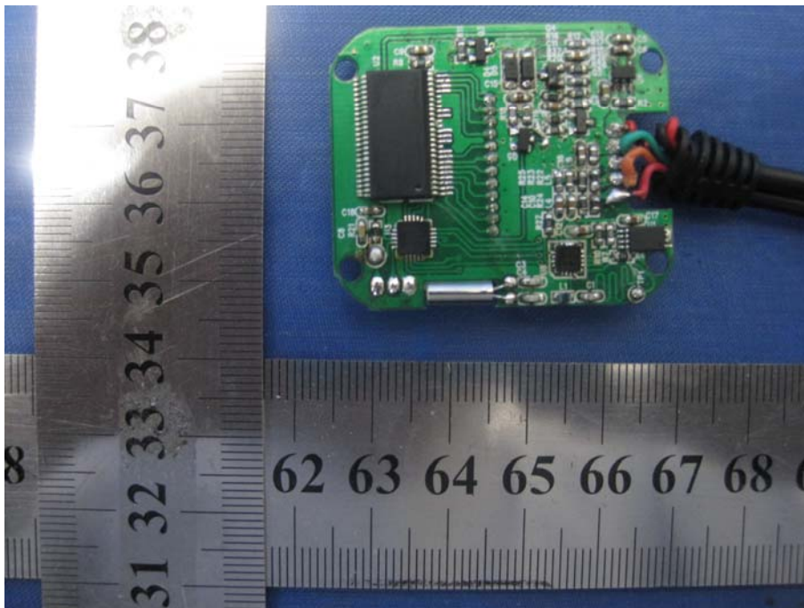
PCB-Back View(2)
