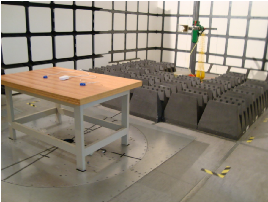
Radiated Emissions - Front View (Above 1 GHz, powered by battery)
