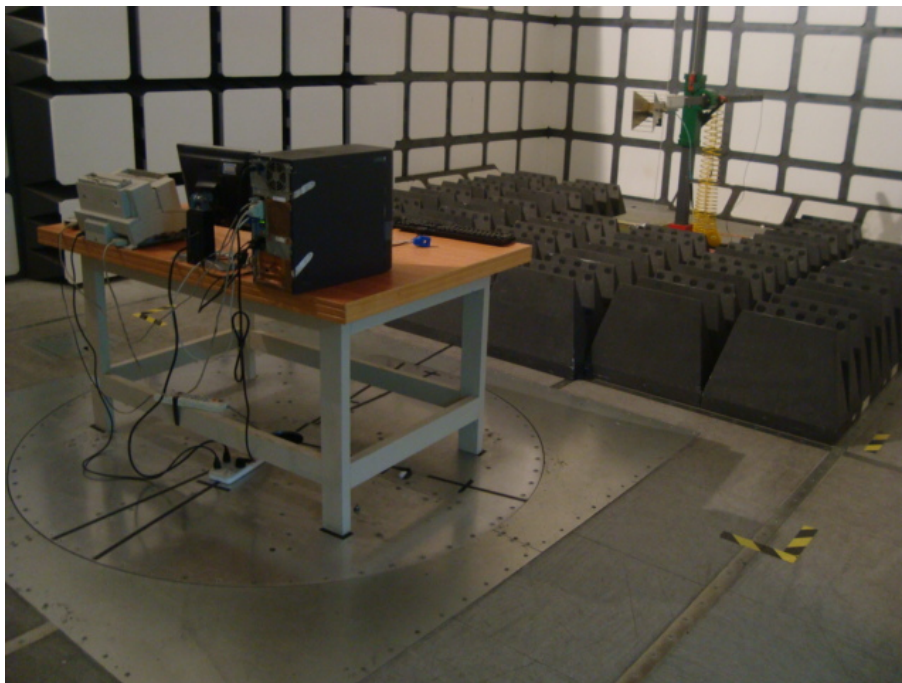
Radiated Emissions - Rear View (Above 1 GHz, powered by PC)
