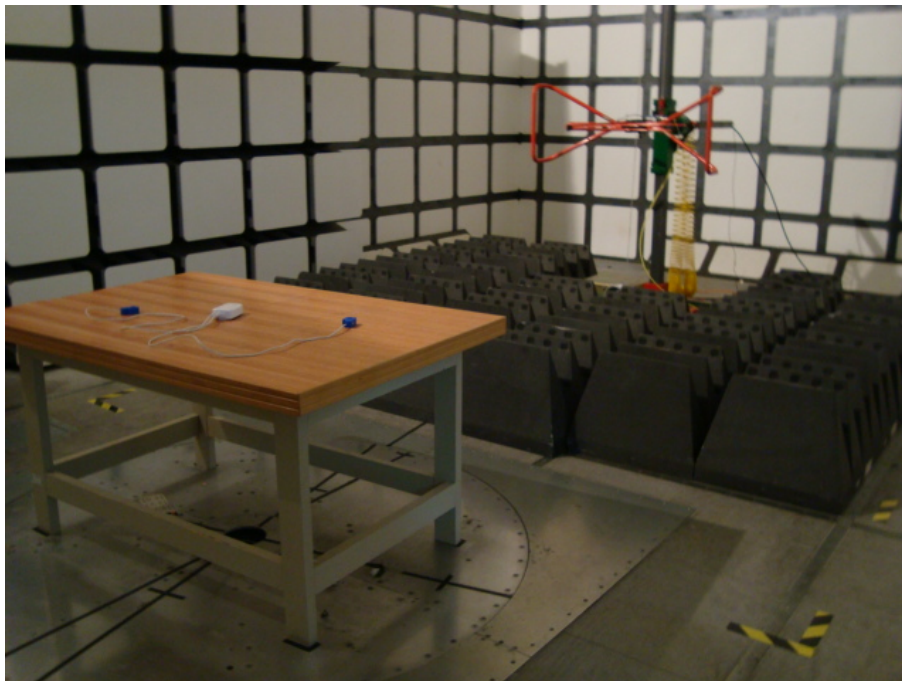
Radiated Emissions - Rear View (Below 1 GHz, powered by battery)
