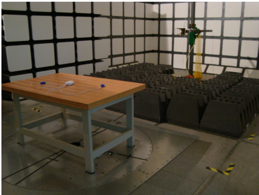
Radiated Emissions - Rear View (Above 1 GHz, powered by battery)
