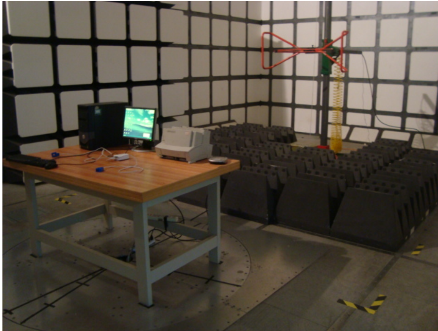
Radiated Emissions - Front View (Below 1 GHz, powered by PC)
