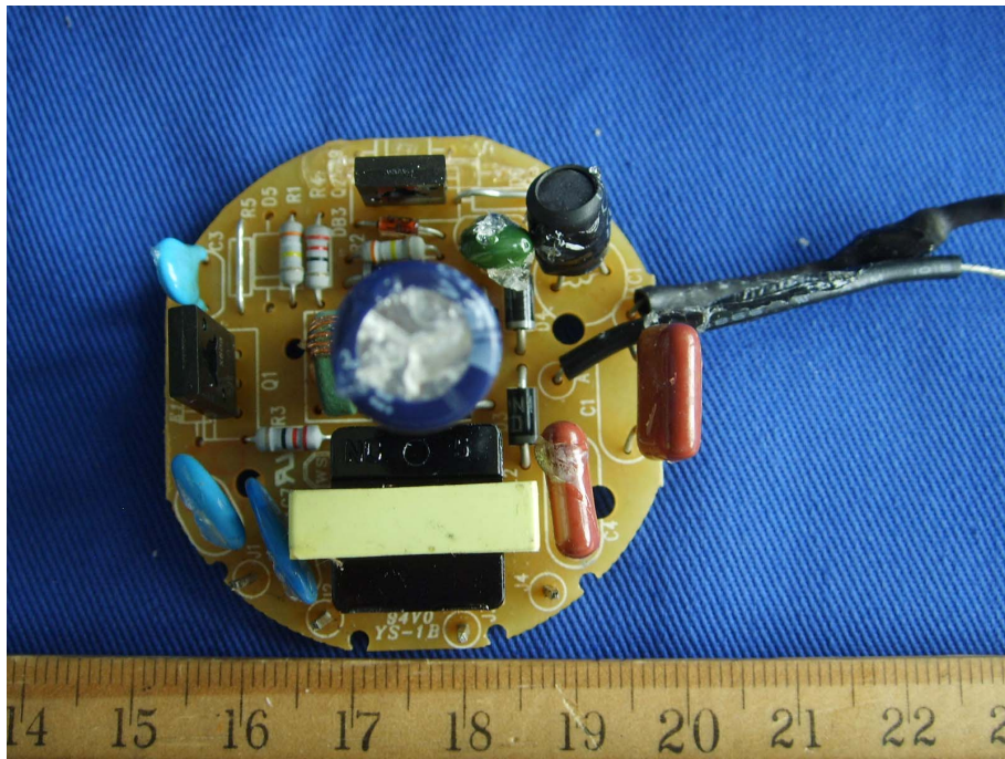
EUT –Components View (LTEA-24W)
