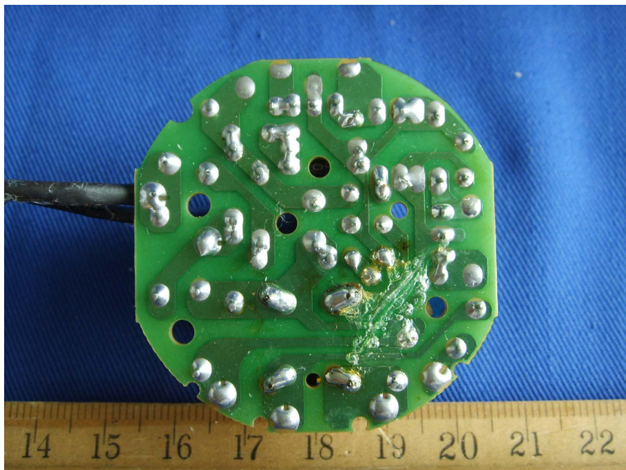
EUT–Solder View (LTEA-24W)
