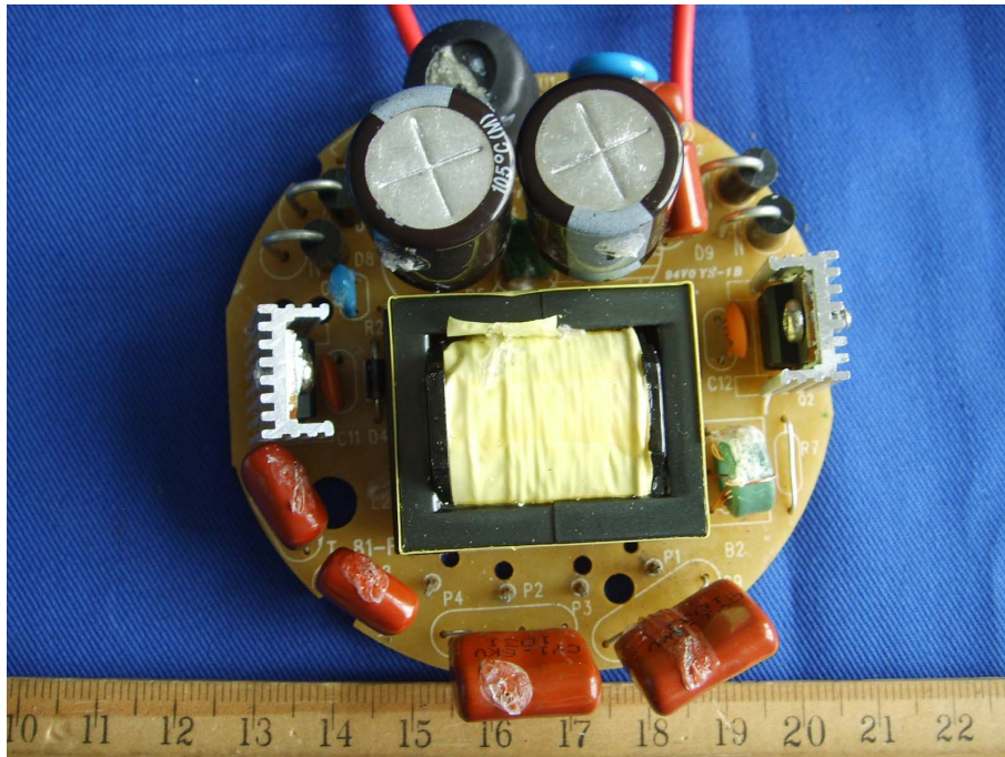
EUT –Components View (LPE-125W)
