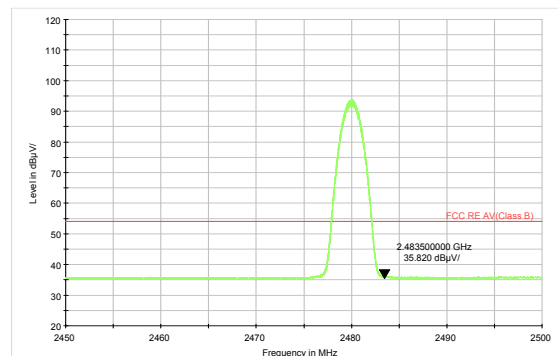
3DH5-Channel 78: Average
