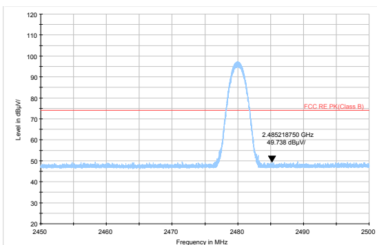
3DH5-Channel 78: Peak
