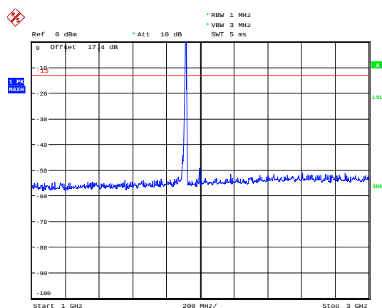
LTE Band 25 3MHz CH-High 1GHz~3GHz
