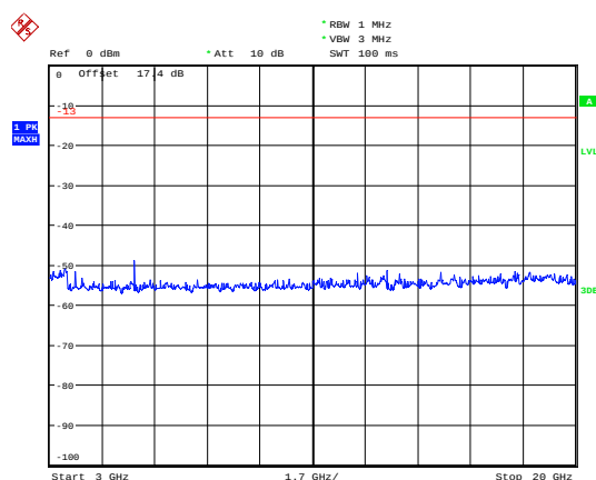
LTE Band 25 3MHz CH-High 3GHz~20GHz
