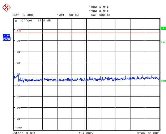
LTE Band 25 3MHz CH-Middle 3GHz~20GHz
