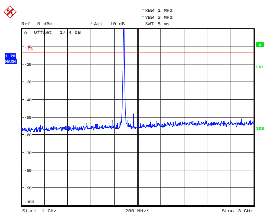
LTE Band 25 3MHz CH-Middle 1GHz~3GHz
