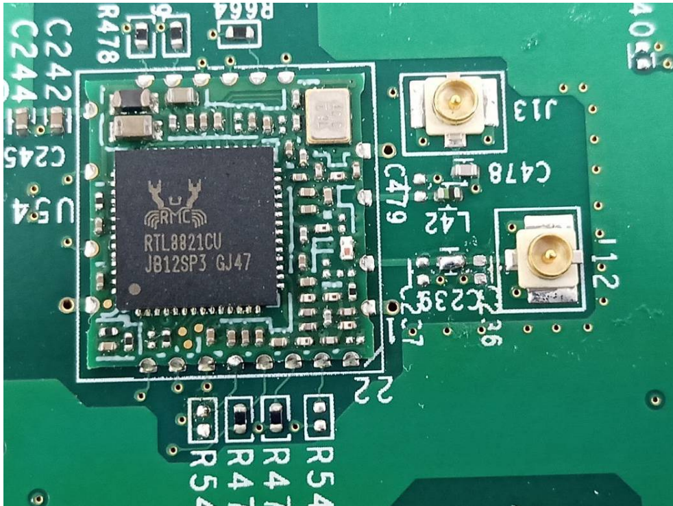
5G Wi-Fi & BT Antenna
