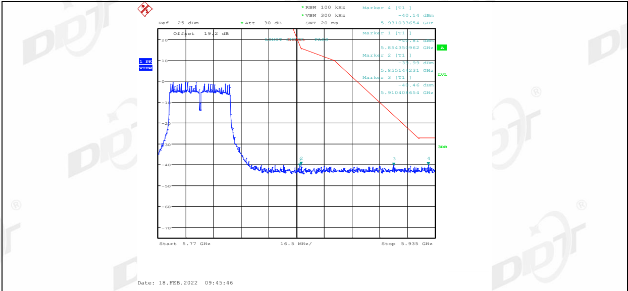
11AC40SISO_Ant1_High_5795
