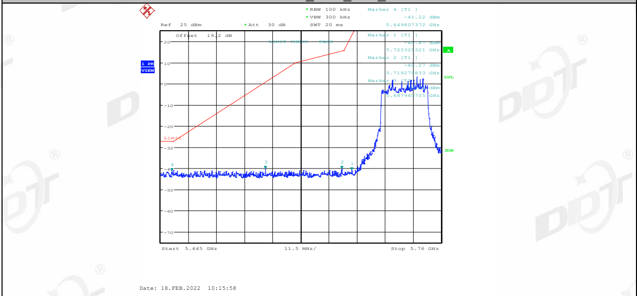
11AX20SISO_Ant1_Low_5745
