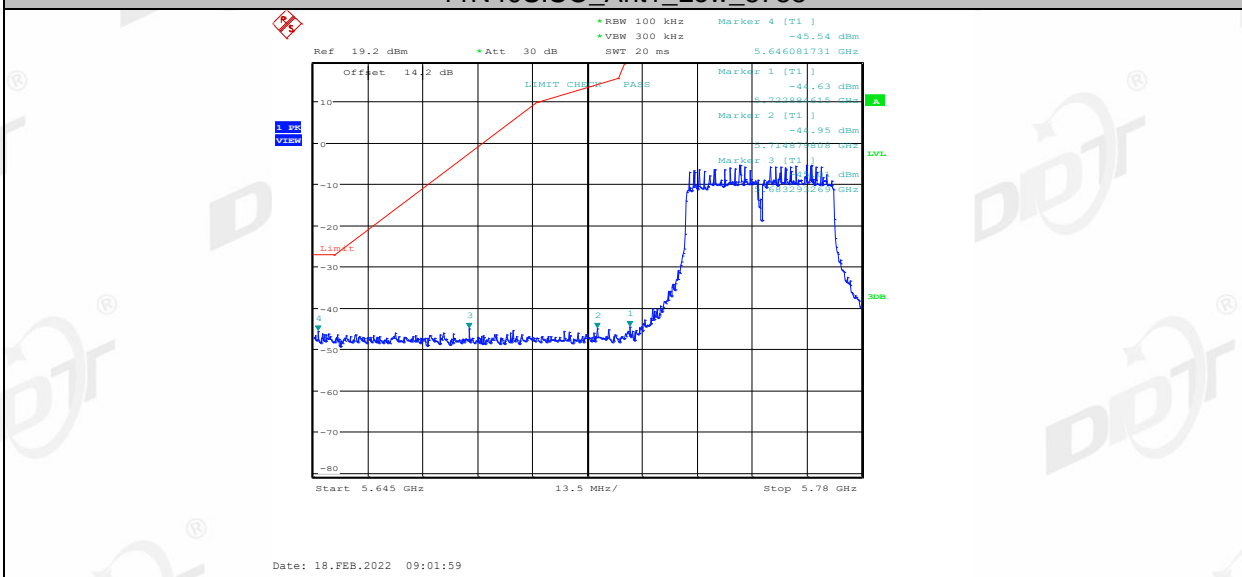
11N40SISO_Ant1_Low_5755
