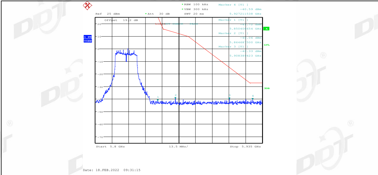
11AC20SISO_Ant1_High_5825
