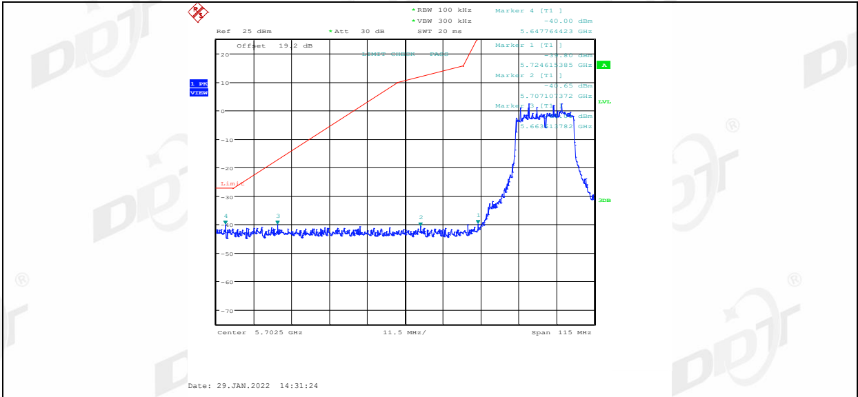
11N20SISO_Ant1_Low_5745
