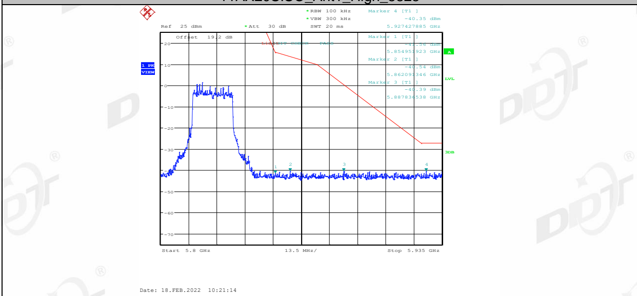
11AX20SISO_Ant1_High_5825
