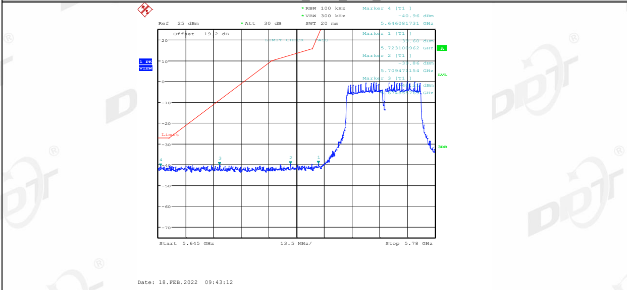
11AC40SISO_Ant1_Low_5755
