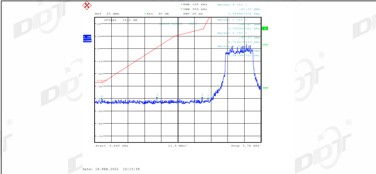
11AX20SISO_Ant1_Low_5745
