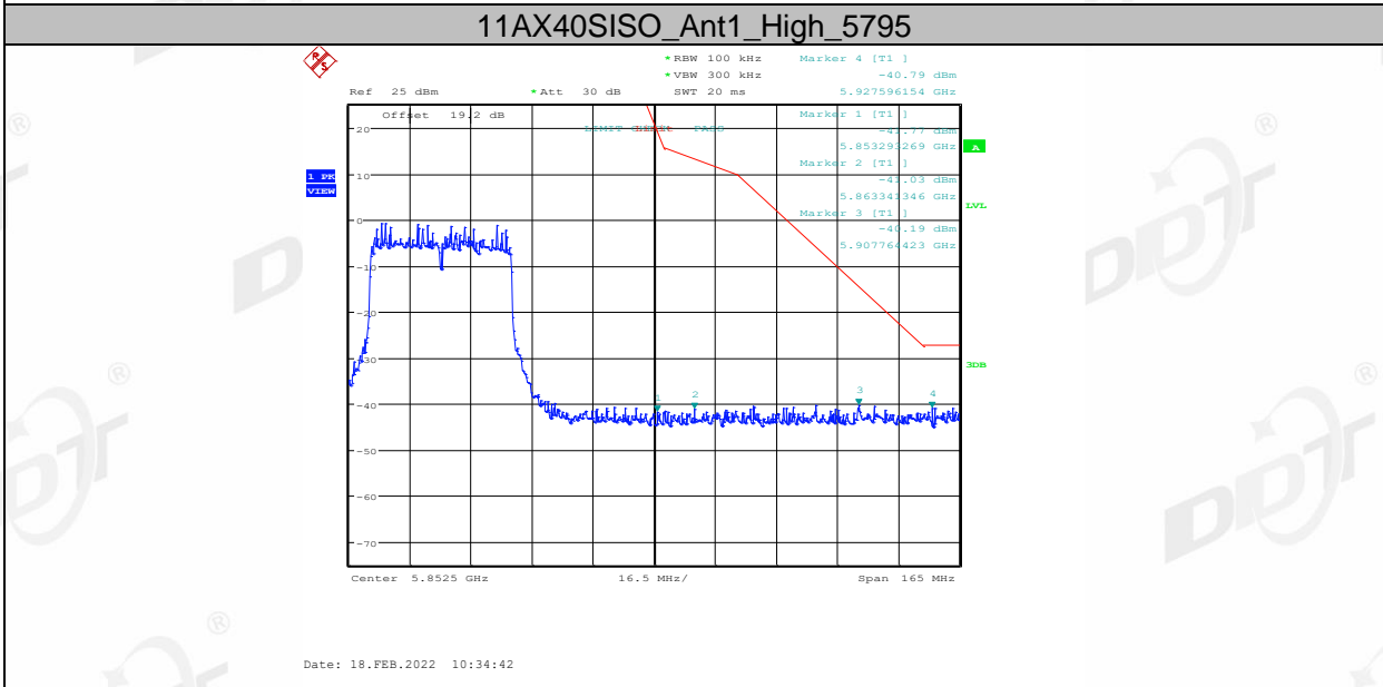
11AX40SISO_Ant1_High_5795
