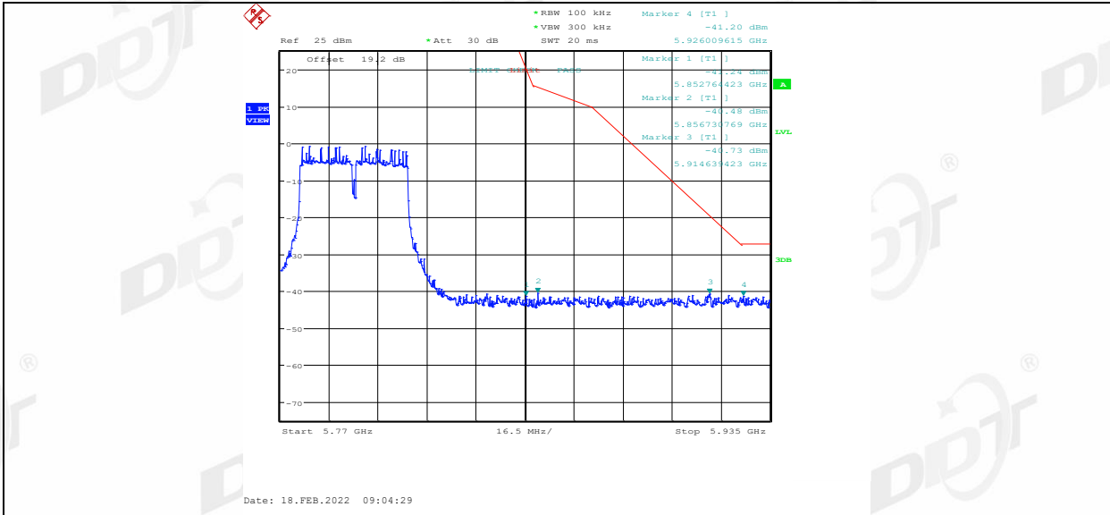
11AC20SISO_Ant1_Low_5745
