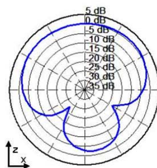
Phi = 0° Plane
