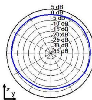
Phi = 90° Plane
