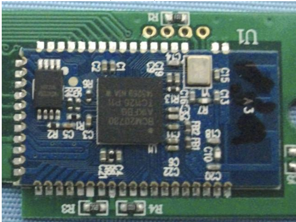
PCB of the EUT-Front View(BT Module)
