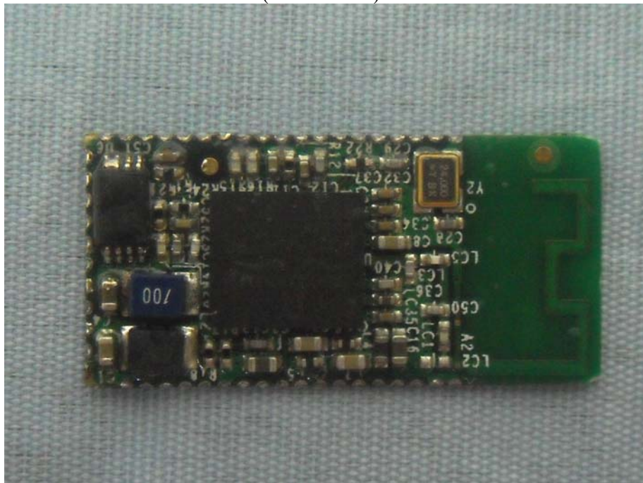
Figure 8 PCB of the EUT-Front View(RF Module)
