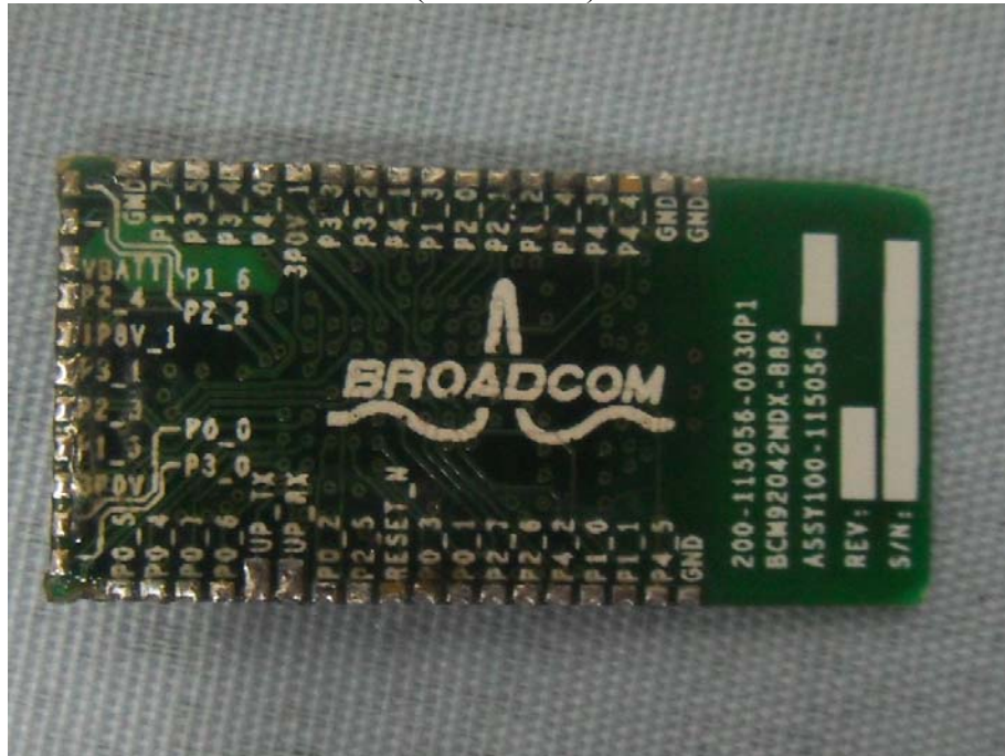
Figure 9 PCB of the EUT-Back View(RF Module)
