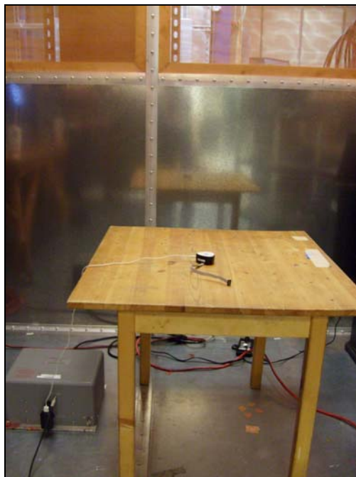
Photograph 2. Conducted Emissions, Test Setup with AC Adaptor
