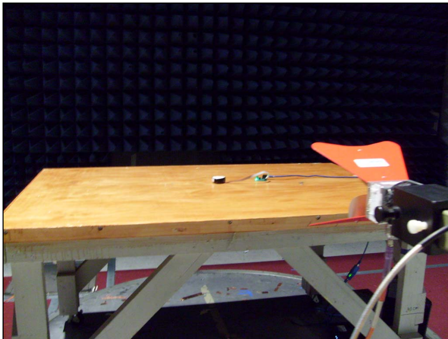
Photograph 6. Restricted Band, Test Setup, 1m
