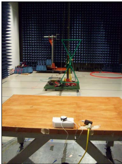
Photograph 4. Radiated Emission, Test Setup with AC Adaptor
