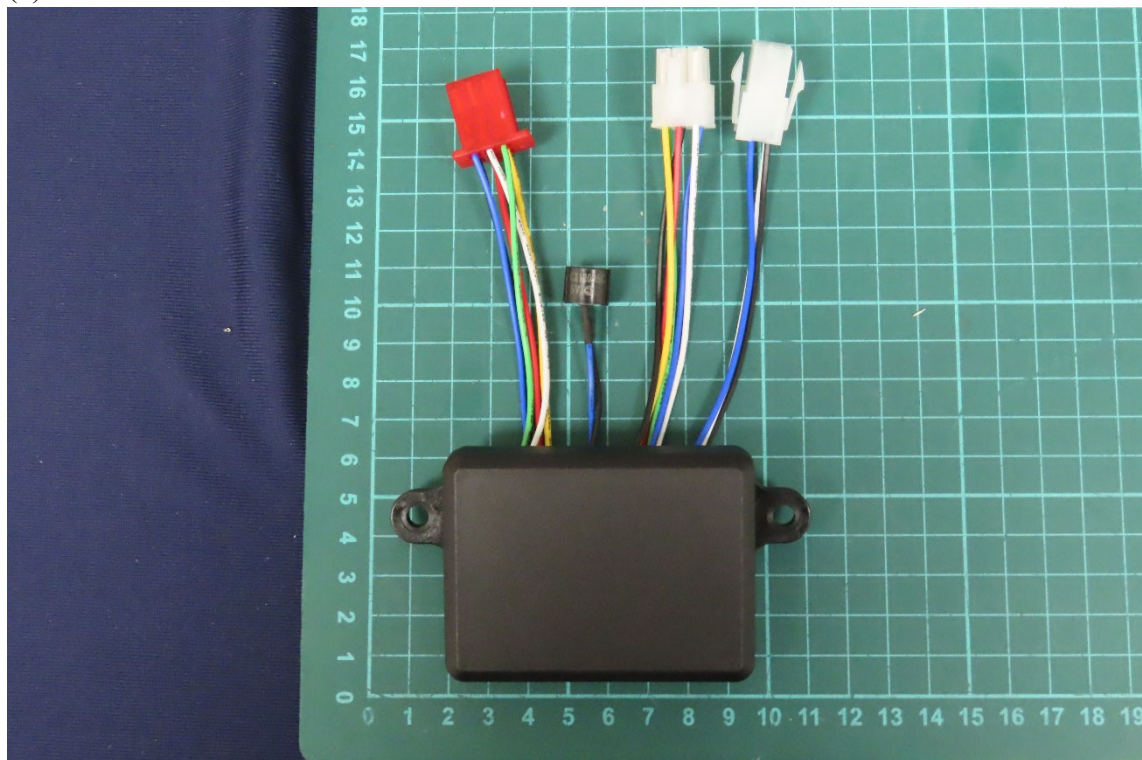
(1) EUT Photo
