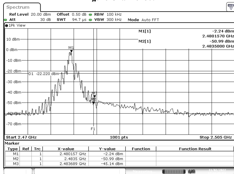
Figure Channel 80:
