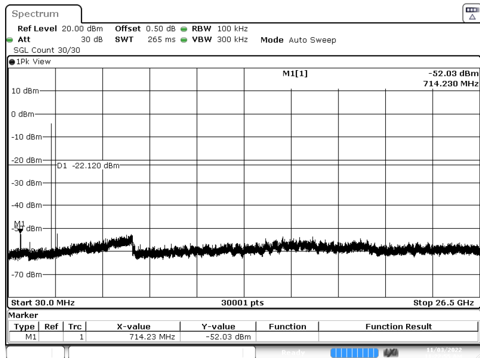
Figure Channel 41:
