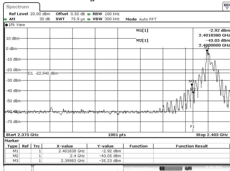
Figure Channel 02:
