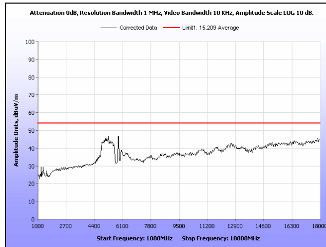
Plot 106. Radiated Spurious Emissions, High Channel, 10 MHz, 1 GHz – 18 GHz, 23 dBi Antenna, Average
