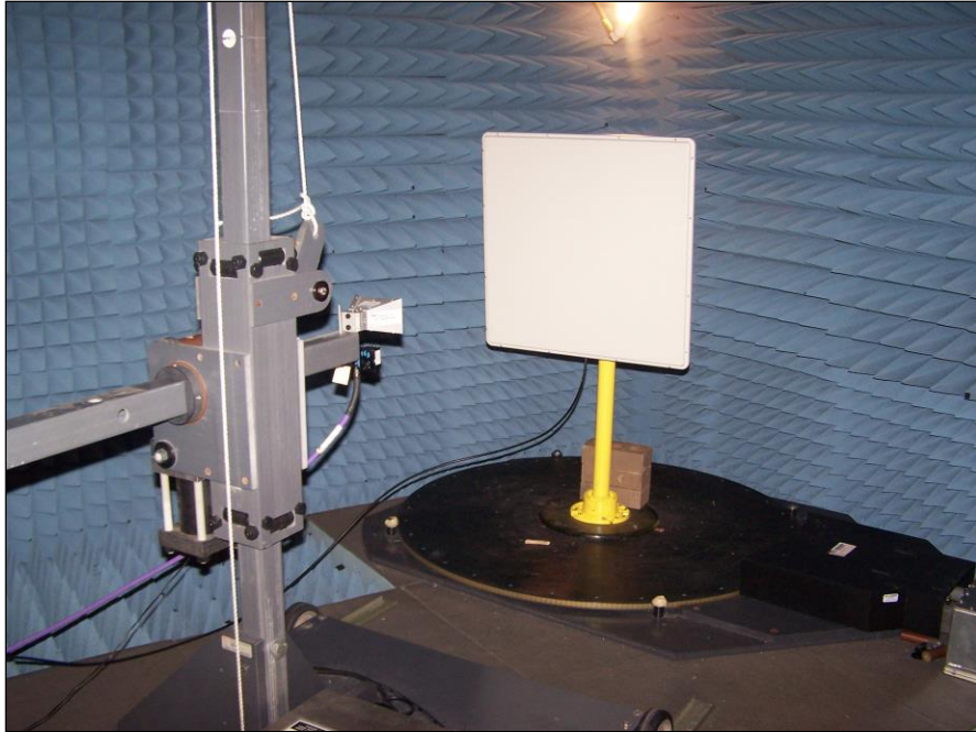
Photograph 6. Radiated Spurious Emissions, Test Setup, 18 GHz – 40 GHz
