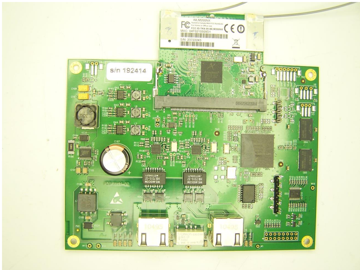
Photograph 5. Front_Full EUT Board
