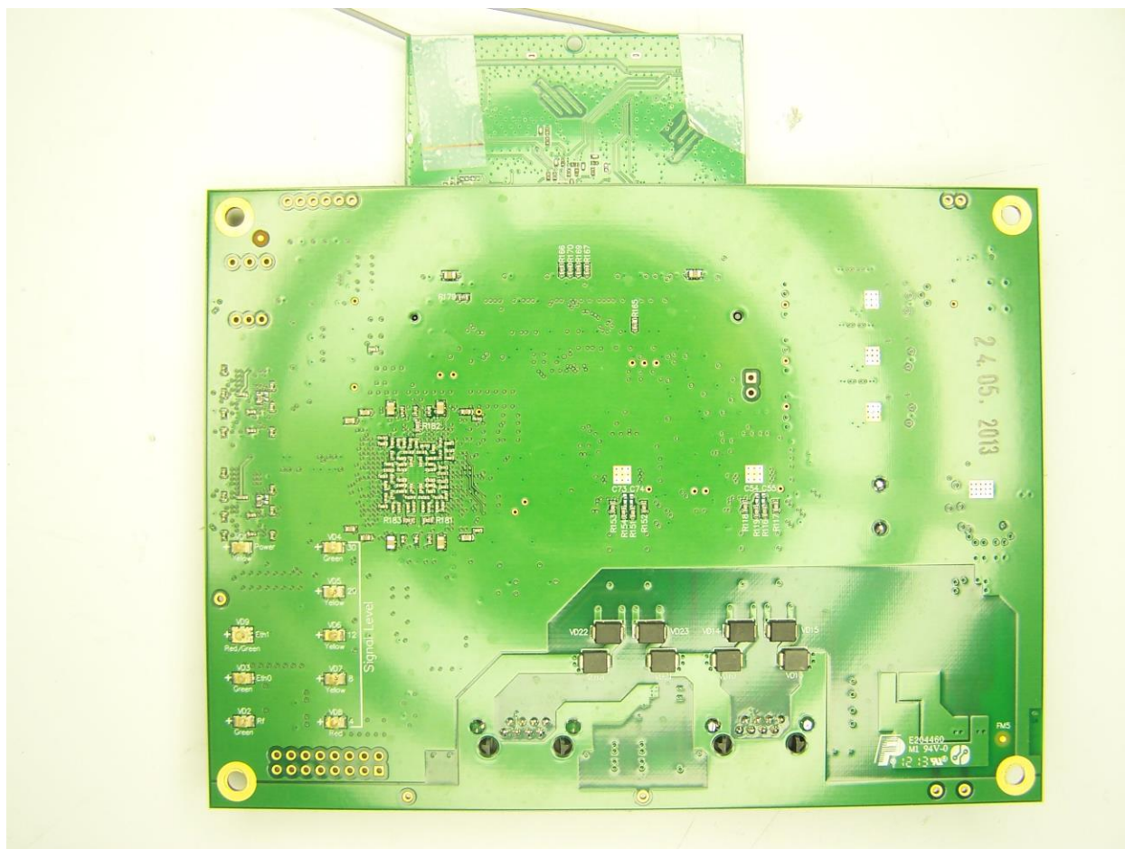
Photograph 1. Back_Full EUT Board
