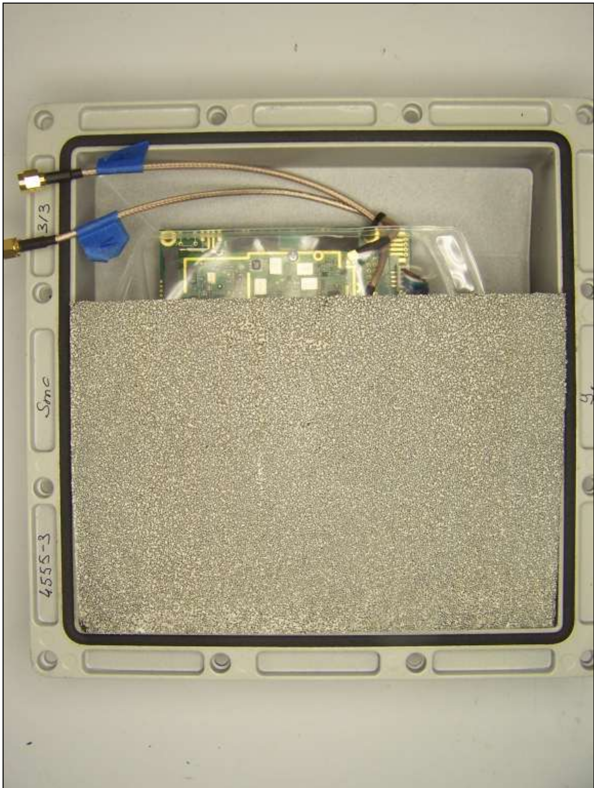
Photograph 6. Smc2x22 interior with absorber
