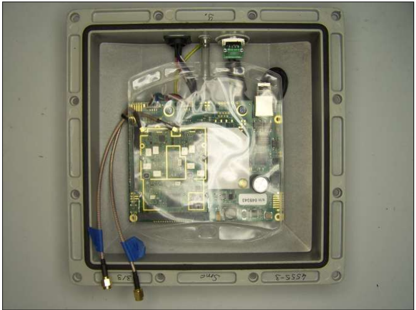
Photograph 7. Smc2x22 interior without absorber
