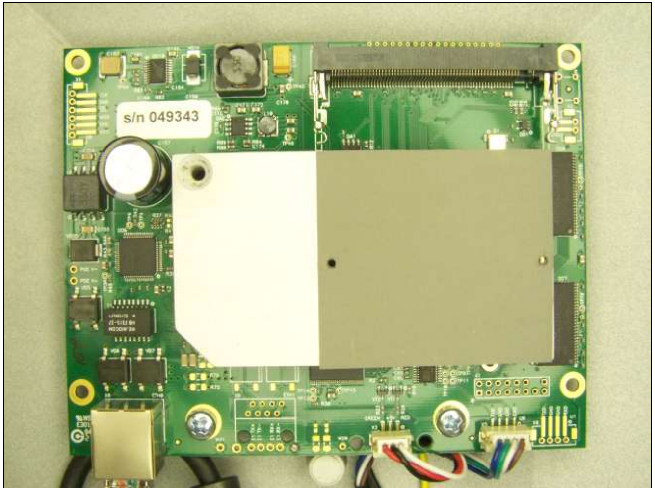
Photograph 4. Smc2x22 board with radio removed
