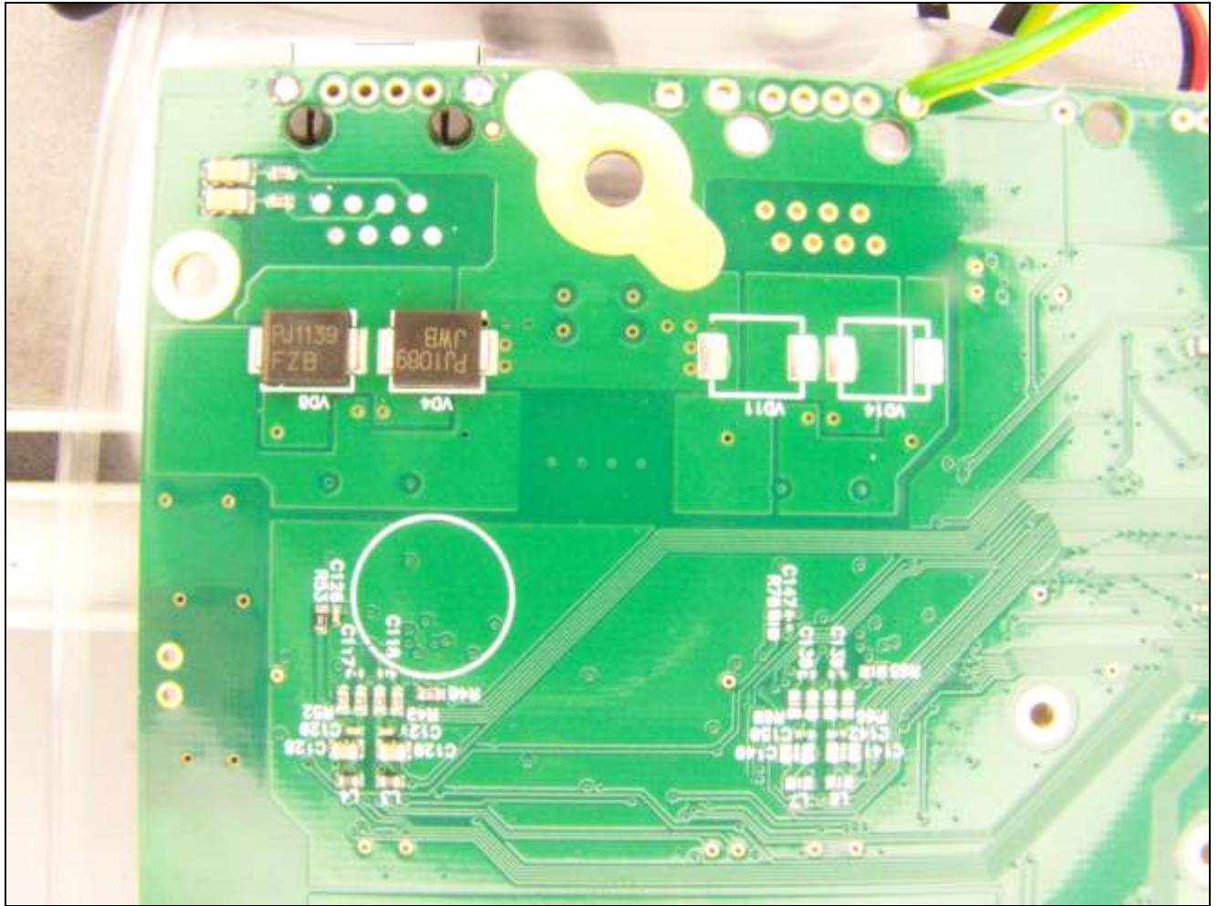
Photograph 1. Smc2x22 board reverse closeup
