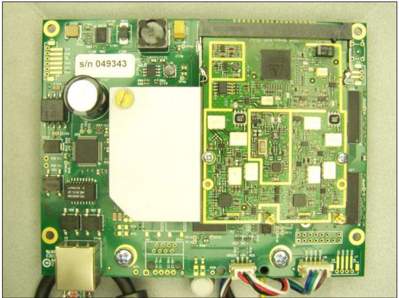
Photograph 5. Smc2x22 entire board
