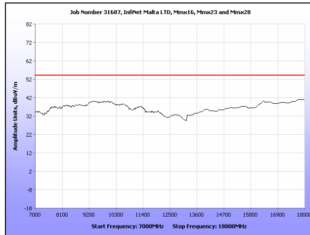
Plot 65. Radiated Spurious Emissions, Mid Channel, 7 GHz – 18 GHz, 40 MHz
