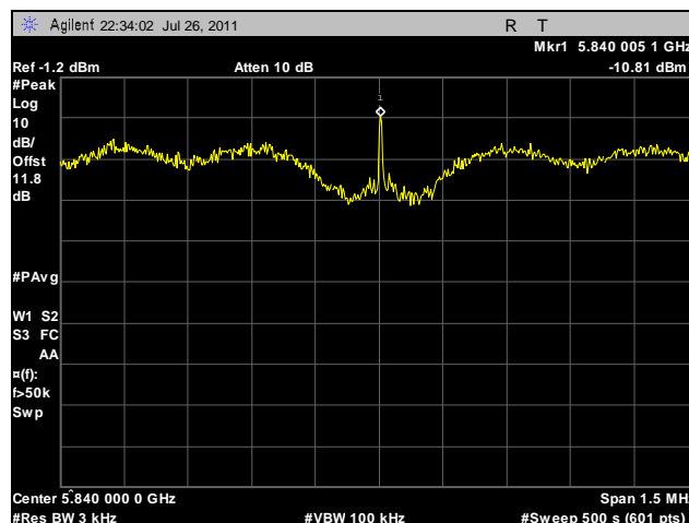
Plot 122. Peak Power Spectral Density, High Channel, 20 MHz, Horizontal Feed
