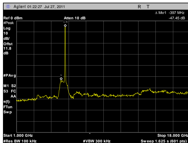
Plot 101. Conducted Spurious Emissions, Low Channel, 1 GHz – 18 GHz, 40 MHz, Vertical Feed
