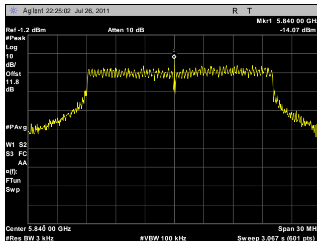
Plot 121. Peak Power Spectral Density, High Channel, 20 MHz, Horizontal Feed, Determination
