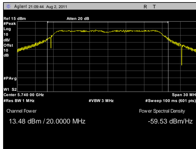
Plot 34. Peak Power Output, Low Channel, 20 MHz, Vertical Feed
