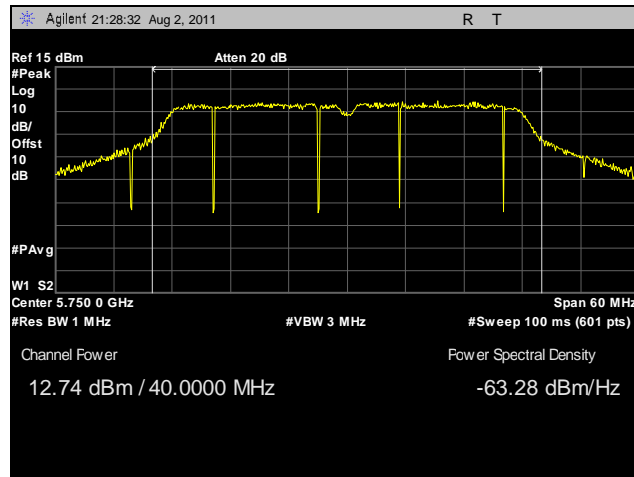
Plot 40. Peak Power Output, Low Channel, 40 MHz, Vertical Feed
