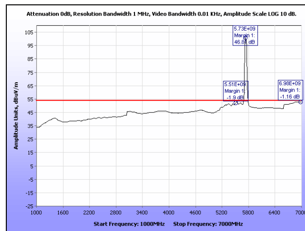
Plot 59. Radiated Spurious Emissions, Low Channel, 1 GHz – 7 GHz, 40 MHz
