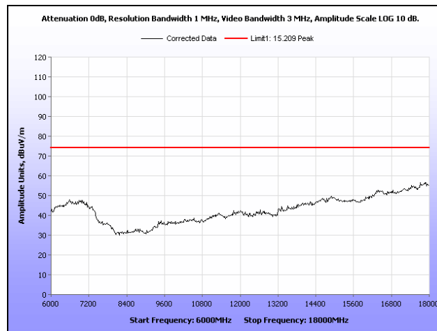
Plot 47. Radiated Spurious Emissions, Low Channel, 6 GHz – 18 GHz, Peak, 20 MHz
