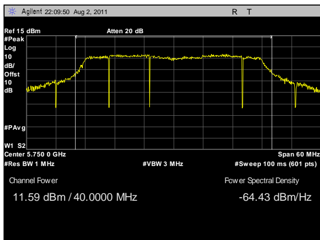
Plot 37. Peak Power Output, Low Channel, 40 MHz, Horizontal Feed
