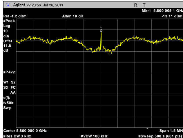
Plot 120. Peak Power Spectral Density, Mid Channel, 20 MHz, Horizontal Feed
