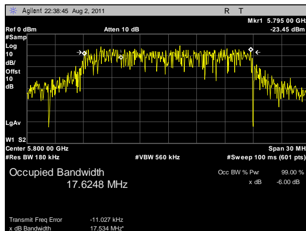
Plot 20. 99% Occupied Bandwidth, Mid Channel, 20 MHz, Horizontal Feed
