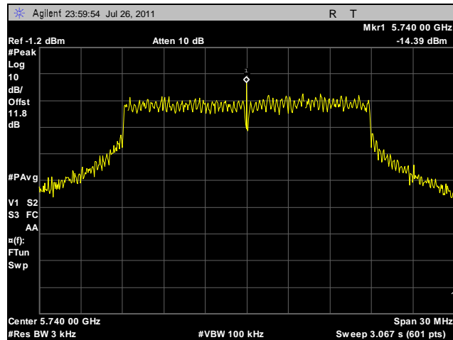
Plot 123. Peak Power Spectral Density, Low Channel, 20 MHz, Vertical Feed, Determination
