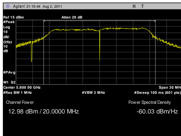
Plot 35. Peak Power Output, Mid Channel, 20 MHz, Vertical Feed
