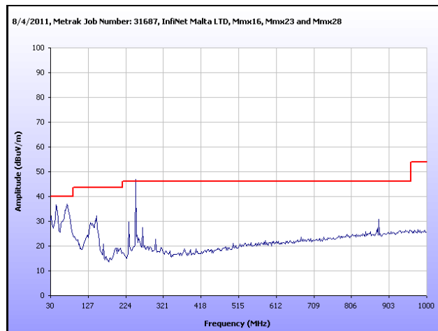
Plot 48. Radiated Spurious Emissions, Mid Channel, 30 MHz – 1 GHz, 20 MHz
