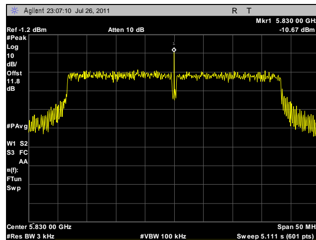
Plot 133. Peak Power Spectral Density, High Channel, 40 MHz, Horizontal Feed, Determination
