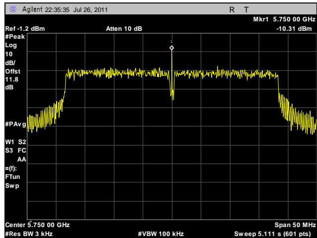
Plot 129. Peak Power Spectral Density, Low Channel, 40 MHz, Horizontal Feed, Determination
