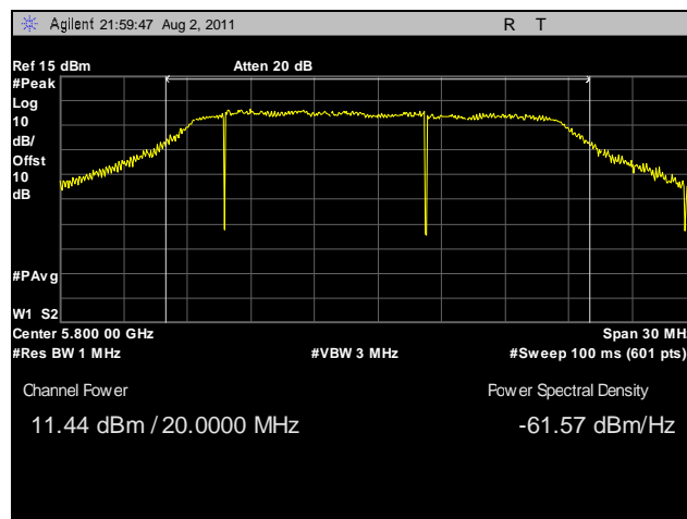
Plot 32. Peak Power Output, Mid Channel, 20 MHz, Horizontal Feed
