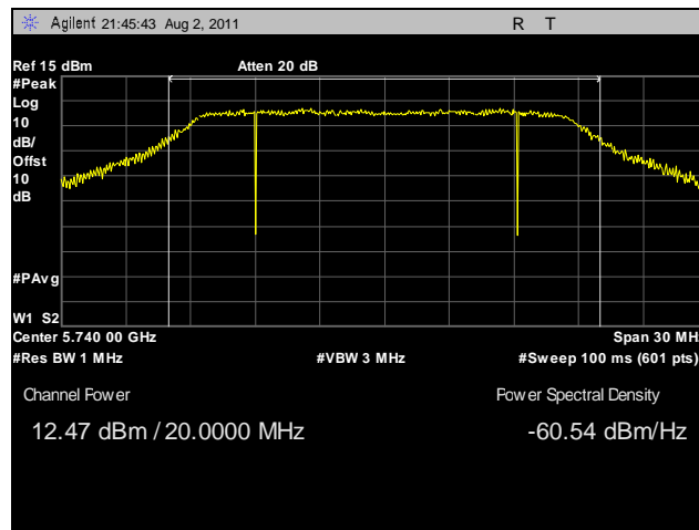
Plot 31. Peak Power Output, Low Channel, 20 MHz, Horizontal Feed
