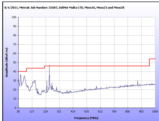
Plot 63. Radiated Spurious Emissions, Mid Channel, 30 MHz – 1 GHz, 40 MHz
