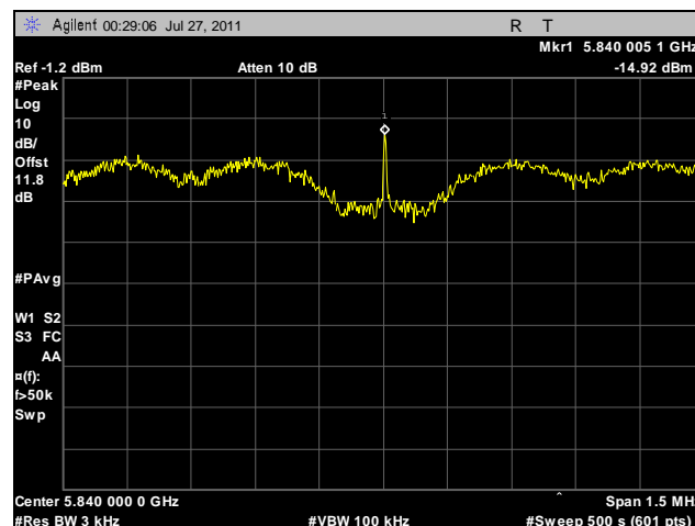
Plot 128. Peak Power Spectral Density, High Channel, 20 MHz, Vertical Feed
