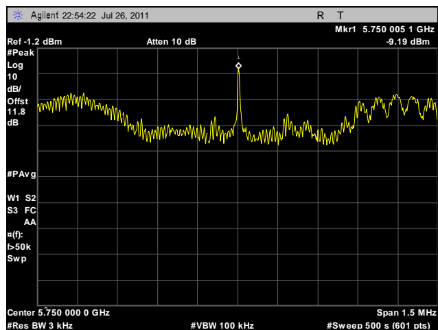
Plot 130. Peak Power Spectral Density, Low Channel, 40 MHz, Horizontal Feed
