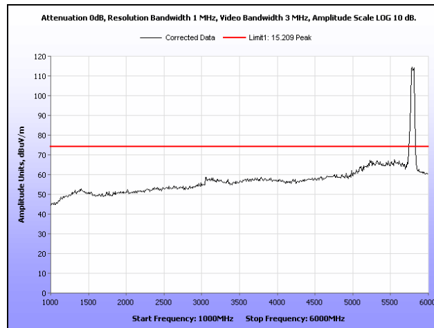
Plot 66. Radiated Spurious Emissions, Mid Channel, 1 GHz – 6 GHz, Peak, 40 MHz
