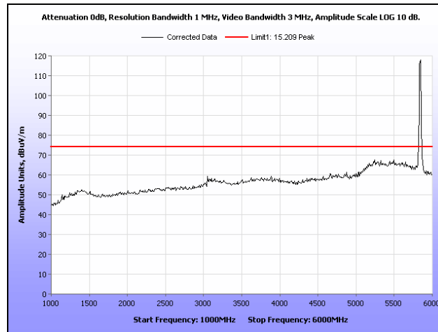
Plot 56. Radiated Spurious Emissions, High Channel, 1 GHz – 6 GHz, Peak, 20 MHz
