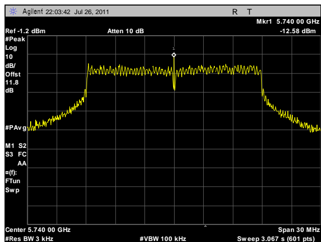
Plot 117. Peak Power Spectral Density, Low Channel, 20 MHz, Horizontal Feed, Determination
