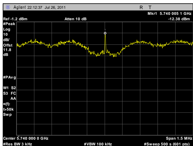
Plot 118. Peak Power Spectral Density, Low Channel, 20 MHz, Horizontal Feed
