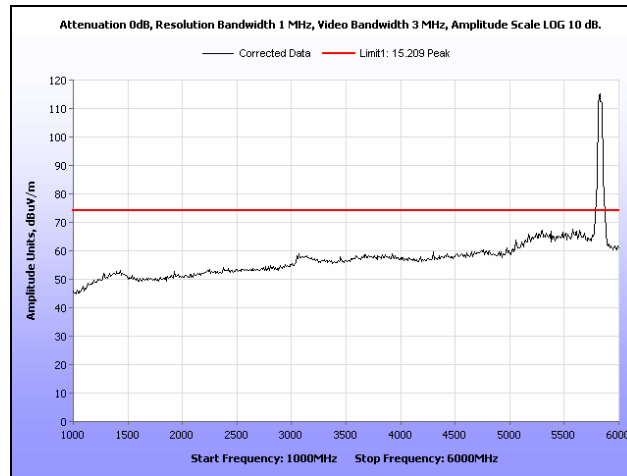
Plot 71. Radiated Spurious Emissions, High Channel, 1 GHz – 6 GHz, Peak, 40 MHz
