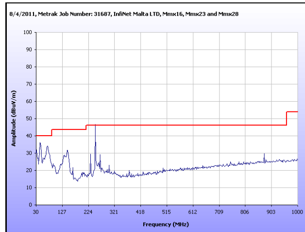
Plot 58. Radiated Spurious Emissions, Low Channel, 30 MHz – 1 GHz, 40 MHz
