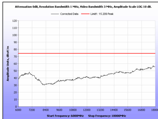
Plot 72. Radiated Spurious Emissions, High Channel, 6 GHz – 18 GHz, Peak, 40 MHz
