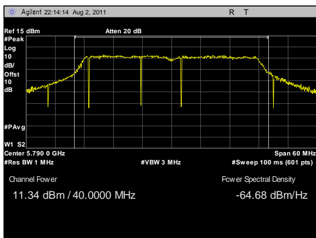
Plot 38. Peak Power Output, Mid Channel, 40 MHz, Horizontal Feed
