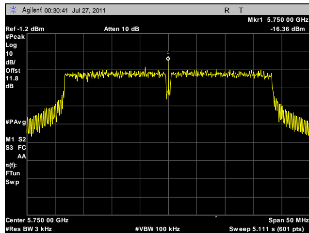
Plot 135. Peak Power Spectral Density, Low Channel, 40 MHz, Vertical Feed, Determination
