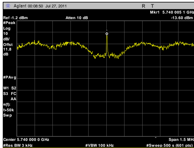
Plot 124. Peak Power Spectral Density, Low Channel, 20 MHz, Vertical Feed
