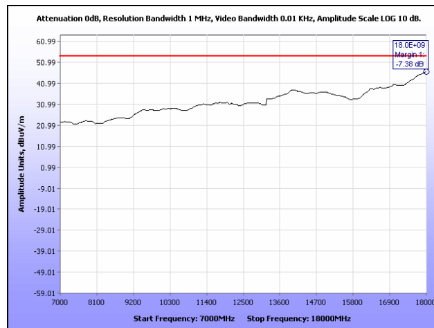
Plot 45. Radiated Spurious Emissions, Low Channel, 7 GHz – 18 GHz, 20 MHz
