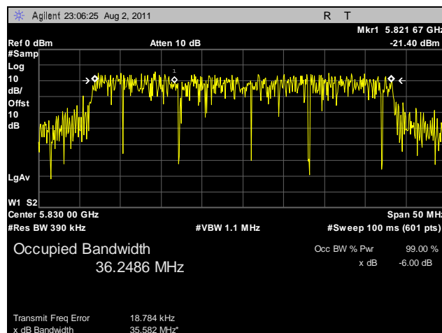
Plot 27. 99% Occupied Bandwidth, High Channel, 40 MHz, Horizontal Feed
