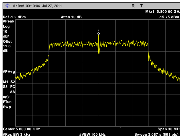
Plot 125. Peak Power Spectral Density, Mid Channel, 20 MHz, Vertical Feed, Determination
