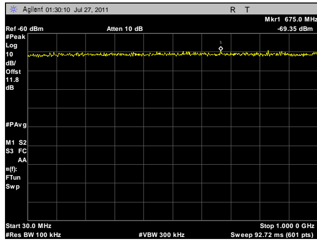
Plot 73. Conducted Spurious Emissions, Low Channel, 30 MHz – 1 GHz, 20 MHz, Horizontal Feed
