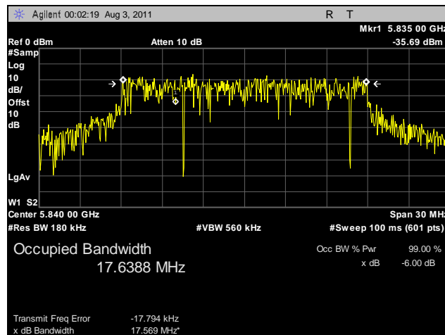
Plot 24. 99% Occupied Bandwidth, High Channel, 20 MHz, Vertical Feed
