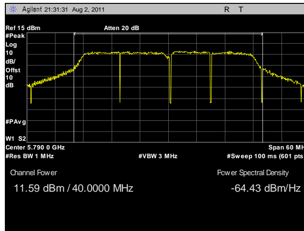
Plot 41. Peak Power Output, Mid Channel, 40 MHz, Vertical Feed
