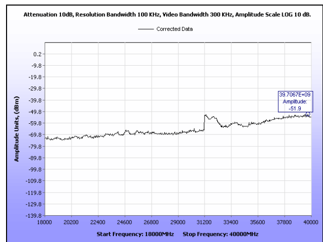
Plot 87. Conducted Spurious Emissions, Mid Channel, 18 GHz – 40 GHz, 20 MHz, Vertical Feed
