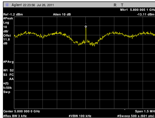
Plot 120. Peak Power Spectral Density, Mid Channel, 20 MHz, Horizontal Feed
