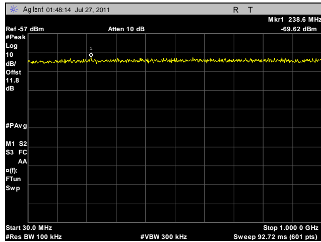
Plot 91. Conducted Spurious Emissions, Low Channel, 30 MHz – 1 GHz, 40 MHz, Horizontal Feed
