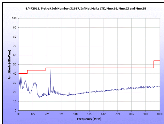
Plot 48. Radiated Spurious Emissions, Mid Channel, 30 MHz – 1 GHz, 20 MHz
