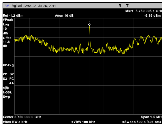
Plot 130. Peak Power Spectral Density, Low Channel, 40 MHz, Horizontal Feed
