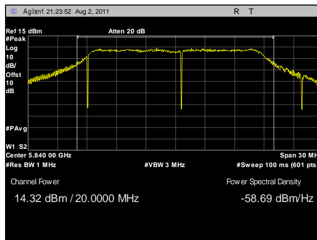
Plot 36. Peak Power Output, High Channel, 20 MHz, Vertical Feed
