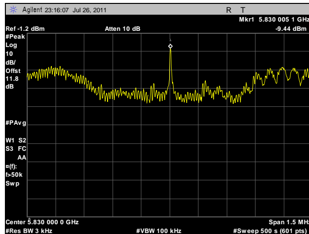
Plot 134. Peak Power Spectral Density, High Channel, 40 MHz, Horizontal Feed
