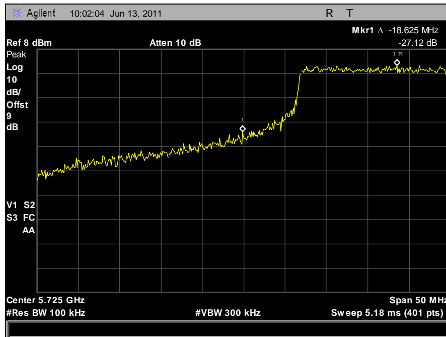
Plot 113. Conducted Band Edge, Low Channel, 40 MHz, Horizontal Feed
