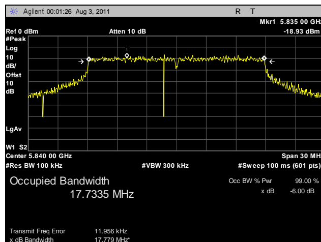
Plot 12. 6 dB Occupied Bandwidth, High Channel, 20 MHz, Vertical Feed
