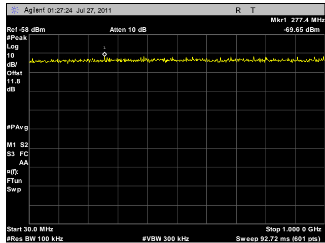
Plot 106. Conducted Spurious Emissions, High Channel, 30 MHz – 1 GHz, 40 MHz, Vertical Feed
