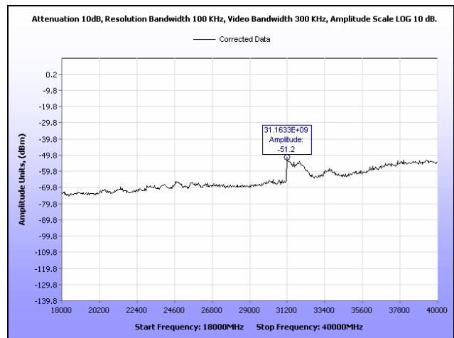
Plot 102. Conducted Spurious Emissions, Low Channel, 18 GHz – 40 GHz, 40 MHz, Vertical Feed
