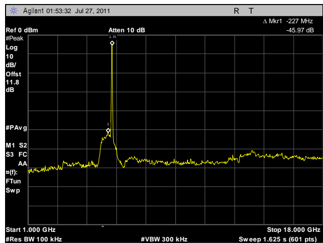
Plot 98. Conducted Spurious Emissions, High Channel, 1 GHz – 18 GHz, 40 MHz, Horizontal Feed
