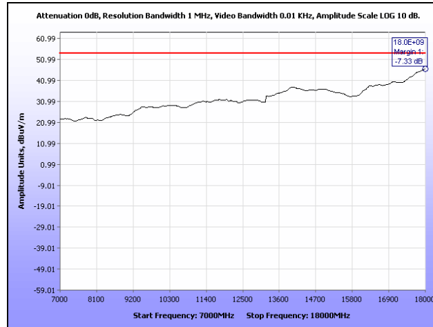
Plot 70. Radiated Spurious Emissions, High Channel, 7 GHz – 18 GHz, 40 MHz
