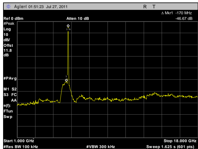
Plot 95. Conducted Spurious Emissions, Mid Channel, 1 GHz – 18 GHz, 40 MHz, Horizontal Feed
