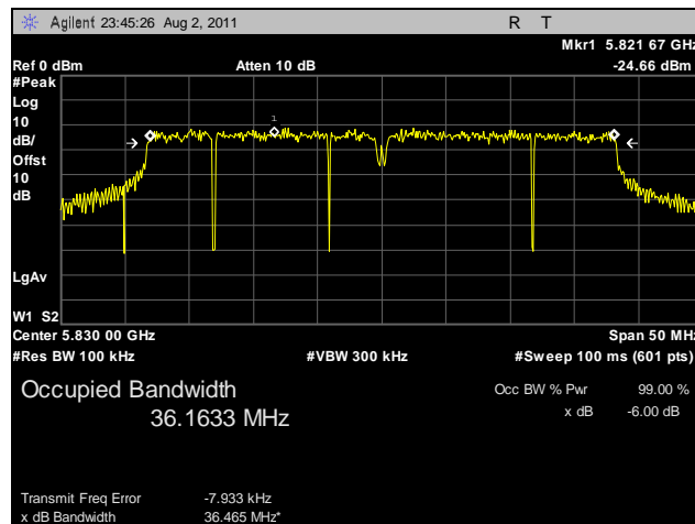
Plot 18. 6 dB Occupied Bandwidth, High Channel, 40 MHz, Vertical Feed
