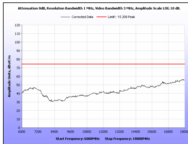
Plot 62. Radiated Spurious Emissions, Low Channel, 6 GHz – 18 GHz, Peak, 40 MHz
