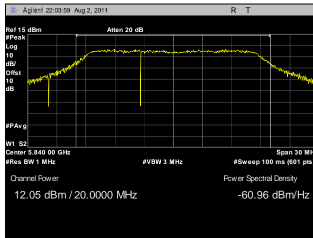
Plot 33. Peak Power Output, High Channel, 20 MHz, Horizontal Feed
