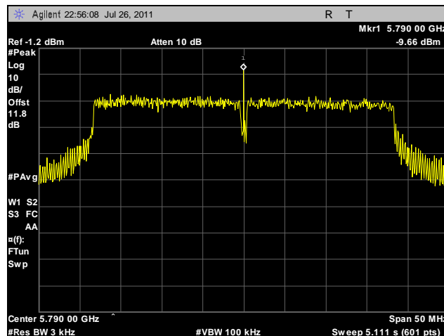
Plot 131. Peak Power Spectral Density, Mid Channel, 40 MHz, Horizontal Feed, Determination
