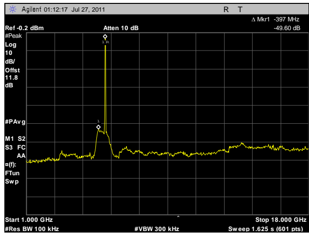
Plot 83. Conducted Spurious Emissions, Low Channel, 1 GHz – 18 GHz, 20 MHz, Vertical Feed
