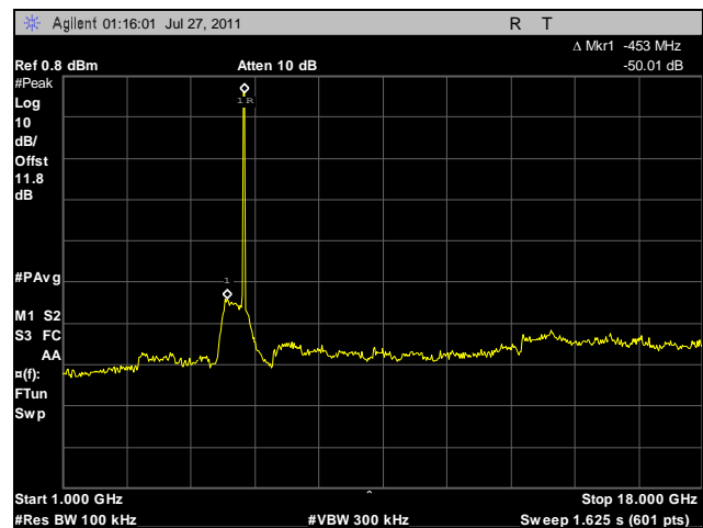
Plot 86. Conducted Spurious Emissions, Mid Channel, 1 GHz – 18 GHz, 20 MHz, Vertical Feed
