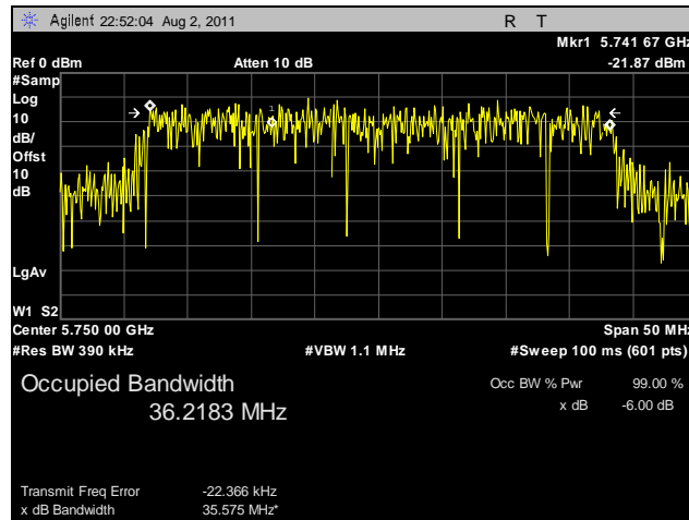
Plot 25. 99% Occupied Bandwidth, Low Channel, 40 MHz, Horizontal Feed
