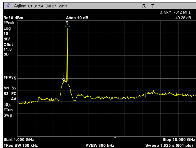
Plot 74. Conducted Spurious Emissions, Low Channel, 1 GHz – 18 GHz, 20 MHz, Horizontal Feed
