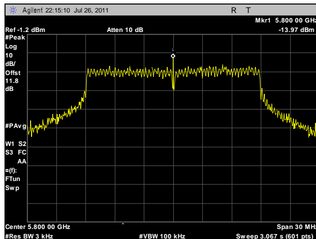
Plot 119. Peak Power Spectral Density, Mid Channel, 20 MHz, Horizontal Feed, Determination
