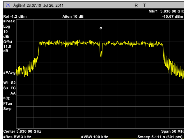
Plot 133. Peak Power Spectral Density, High Channel, 40 MHz, Horizontal Feed, Determination
