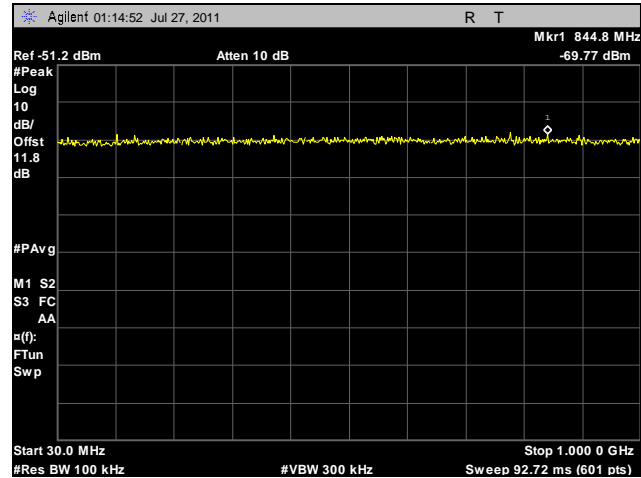
Plot 85. Conducted Spurious Emissions, Mid Channel, 30 MHz – 1 GHz, 20 MHz, Vertical Feed
