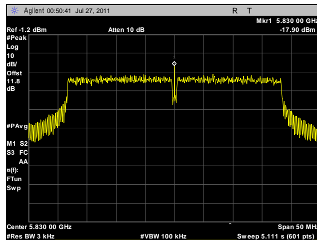
Plot 139. Peak Power Spectral Density, High Channel, 40 MHz, Vertical Feed, Determination
