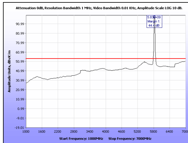
Plot 69. Radiated Spurious Emissions, High Channel, 1 GHz – 7 GHz, 40 MHz
