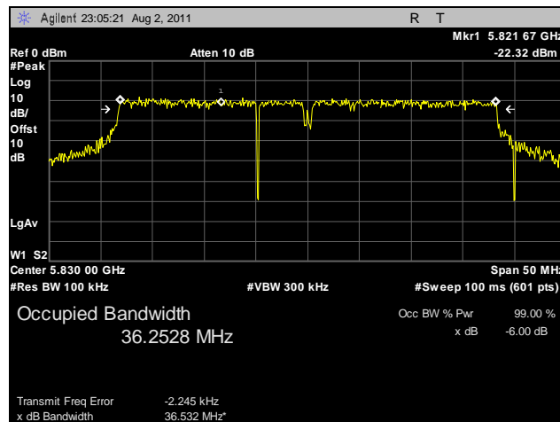
Plot 15. 6 dB Occupied Bandwidth, High Channel, 40 MHz, Horizontal Feed
