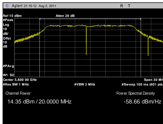
Plot 35. Peak Power Output, Mid Channel, 20 MHz, Vertical Feed
