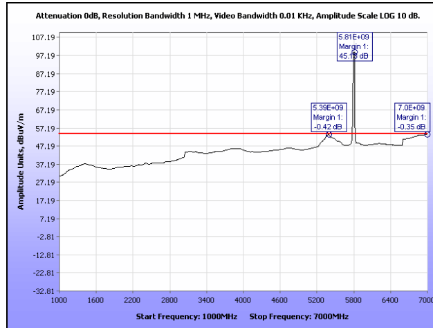
Plot 49. Radiated Spurious Emissions, Mid Channel, 1 GHz – 7 GHz, 20 MHz
