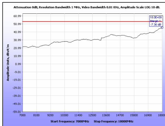
Plot 65. Radiated Spurious Emissions, Mid Channel, 7 GHz – 18 GHz, 40 MHz
