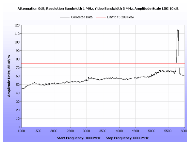
Plot 66. Radiated Spurious Emissions, Mid Channel, 1 GHz – 6 GHz, Peak, 40 MHz
