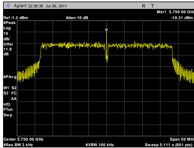
Plot 129. Peak Power Spectral Density, Low Channel, 40 MHz, Horizontal Feed, Determination
