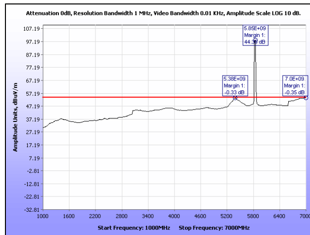
Plot 54. Radiated Spurious Emissions, High Channel, 1 GHz – 7 GHz, 20 MHz
