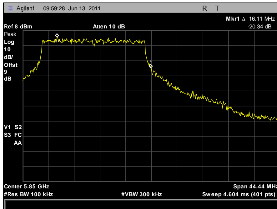
Plot 110. Conducted Band Edge, High Channel, 20 MHz, Horizontal Feed
