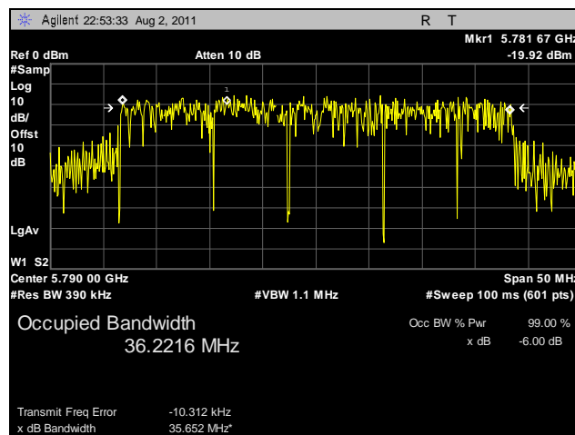
Plot 26. 99% Occupied Bandwidth, Mid Channel, 40 MHz, Horizontal Feed
