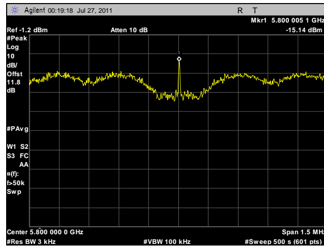
Plot 126. Peak Power Spectral Density, Mid Channel, 20 MHz, Vertical Feed
