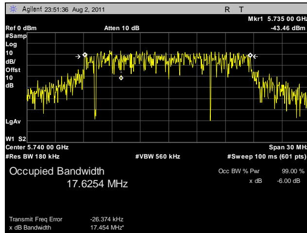
Plot 22. 99% Occupied Bandwidth, Low Channel, 20 MHz, Vertical Feed
