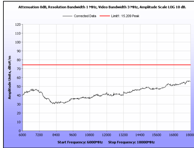
Plot 67. Radiated Spurious Emissions, Mid Channel, 6 GHz – 18 GHz, Peak, 40 MHz
