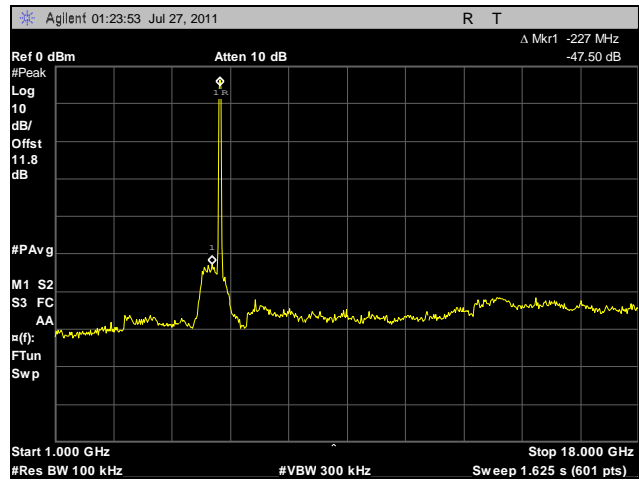
Plot 104. Conducted Spurious Emissions, Mid Channel, 1 GHz – 18 GHz, 40 MHz, Vertical Feed
