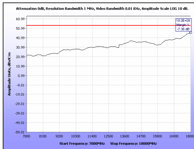
Plot 50. Radiated Spurious Emissions, Mid Channel, 7 GHz – 18 GHz, 20 MHz
