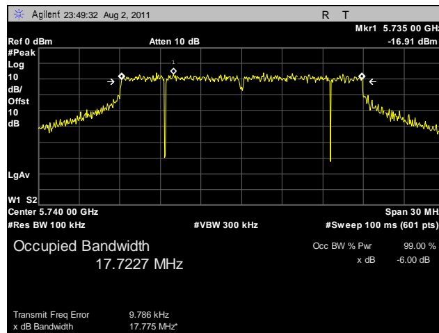
Plot 10. 6 dB Occupied Bandwidth, Low Channel, 20 MHz, Vertical Feed
