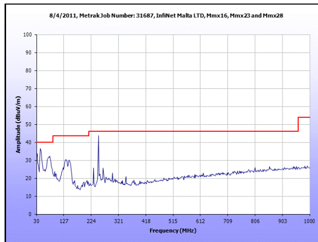
Plot 53. Radiated Spurious Emissions, High Channel, 30 MHz – 1 GHz, 20 MHz
