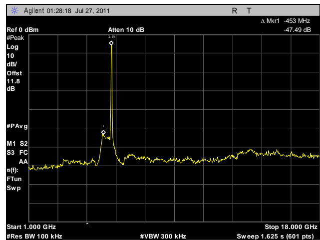
Plot 107. Conducted Spurious Emissions, High Channel, 1 GHz – 18 GHz, 40 MHz, Vertical Feed
