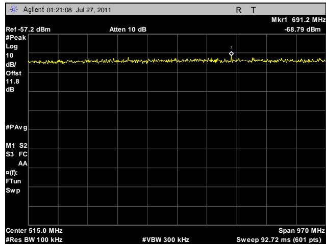
Plot 100. Conducted Spurious Emissions, Low Channel, 30 MHz – 1 GHz, 40 MHz, Vertical Feed
