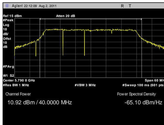
Plot 38. Peak Power Output, Mid Channel, 40 MHz, Horizontal Feed
