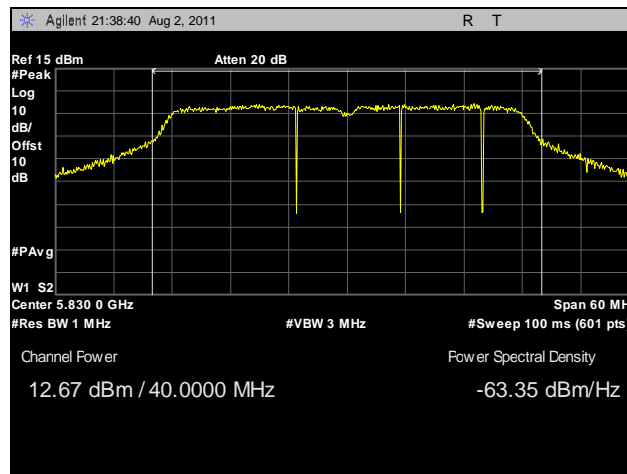
Plot 42. Peak Power Output, High Channel, 40 MHz, Vertical Feed
