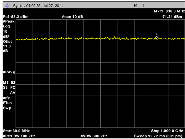
Plot 82. Conducted Spurious Emissions, Low Channel, 30 MHz – 1 GHz, 20 MHz, Vertical Feed
