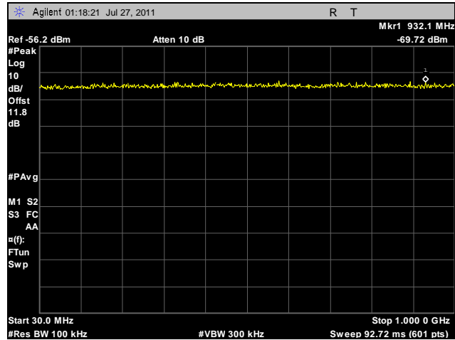
Plot 88. Conducted Spurious Emissions, High Channel, 30 MHz – 1 GHz, 20 MHz, Vertical Feed
