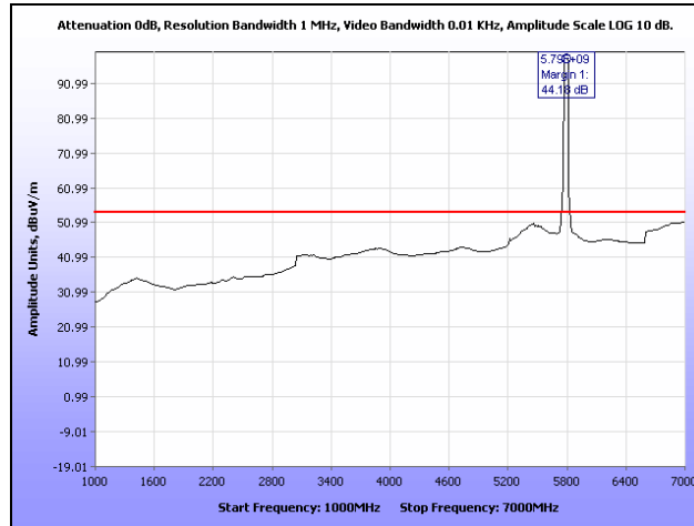
Plot 64. Radiated Spurious Emissions, Mid Channel, 1 GHz – 7 GHz, 40 MHz
