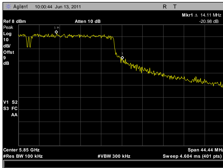
Plot 114. Conducted Band Edge, High Channel, 40 MHz, Horizontal Feed
