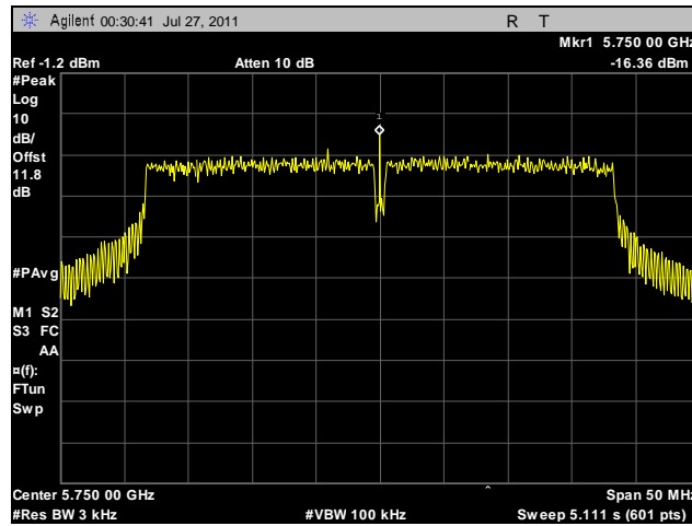
Plot 135. Peak Power Spectral Density, Low Channel, 40 MHz, Vertical Feed, Determination
