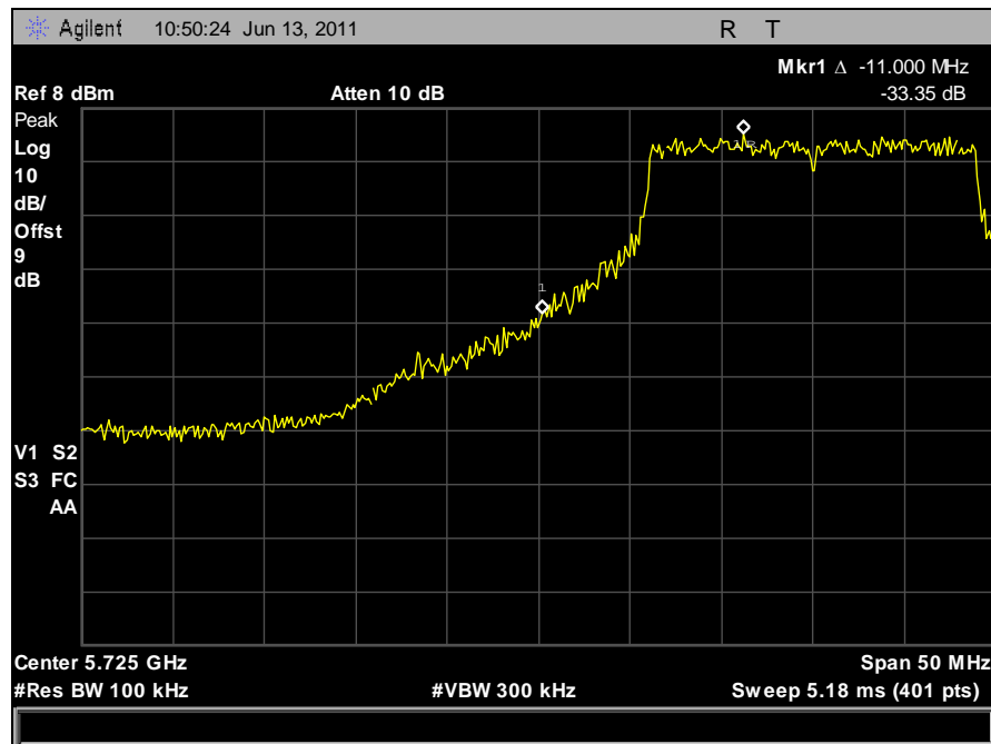
Plot 111. Conducted Band Edge, Low Channel, 20 MHz, Vertical Feed
