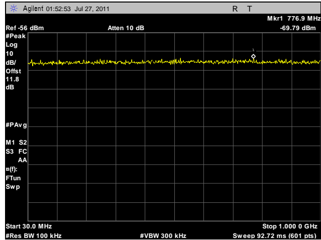
Plot 97. Conducted Spurious Emissions, High Channel, 30 MHz – 1 GHz, 40 MHz, Horizontal Feed
