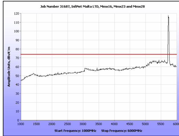
Plot 46. Radiated Spurious Emissions, Low Channel, 1 GHz – 6 GHz, Peak, 20 MHz
