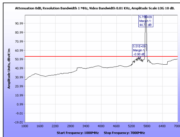
Plot 59. Radiated Spurious Emissions, Low Channel, 1 GHz – 7 GHz, 40 MHz
