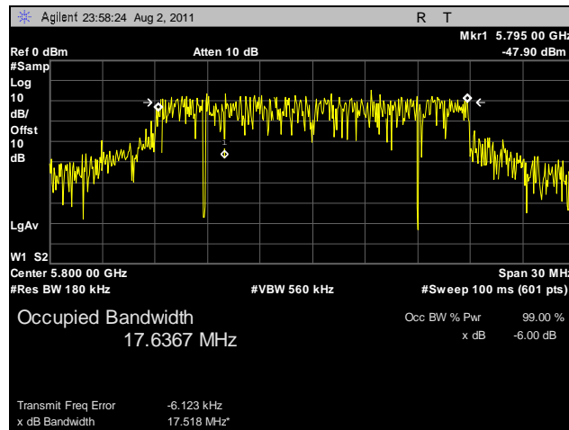
Plot 23. 99% Occupied Bandwidth, Mid Channel, 20 MHz, Vertical Feed
