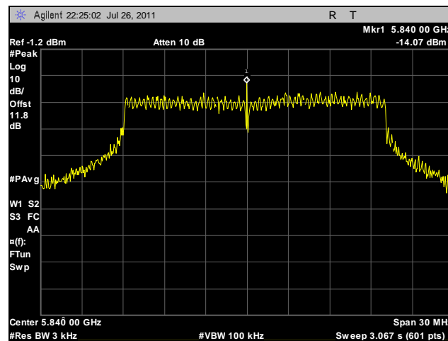
Plot 121. Peak Power Spectral Density, High Channel, 20 MHz, Horizontal Feed, Determination
