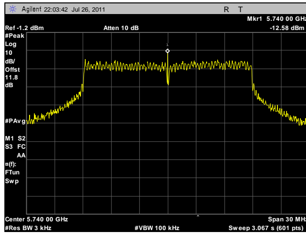
Plot 117. Peak Power Spectral Density, Low Channel, 20 MHz, Horizontal Feed, Determination
