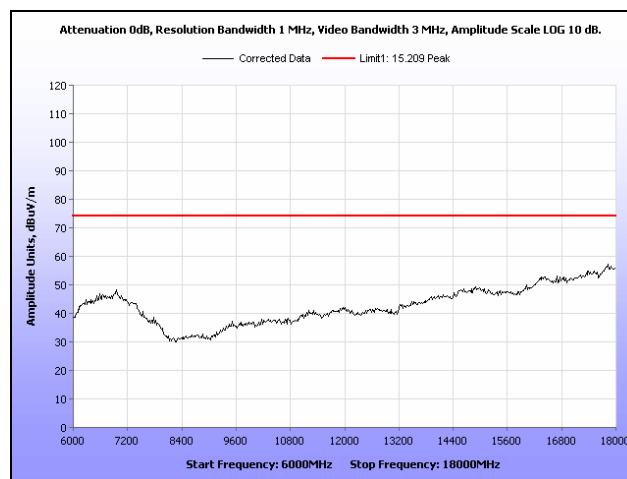
Plot 72. Radiated Spurious Emissions, High Channel, 6 GHz – 18 GHz, Peak, 40 MHz
