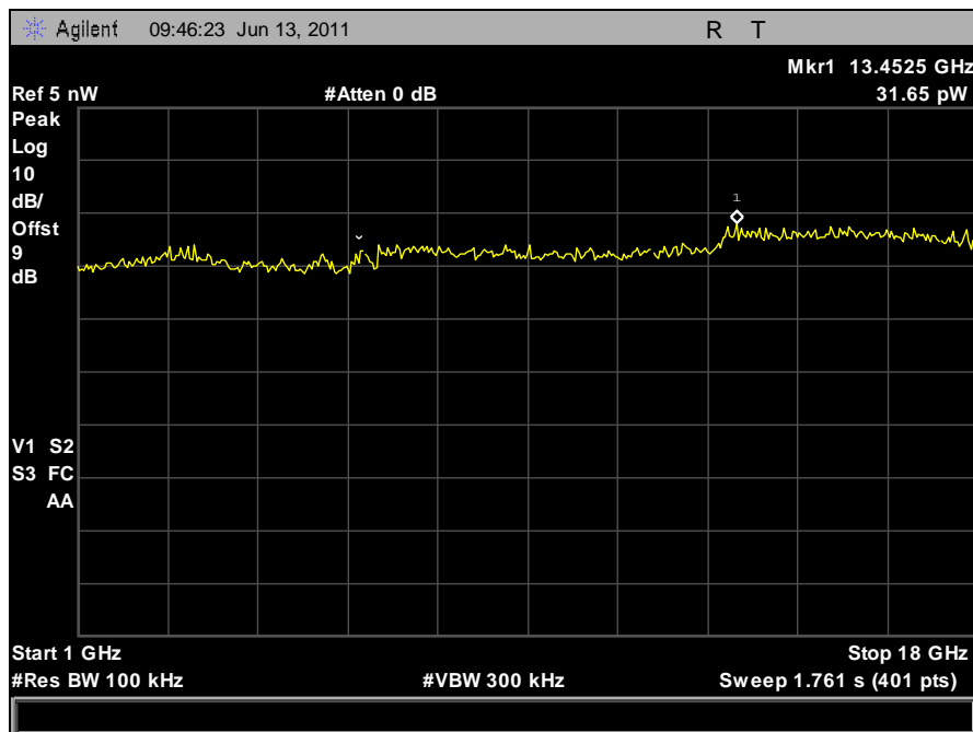
Plot 144. Conducted Receiver Spurious Emissions, Mid Channel, 1 GHz – 18 GHz, Vertical Feed
