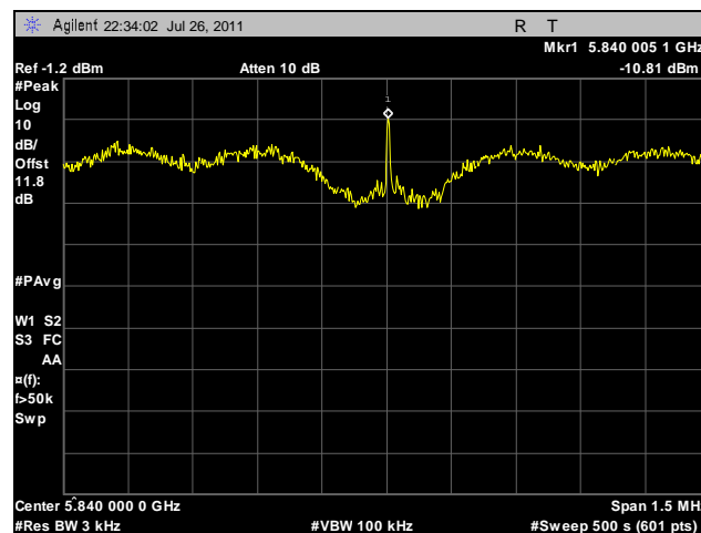
Plot 122. Peak Power Spectral Density, High Channel, 20 MHz, Horizontal Feed
