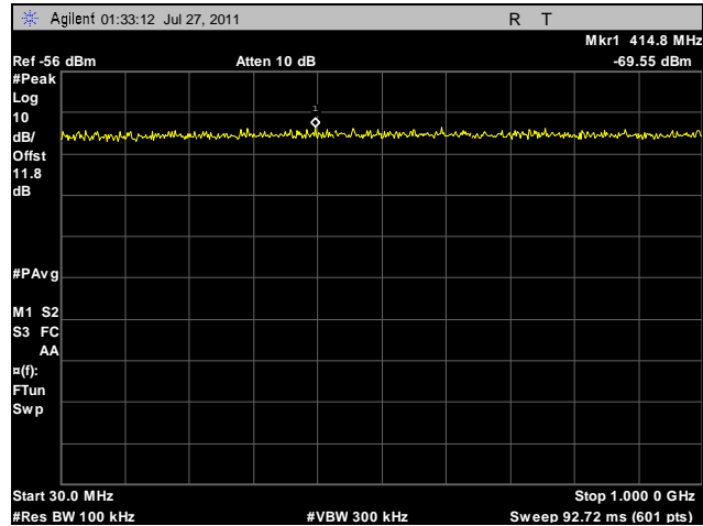
Plot 76. Conducted Spurious Emissions, Mid Channel, 30 MHz – 1 GHz, 20 MHz, Horizontal Feed
