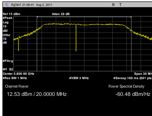
Plot 32. Peak Power Output, Mid Channel, 20 MHz, Horizontal Feed
