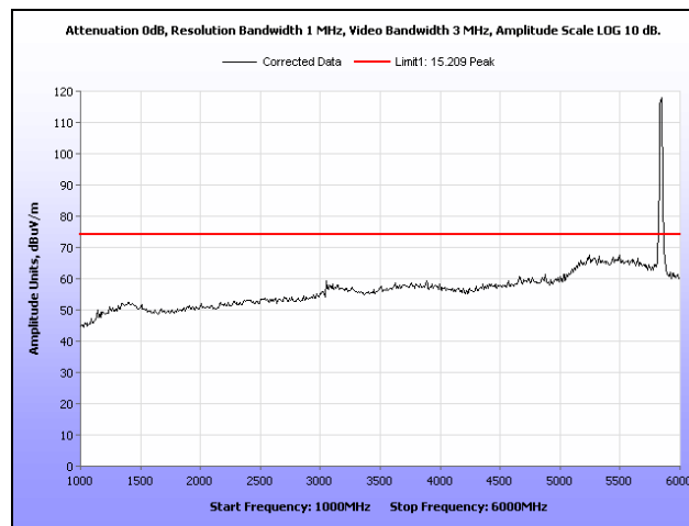
Plot 56. Radiated Spurious Emissions, High Channel, 1 GHz – 6 GHz, Peak, 20 MHz
