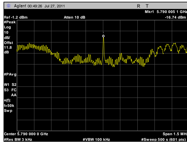
Plot 138. Peak Power Spectral Density, Mid Channel, 40 MHz, Vertical Feed
