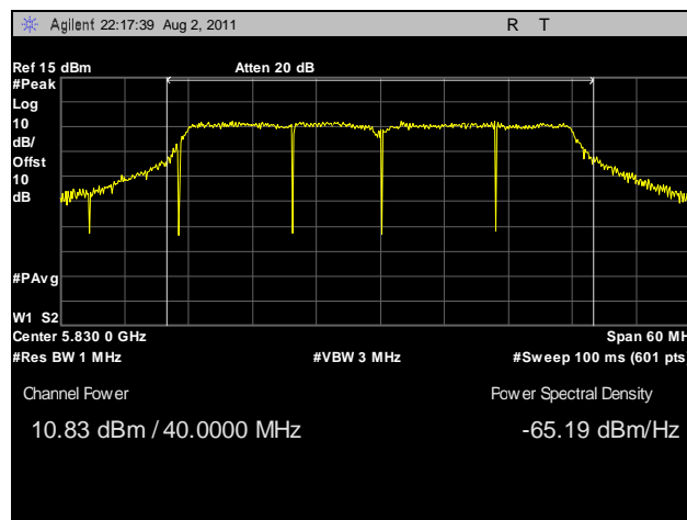
Plot 39. Peak Power Output, High Channel, 40 MHz, Horizontal Feed
