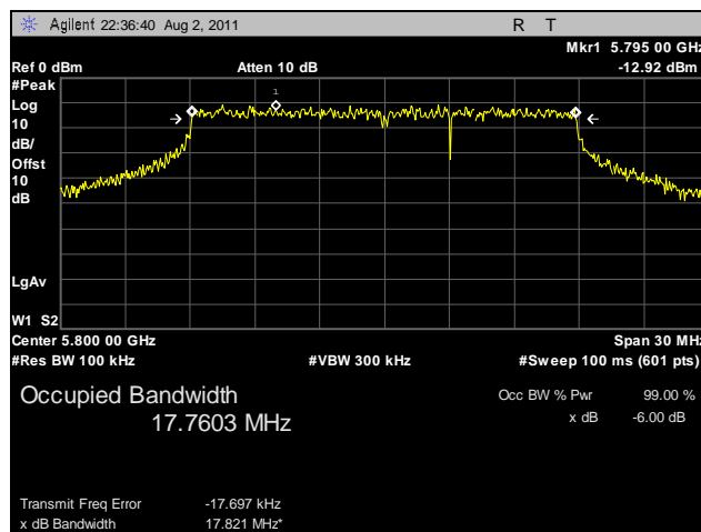
Plot 8. 6 dB Occupied Bandwidth, Mid Channel, 20 MHz, Horizontal Feed
