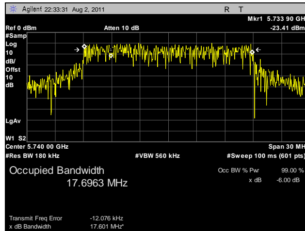
Plot 19. 99% Occupied Bandwidth, Low Channel, 20 MHz, Horizontal Feed
