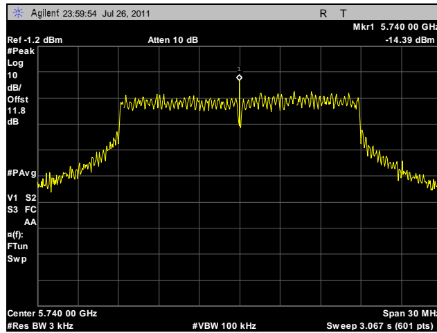
Plot 123. Peak Power Spectral Density, Low Channel, 20 MHz, Vertical Feed, Determination
