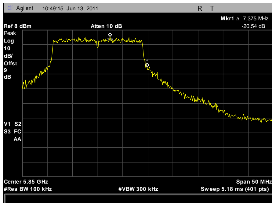
Plot 112. Conducted Band Edge, High Channel, 20 MHz, Vertical Feed
