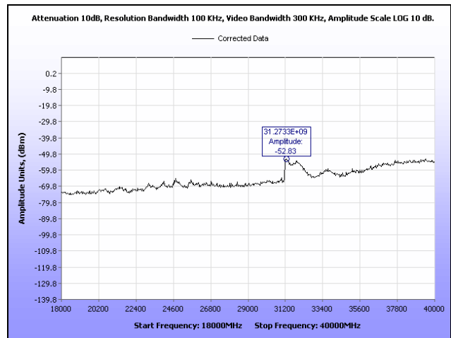
Plot 105. Conducted Spurious Emissions, Mid Channel, 18 GHz – 40 GHz, 40 MHz, Vertical Feed
