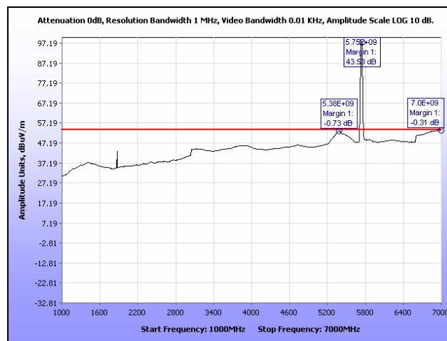
Plot 44. Radiated Spurious Emissions, Low Channel, 1 GHz – 7 GHz, 20 MHz
