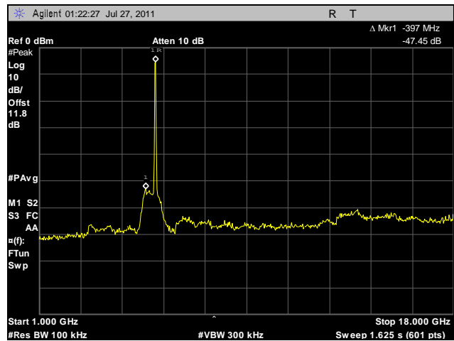
Plot 101. Conducted Spurious Emissions, Low Channel, 1 GHz – 18 GHz, 40 MHz, Vertical Feed
