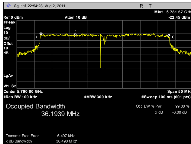
Plot 14. 6 dB Occupied Bandwidth, Mid Channel, 40 MHz, Horizontal Feed
