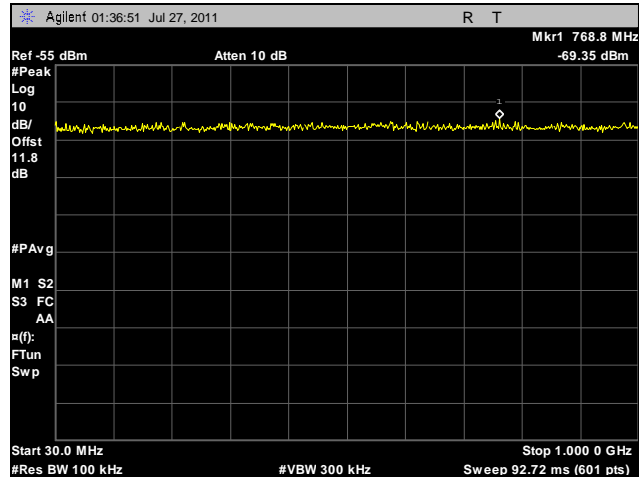
Plot 103. Conducted Spurious Emissions, Mid Channel, 30 MHz – 1 GHz, 40 MHz, Vertical Feed
