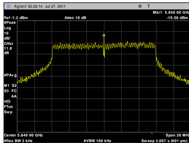
Plot 127. Peak Power Spectral Density, High Channel, 20 MHz, Vertical Feed, Determination
