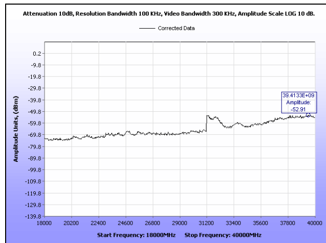
Plot 75. Conducted Spurious Emissions, Low Channel, 18 GHz – 40 GHz, 20 MHz, Horizontal Feed
