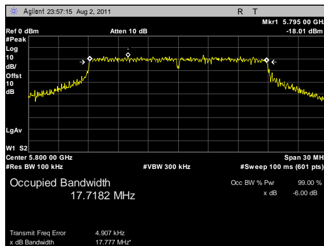
Plot 11. 6 dB Occupied Bandwidth, Mid Channel, 20 MHz, Vertical Feed
