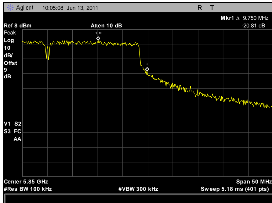
Plot 116. Conducted Band Edge, High Channel, 40 MHz, Vertical Feed
