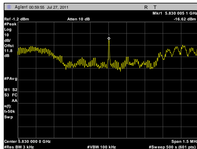
Plot 140. Peak Power Spectral Density, High Channel, 40 MHz, Vertical Feed
