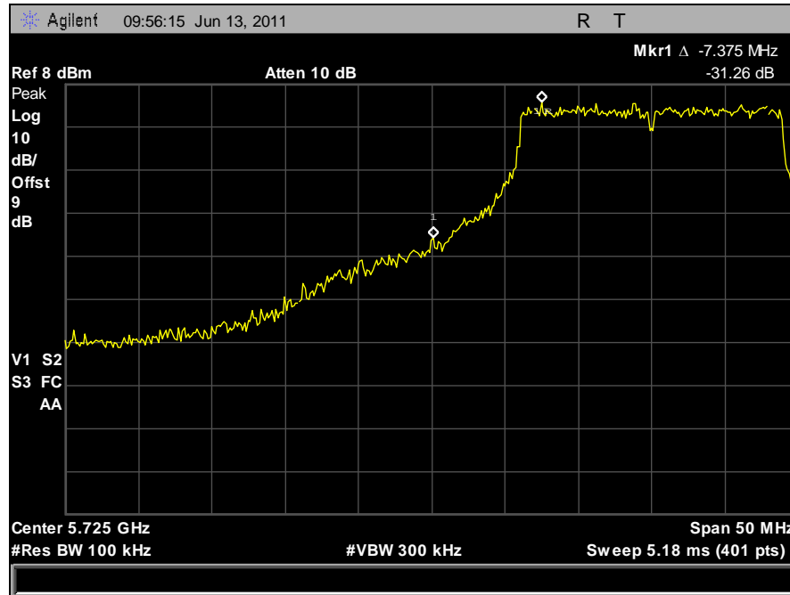
Plot 109. Conducted Band Edge, Low Channel, 20 MHz, Horizontal Feed
