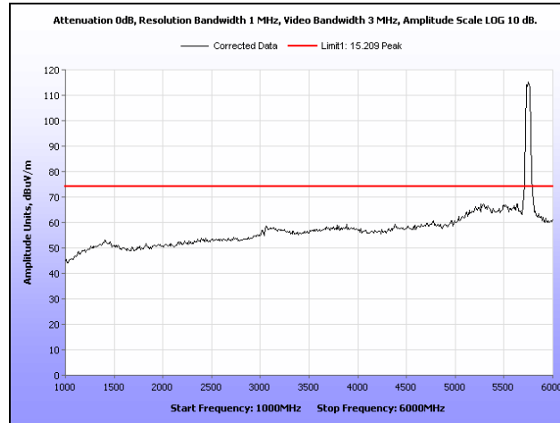
Plot 61. Radiated Spurious Emissions, Low Channel, 1 GHz – 6 GHz, Peak, 40 MHz
