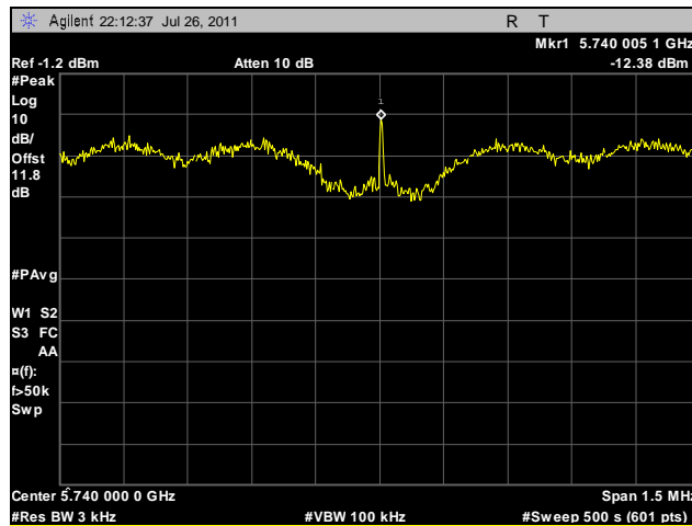
Plot 118. Peak Power Spectral Density, Low Channel, 20 MHz, Horizontal Feed
