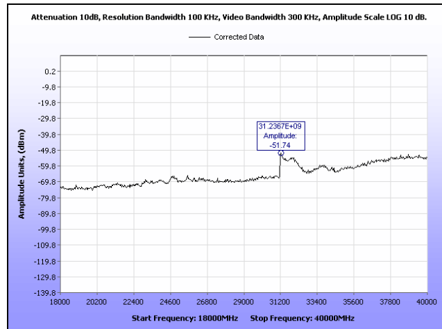
Plot 93. Conducted Spurious Emissions, Low Channel, 18 GHz – 40 GHz, 40 MHz, Horizontal Feed
