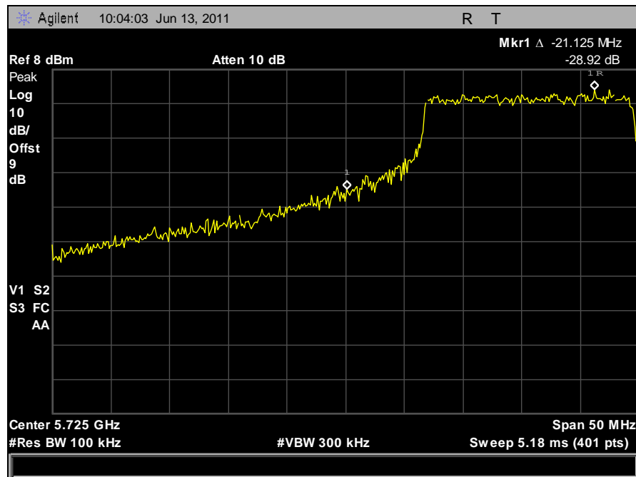
Plot 115. Conducted Band Edge, Low Channel, 40 MHz, Vertical Feed
