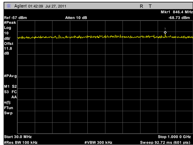
Plot 79. Conducted Spurious Emissions, High Channel, 30 MHz – 1 GHz, 20 MHz, Horizontal Feed
