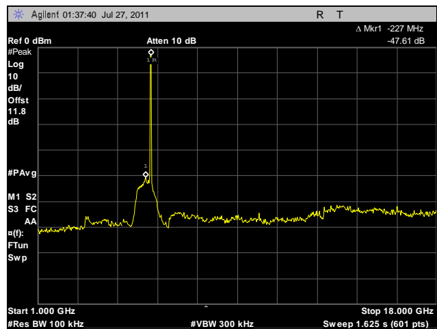
Plot 77. Conducted Spurious Emissions, Mid Channel, 1 GHz – 18 GHz, 20 MHz, Horizontal Feed
