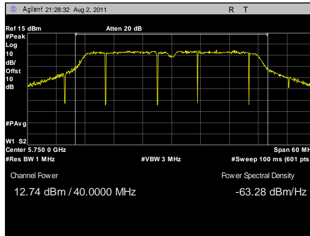
Plot 40. Peak Power Output, Low Channel, 40 MHz, Vertical Feed
