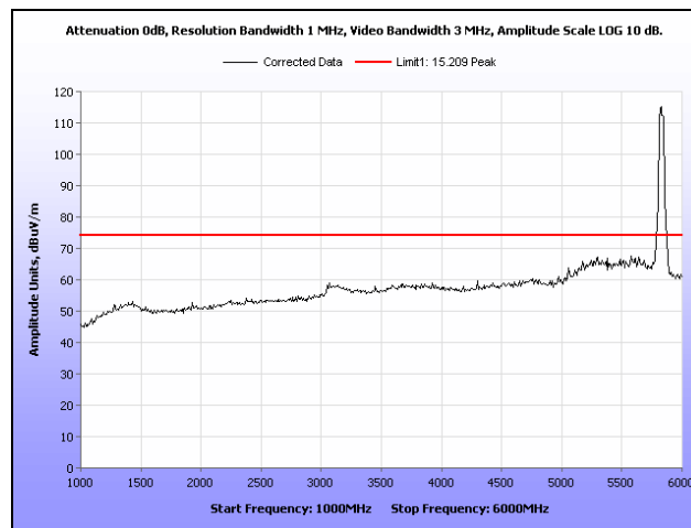
Plot 71. Radiated Spurious Emissions, High Channel, 1 GHz – 6 GHz, Peak, 40 MHz
