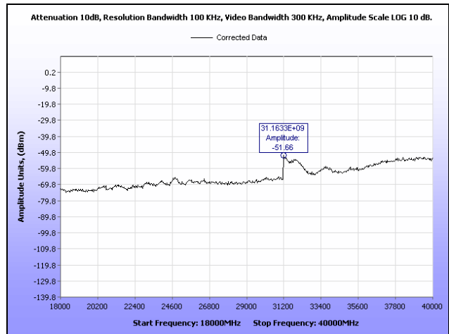
Plot 84. Conducted Spurious Emissions, Low Channel, 18 GHz – 40 GHz, 20 MHz, Vertical Feed
