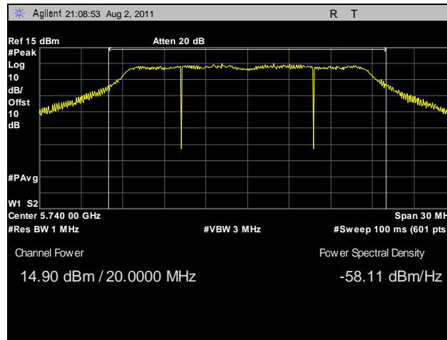
Plot 34. Peak Power Output, Low Channel, 20 MHz, Vertical Feed
