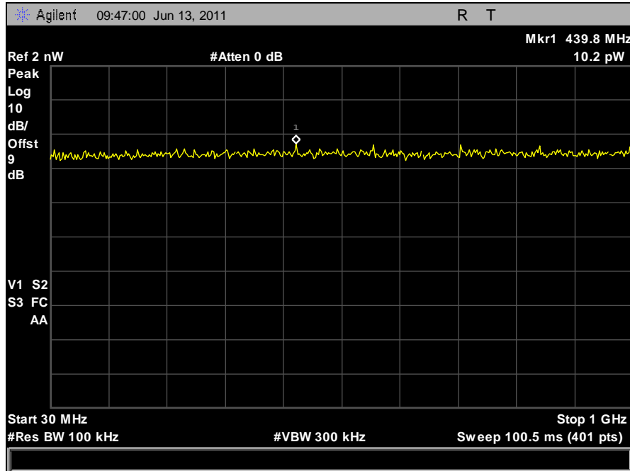
Plot 143. Conducted Receiver Spurious Emissions, Mid Channel, 30 MHz – 1 GHz, Vertical Feed
