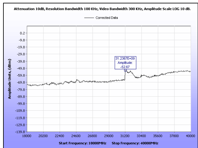
Plot 78. Conducted Spurious Emissions, Mid Channel, 18 GHz – 40 GHz, 20 MHz, Horizontal Feed
