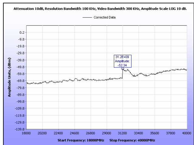
Plot 96. Conducted Spurious Emissions, Mid Channel, 18 GHz – 40 GHz, 40 MHz, Horizontal Feed
