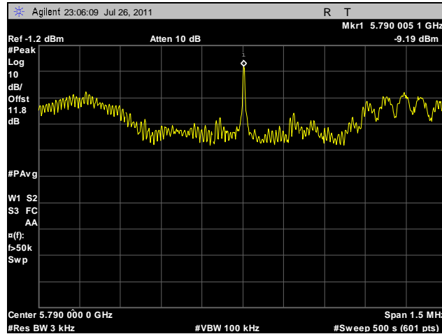
Plot 132. Peak Power Spectral Density, Mid Channel, 40 MHz, Horizontal Feed
