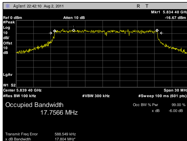
Plot 9. 6 dB Occupied Bandwidth, High Channel, 20 MHz, Horizontal Feed
