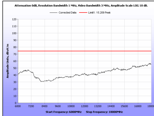
Plot 52. Radiated Spurious Emissions, Mid Channel, 6 GHz – 18 GHz, Peak, 20 MHz
