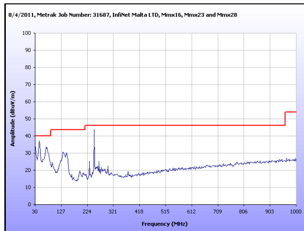
Plot 68. Radiated Spurious Emissions, High Channel, 30 MHz – 1 GHz, 40 MHz
