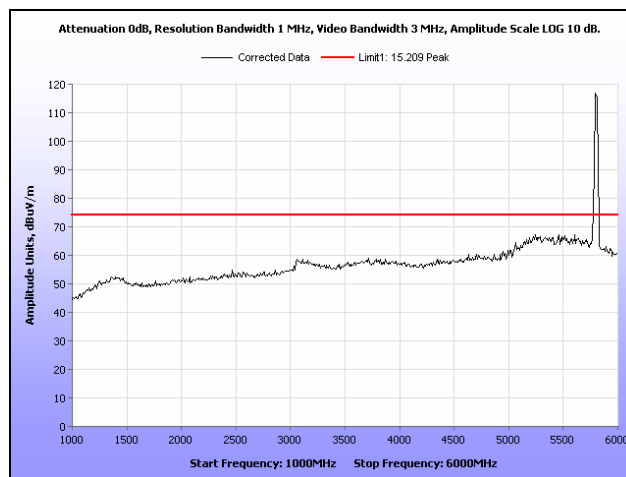
Plot 51. Radiated Spurious Emissions, Mid Channel, 1 GHz – 6 GHz, Peak, 20 MHz
