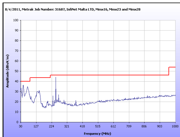
Plot 63. Radiated Spurious Emissions, Mid Channel, 30 MHz – 1 GHz, 40 MHz
