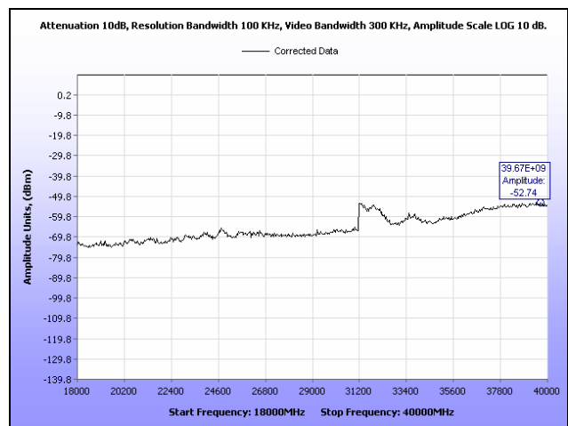
Plot 90. Conducted Spurious Emissions, High Channel, 18 GHz – 40 GHz, 20 MHz, Vertical Feed
