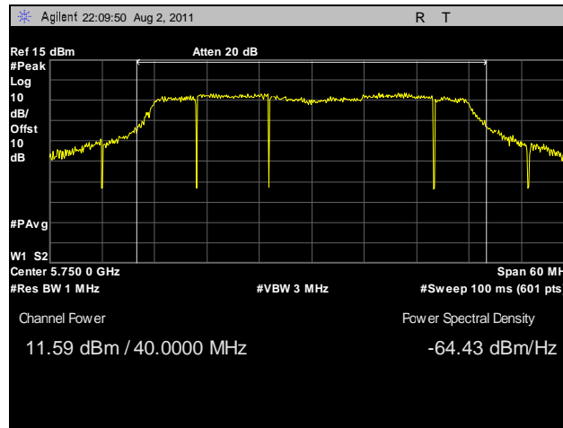
Plot 37. Peak Power Output, Low Channel, 40 MHz, Horizontal Feed
