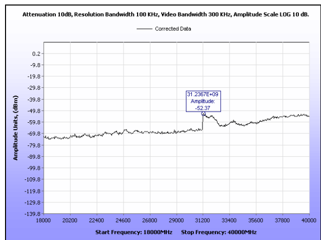
Plot 99. Conducted Spurious Emissions, High Channel, 18 GHz – 40 GHz, 40 MHz, Horizontal Feed
