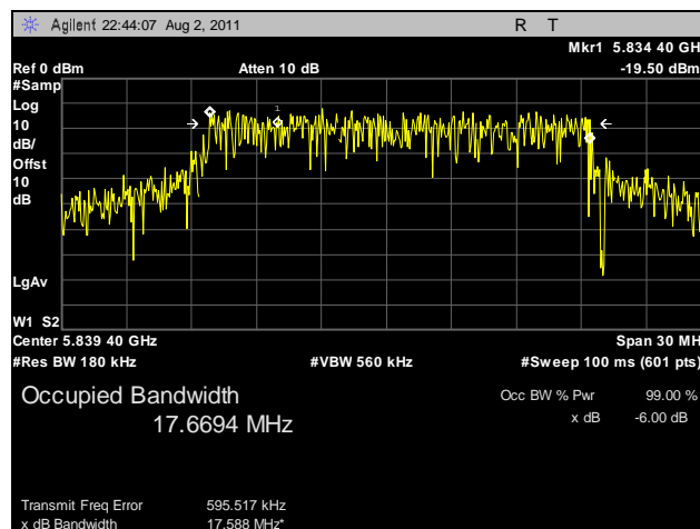
Plot 21. 99% Occupied Bandwidth, High Channel, 20 MHz, Horizontal Feed
