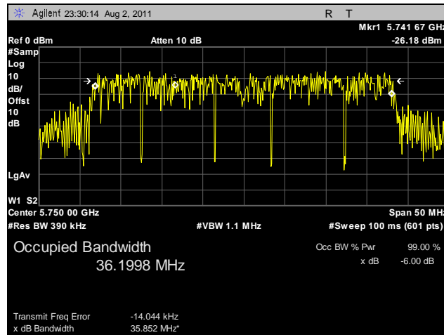
Plot 28. 99% Occupied Bandwidth, Low Channel, 40 MHz, Vertical Feed
