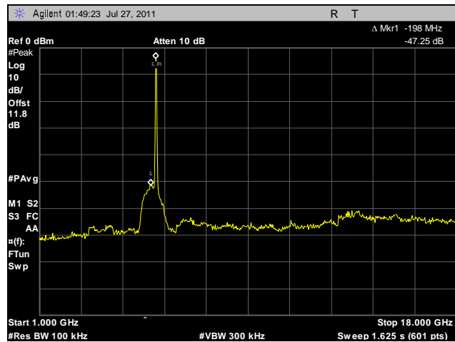
Plot 92. Conducted Spurious Emissions, Low Channel, 1 GHz – 18 GHz, 40 MHz, Horizontal Feed
