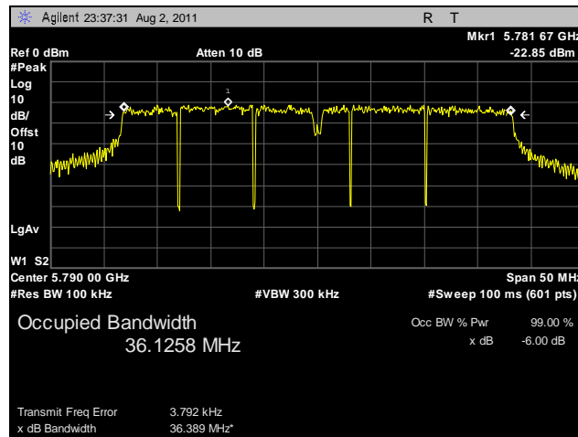
Plot 17. 6 dB Occupied Bandwidth, Mid Channel, 40 MHz, Vertical Feed
