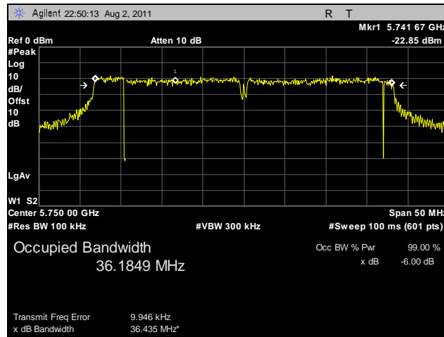
Plot 13. 6 dB Occupied Bandwidth, Low Channel, 40 MHz, Horizontal Feed
