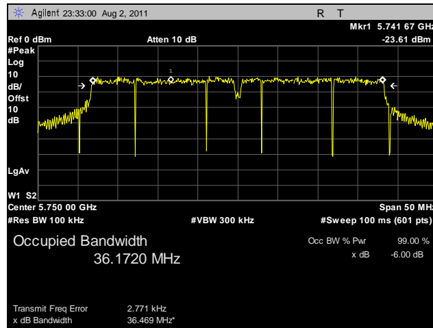
Plot 16. 6 dB Occupied Bandwidth, Low Channel, 40 MHz, Vertical Feed
