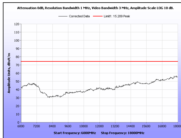
Plot 47. Radiated Spurious Emissions, Low Channel, 6 GHz – 18 GHz, Peak, 20 MHz
