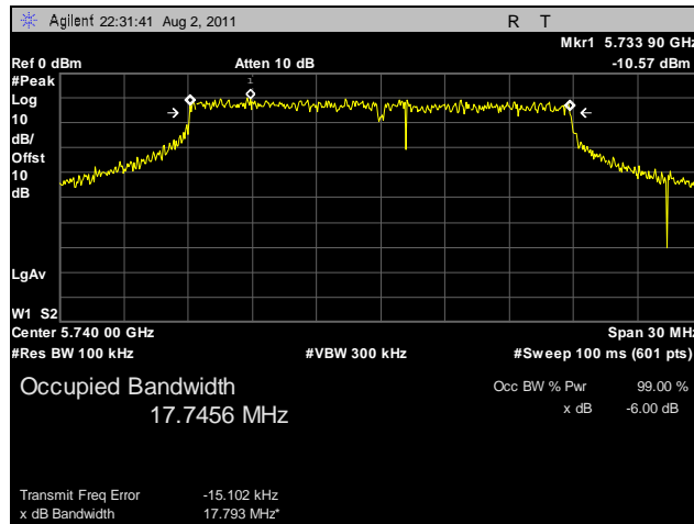
Plot 7. 6 dB Occupied Bandwidth, Low Channel, 20 MHz, Horizontal Feed
