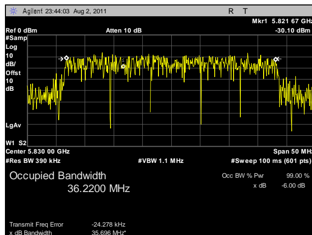
Plot 30. 99% Occupied Bandwidth, High Channel, 40 MHz, Vertical Feed
