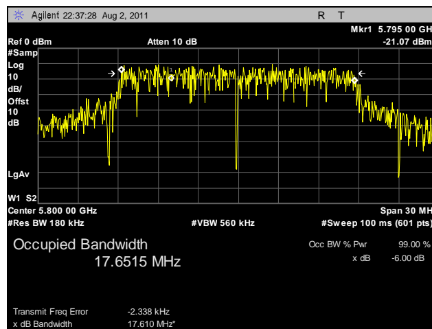
Plot 20. 99% Occupied Bandwidth, Mid Channel, 20 MHz, Horizontal Feed
