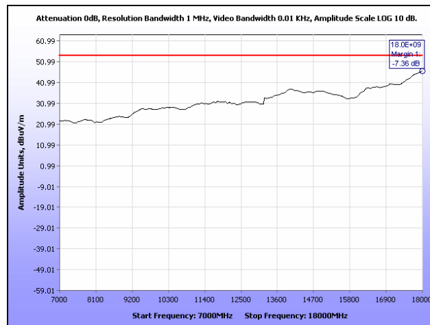
Plot 60. Radiated Spurious Emissions, Low Channel, 7 GHz – 18 GHz, 40 MHz
