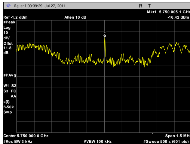
Plot 136. Peak Power Spectral Density, Low Channel, 40 MHz, Vertical Feed
