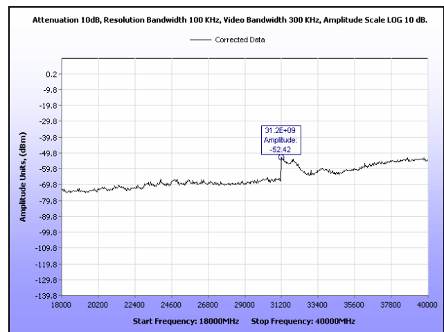
Plot 108. Conducted Spurious Emissions, High Channel, 18 GHz – 40 GHz, 40 MHz, Vertical Feed
