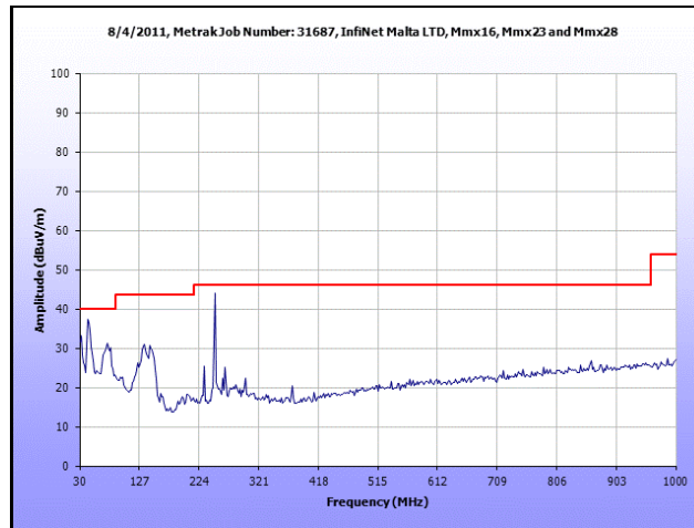
Plot 43. Radiated Spurious Emissions, Low Channel, 30 MHz – 1 GHz, 20 MHz
