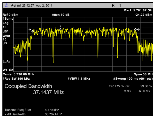
Plot 29. 99% Occupied Bandwidth, Mid Channel, 40 MHz, Vertical Feed
