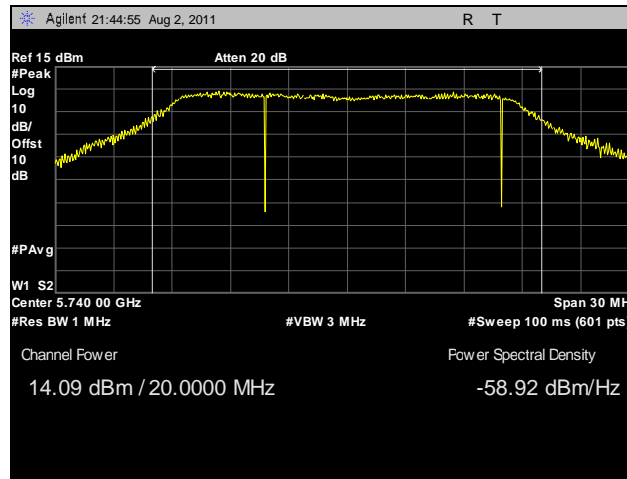
Plot 31. Peak Power Output, Low Channel, 20 MHz, Horizontal Feed
