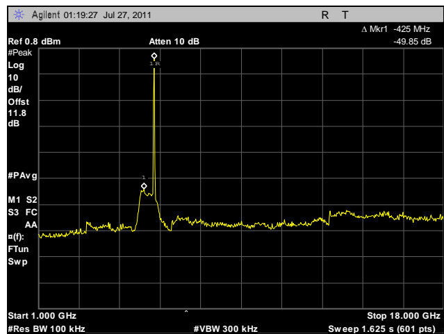
Plot 89. Conducted Spurious Emissions, High Channel, 1 GHz – 18 GHz, 20 MHz, Vertical Feed
