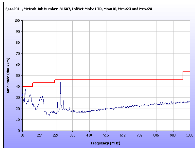
Plot 58. Radiated Spurious Emissions, Low Channel, 30 MHz – 1 GHz, 40 MHz
