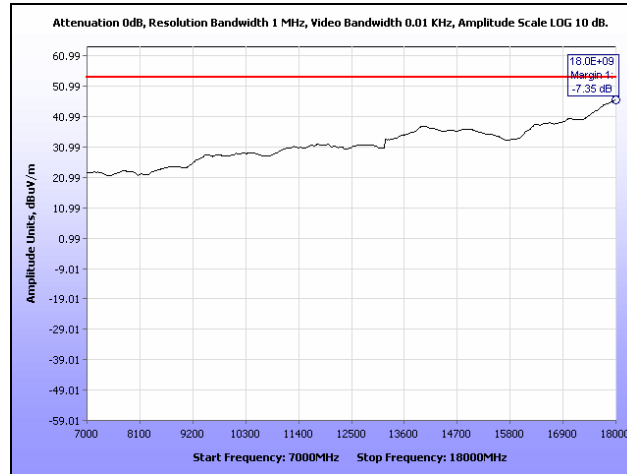
Plot 55. Radiated Spurious Emissions, High Channel, 7 GHz – 18 GHz, 20 MHz
