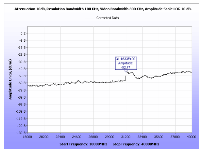
Plot 81. Conducted Spurious Emissions, High Channel, 18 GHz – 40 GHz, 20 MHz, Horizontal Feed
