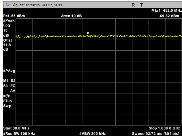
Plot 94. Conducted Spurious Emissions, Mid Channel, 30 MHz – 1 GHz, 40 MHz, Horizontal Feed
