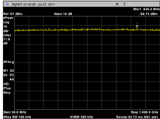
Plot 67. Conducted Spurious Emissions, High Channel, 30 MHz – 1 GHz, 20 MHz, Horizontal Feed
