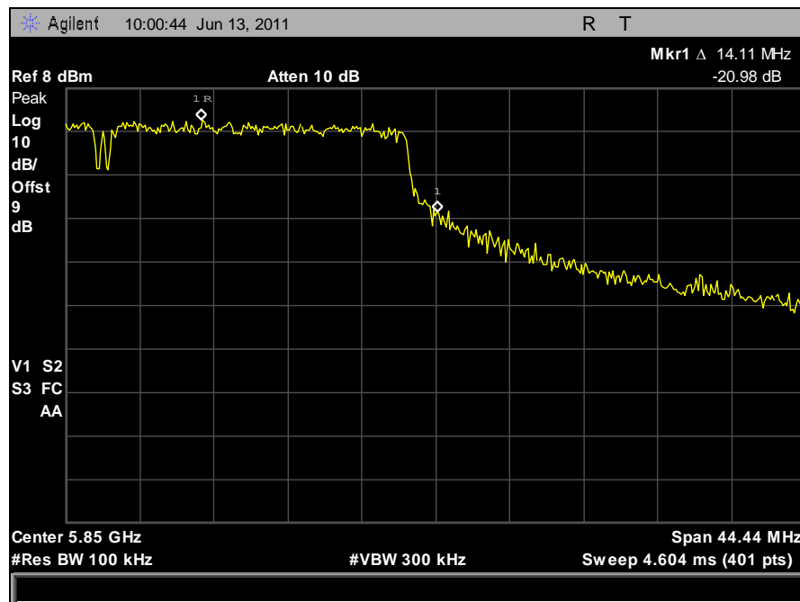
Plot 102. Conducted Band Edge, High Channel, 40 MHz, Horizontal Feed
