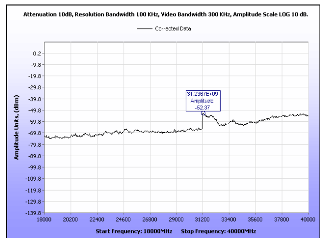
Plot 87. Conducted Spurious Emissions, High Channel, 18 GHz – 40 GHz, 40 MHz, Horizontal Feed
