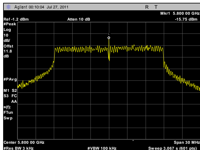
Plot 113. Peak Power Spectral Density, Mid Channel, 20 MHz, Vertical Feed, Determination
