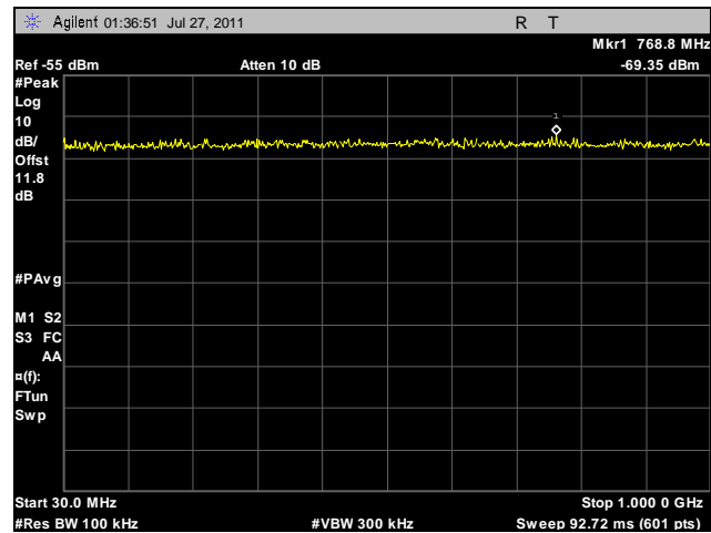
Plot 91. Conducted Spurious Emissions, Mid Channel, 30 MHz – 1 GHz, 40 MHz, Vertical Feed
