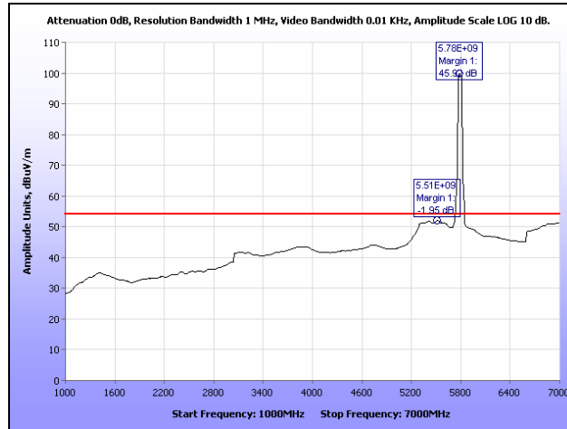
Plot 52. Radiated Spurious Emissions, Mid Channel, 1 GHz – 7 GHz, 40 MHz
