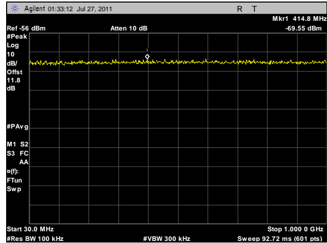
Plot 64. Conducted Spurious Emissions, Mid Channel, 30 MHz – 1 GHz, 20 MHz, Horizontal Feed
