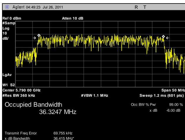
Plot 17. 99% Occupied Bandwidth, Mid Channel, 40 MHz
