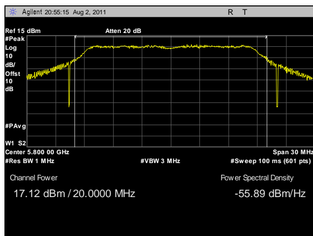
Plot 23. Peak Power Output, Mid Channel, 20 MHz, Vertical Feed
