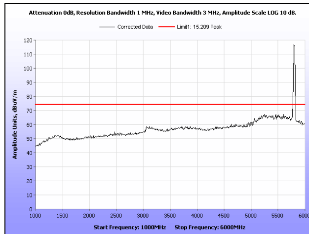
Plot 39. Radiated Spurious Emissions, Mid Channel, 1 GHz – 6 GHz, Peak, 20 MHz
