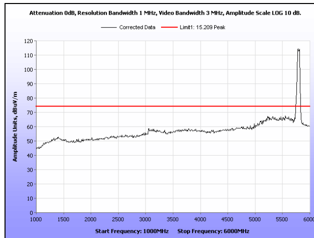
Plot 54. Radiated Spurious Emissions, Mid Channel, 1 GHz – 6 GHz, Peak, 40 MHz
