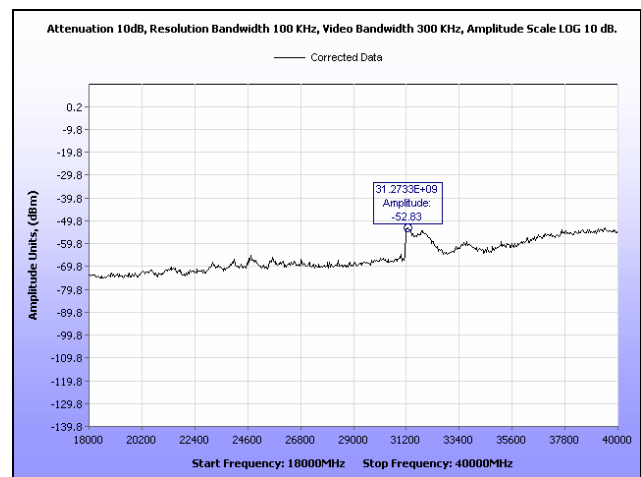
Plot 93. Conducted Spurious Emissions, Mid Channel, 18 GHz – 40 GHz, 40 MHz, Vertical Feed
