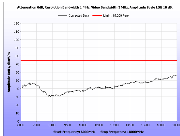
Plot 55. Radiated Spurious Emissions, Mid Channel, 6 GHz – 18 GHz, Peak, 40 MHz
