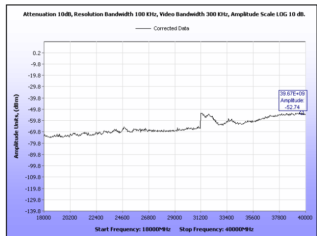
Plot 78. Conducted Spurious Emissions, High Channel, 18 GHz – 40 GHz, 20 MHz, Vertical Feed
