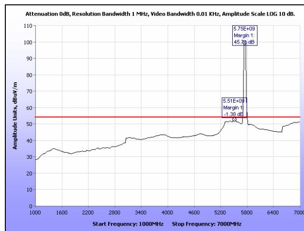
Plot 47. Radiated Spurious Emissions, Low Channel, 1 GHz – 7 GHz, 40 MHz
