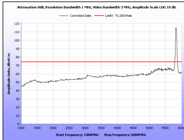
Plot 59. Radiated Spurious Emissions, High Channel, 1 GHz – 6 GHz, Peak, 40 MHz
