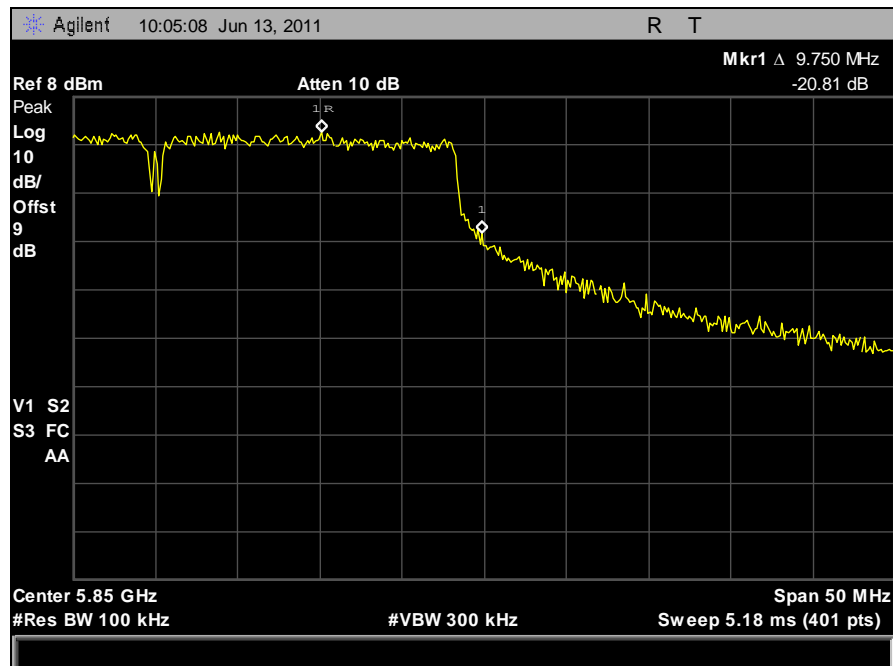
Plot 104. Conducted Band Edge, High Channel, 40 MHz, Vertical Feed
