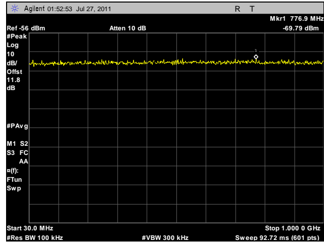
Plot 85. Conducted Spurious Emissions, High Channel, 30 MHz – 1 GHz, 40 MHz, Horizontal Feed
