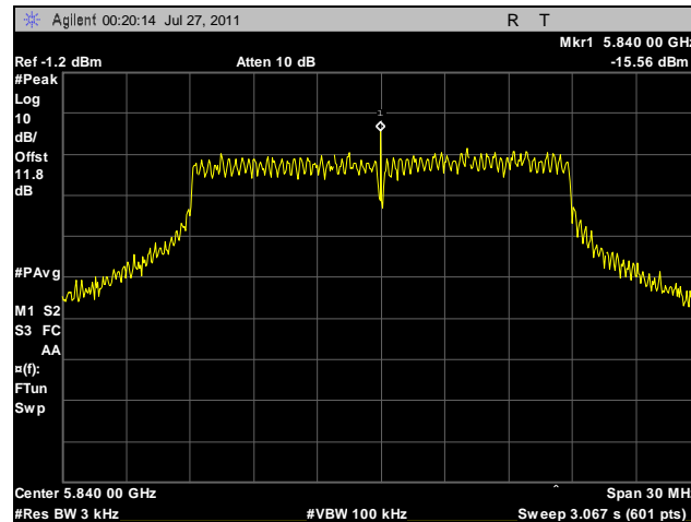
Plot 115. Peak Power Spectral Density, High Channel, 20 MHz, Vertical Feed, Determination
