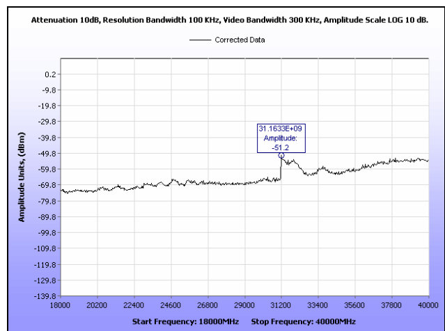
Plot 90. Conducted Spurious Emissions, Low Channel, 18 GHz – 40 GHz, 40 MHz, Vertical Feed
