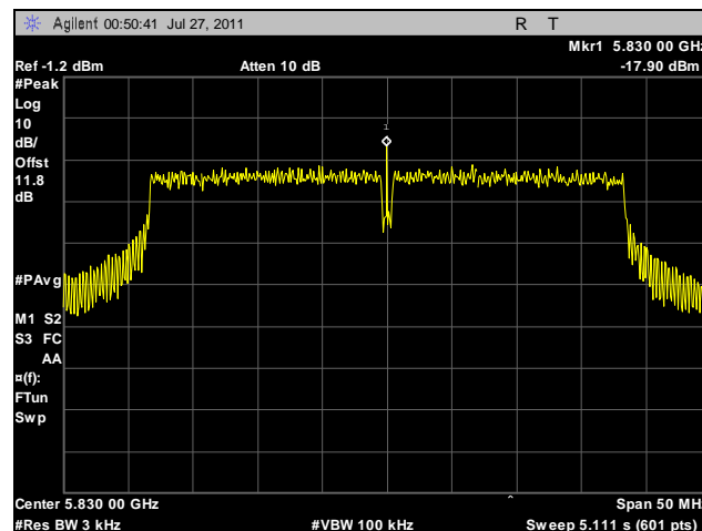
Plot 127. Peak Power Spectral Density, High Channel, 40 MHz, Vertical Feed, Determination
