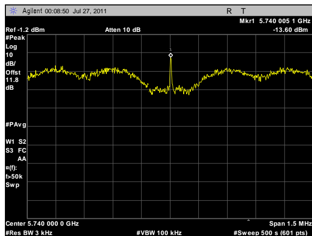
Plot 112. Peak Power Spectral Density, Low Channel, 20 MHz, Vertical Feed
