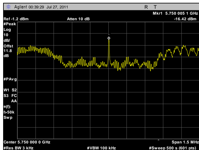
Plot 124. Peak Power Spectral Density, Low Channel, 40 MHz, Vertical Feed
