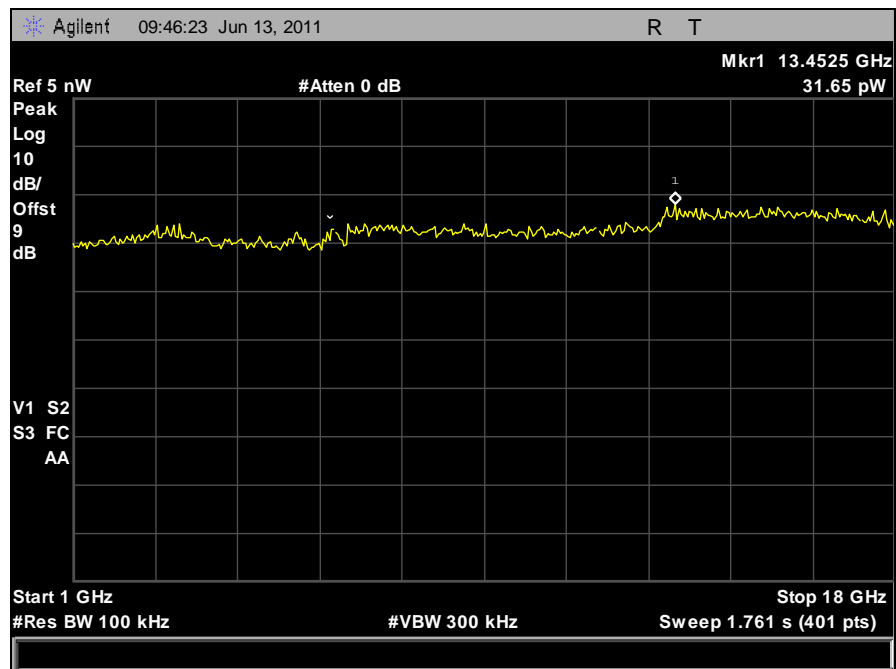
Plot 132. Conducted Receiver Spurious Emissions, Mid Channel, 1 GHz – 18 GHz, Vertical Feed
