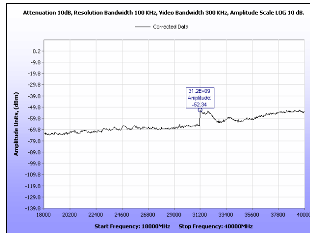
Plot 84. Conducted Spurious Emissions, Mid Channel, 18 GHz – 40 GHz, 40 MHz, Horizontal Feed
