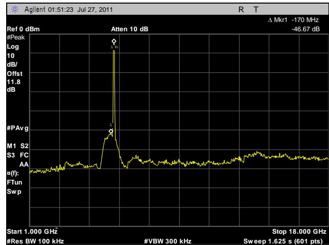
Plot 83. Conducted Spurious Emissions, Mid Channel, 1 GHz – 18 GHz, 40 MHz, Horizontal Feed
