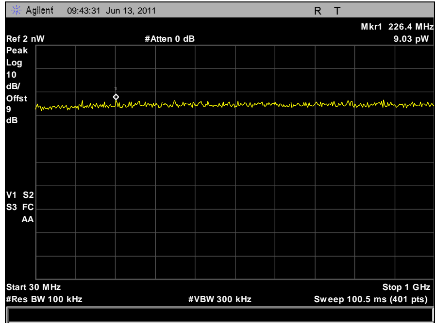
Plot 129. Conducted Receiver Spurious Emissions, Mid Channel, 30 MHz – 1 GHz, Horizontal Feed
