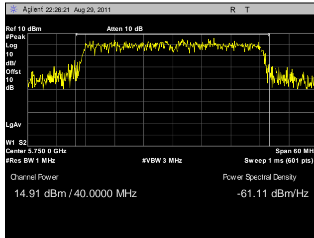
Plot 25. Peak Power Output, Low Channel, 40 MHz, Horizontal Feed
