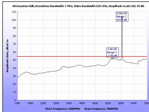
Plot 42. Radiated Spurious Emissions, High Channel, 1 GHz – 7 GHz, 20 MHz
