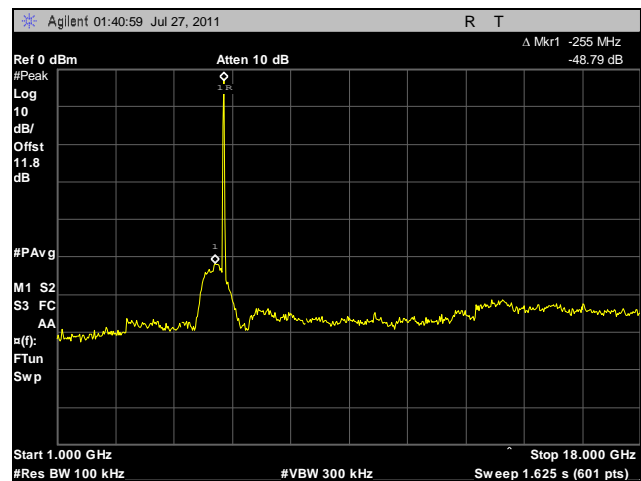
Plot 68. Conducted Spurious Emissions, High Channel, 1 GHz – 18 GHz, 20 MHz, Horizontal Feed
