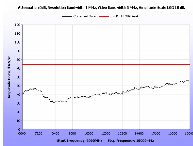
Plot 50. Radiated Spurious Emissions, Low Channel, 6 GHz – 18 GHz, Peak, 40 MHz
