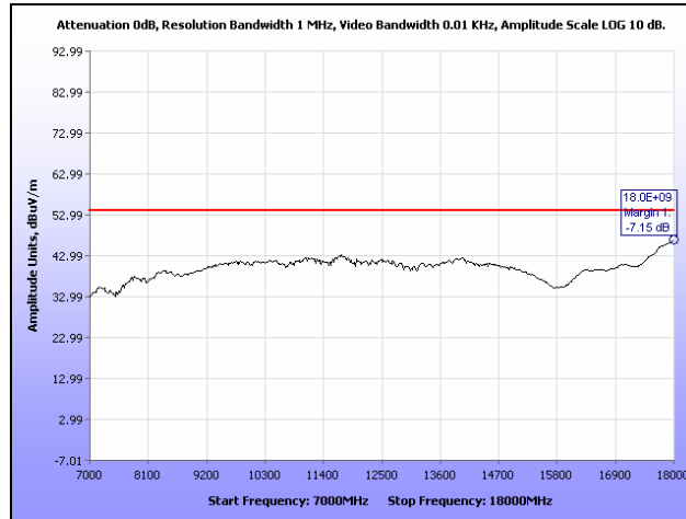
Plot 43. Radiated Spurious Emissions, High Channel, 7 GHz – 18 GHz, 20 MHz
