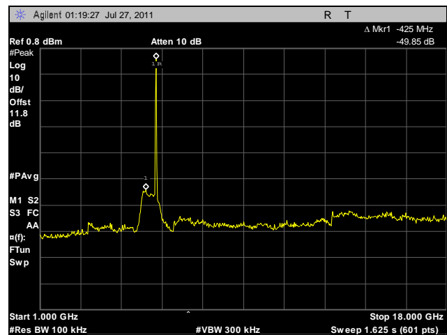
Plot 77. Conducted Spurious Emissions, High Channel, 1 GHz – 18 GHz, 20 MHz, Vertical Feed
