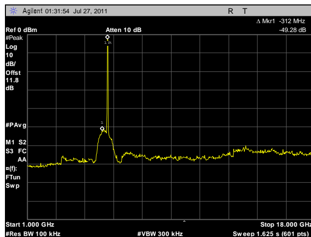
Plot 62. Conducted Spurious Emissions, Low Channel, 1 GHz – 18 GHz, 20 MHz, Horizontal Feed
