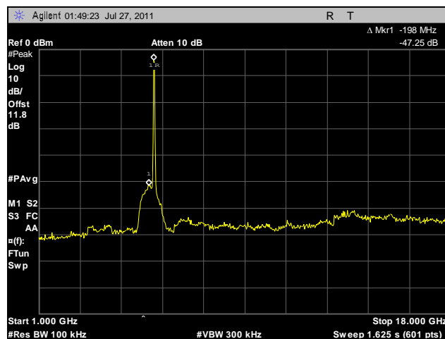
Plot 80. Conducted Spurious Emissions, Low Channel, 1 GHz – 18 GHz, 40 MHz, Horizontal Feed
