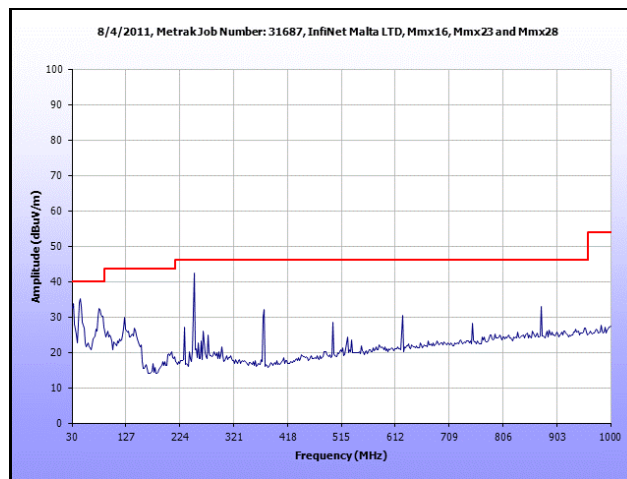
Plot 41. Radiated Spurious Emissions, High Channel, 30 MHz – 1 GHz, 20 MHz
