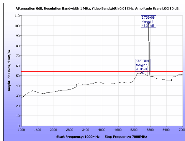
Plot 32. Radiated Spurious Emissions, Low Channel, 1 GHz – 7 GHz, 20 MHz
