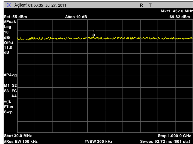
Plot 82. Conducted Spurious Emissions, Mid Channel, 30 MHz – 1 GHz, 40 MHz, Horizontal Feed
