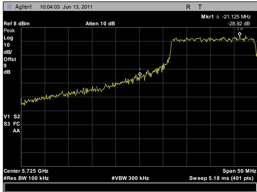
Plot 103. Conducted Band Edge, Low Channel, 40 MHz, Vertical Feed
