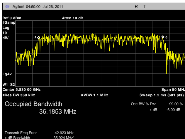
Plot 18. 99% Occupied Bandwidth, High Channel, 40 MHz
