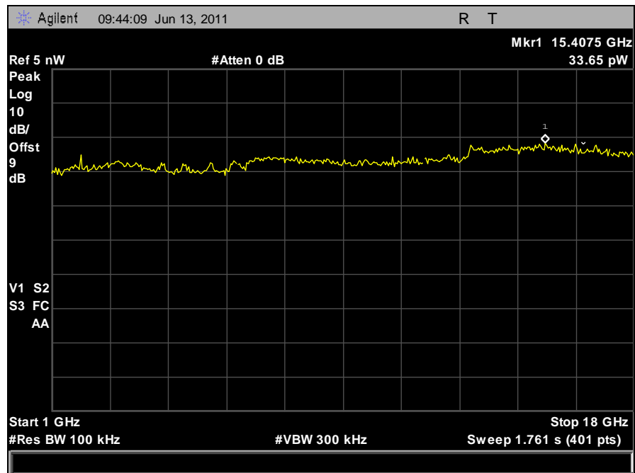
Plot 130. Conducted Receiver Spurious Emissions, Mid Channel, 1 GHz – 18 GHz, Horizontal Feed
