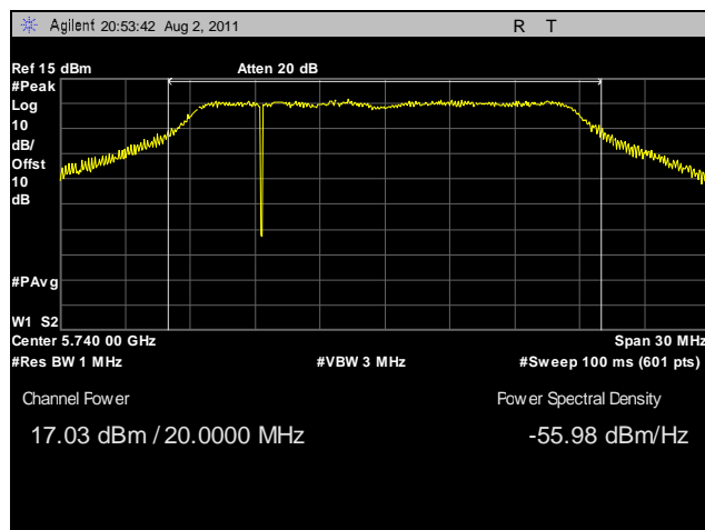
Plot 22. Peak Power Output, Low Channel, 20 MHz, Vertical Feed
