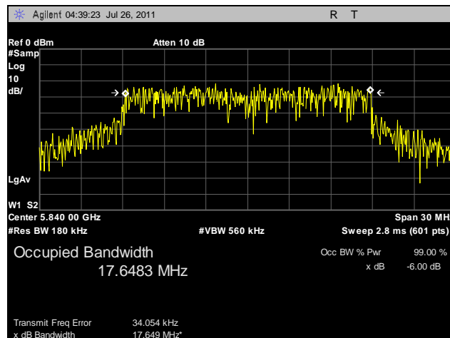
Plot 15. 99% Occupied Bandwidth, High Channel, 20 MHz
