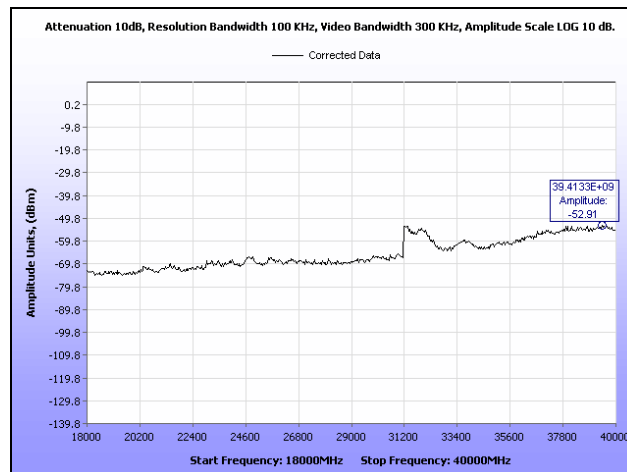
Plot 63. Conducted Spurious Emissions, Low Channel, 18 GHz – 40 GHz, 20 MHz, Horizontal Feed
