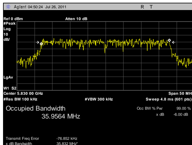
Plot 12. 6 dB Occupied Bandwidth, High Channel, 40 MHz
