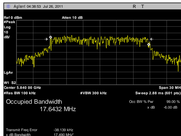
Plot 9. 6 dB Occupied Bandwidth, High Channel, 20 MHz
