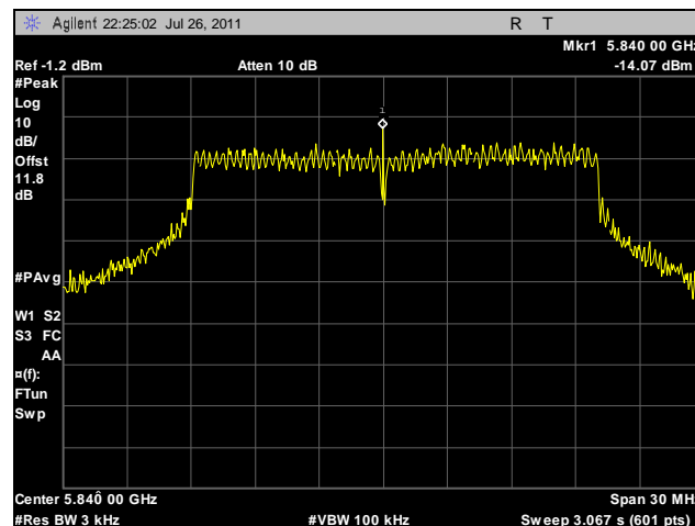
Plot 109. Peak Power Spectral Density, High Channel, 20 MHz, Horizontal Feed, Determination
