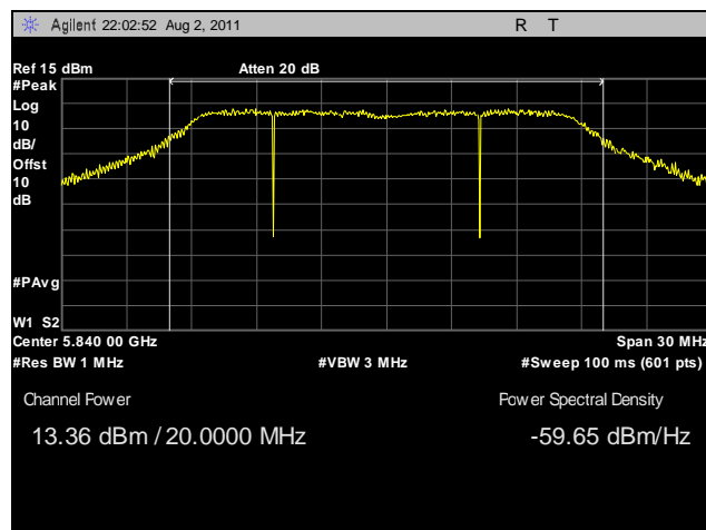
Plot 21. Peak Power Output, High Channel, 20 MHz, Horizontal Feed
