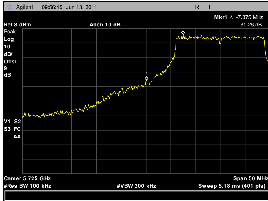
Plot 97. Conducted Band Edge, Low Channel, 20 MHz, Horizontal Feed
