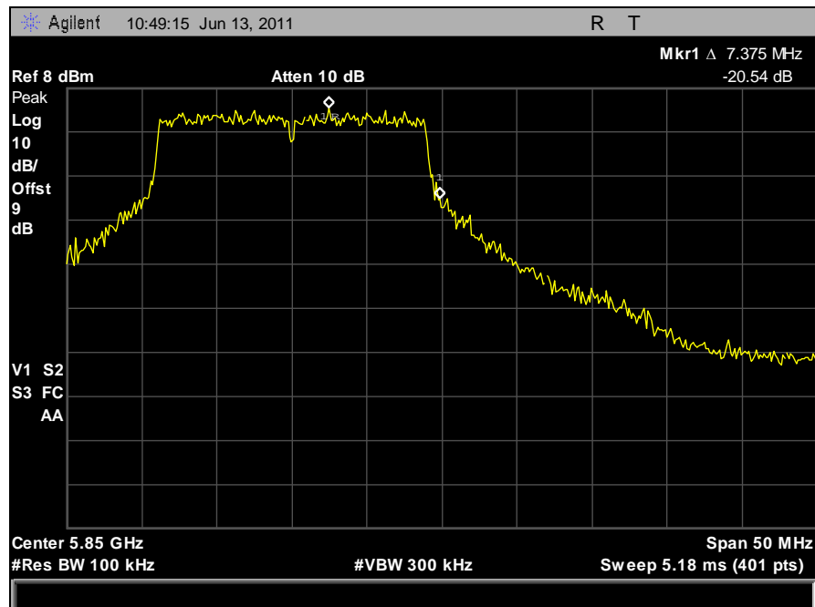
Plot 100. Conducted Band Edge, High Channel, 20 MHz, Vertical Feed
