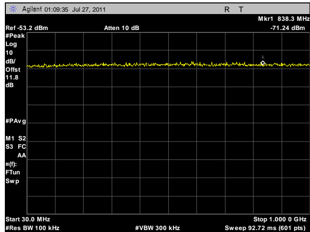
Plot 70. Conducted Spurious Emissions, Low Channel, 30 MHz – 1 GHz, 20 MHz, Vertical Feed
