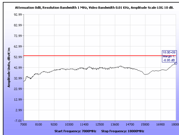
Plot 48. Radiated Spurious Emissions, Low Channel, 7 GHz – 18 GHz, 40 MHz
