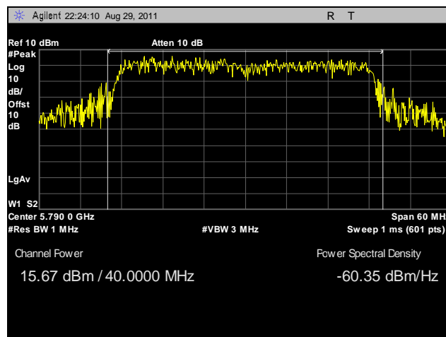
Plot 29. Peak Power Output, Mid Channel, 40 MHz, Vertical Feed
