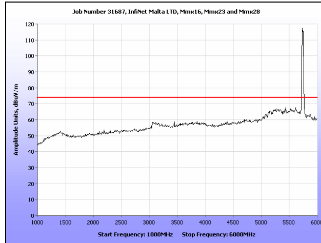
Plot 34. Radiated Spurious Emissions, Low Channel, 1 GHz – 6 GHz, Peak, 20 MHz
