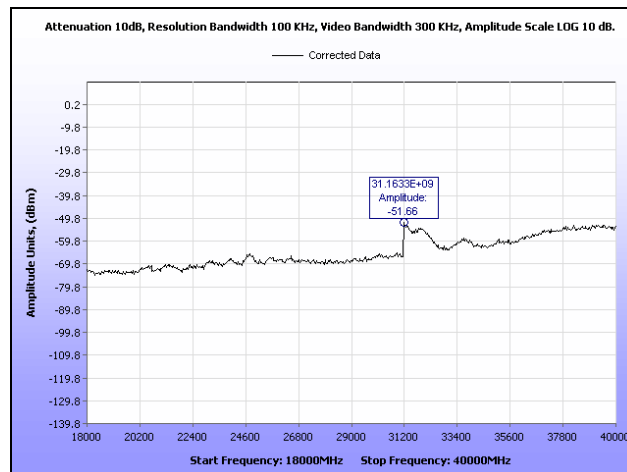
Plot 72. Conducted Spurious Emissions, Low Channel, 18 GHz – 40 GHz, 20 MHz, Vertical Feed
