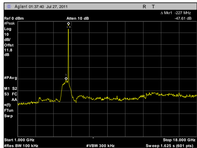
Plot 65. Conducted Spurious Emissions, Mid Channel, 1 GHz – 18 GHz, 20 MHz, Horizontal Feed
