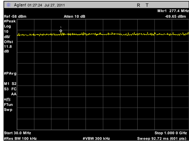
Plot 94. Conducted Spurious Emissions, High Channel, 30 MHz – 1 GHz, 40 MHz, Vertical Feed
