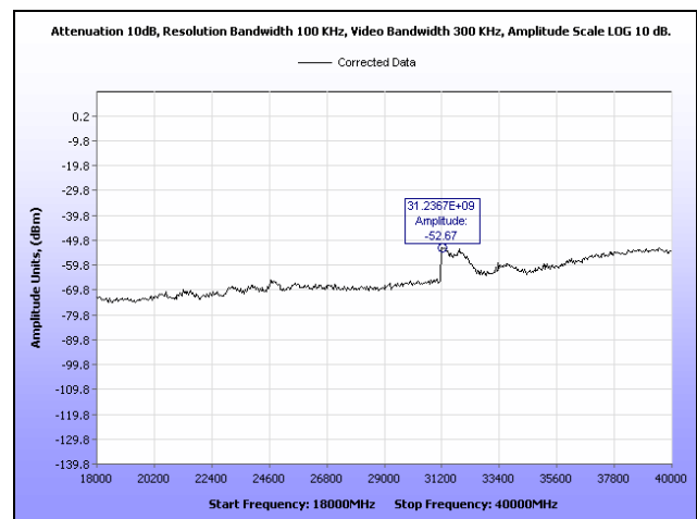
Plot 66. Conducted Spurious Emissions, Mid Channel, 18 GHz – 40 GHz, 20 MHz, Horizontal Feed
