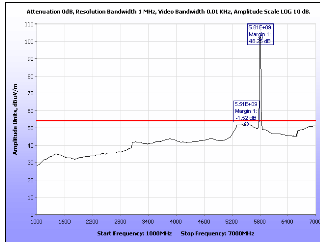
Plot 37. Radiated Spurious Emissions, Mid Channel, 1 GHz – 7 GHz, 20 MHz
