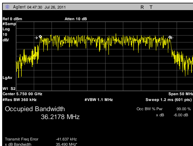
Plot 16. 99% Occupied Bandwidth, Low Channel, 40 MHz
