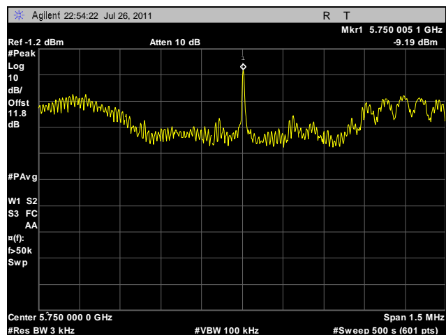
Plot 118. Peak Power Spectral Density, Low Channel, 40 MHz, Horizontal Feed
