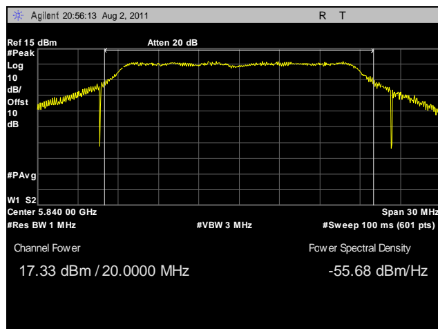
Plot 24. Peak Power Output, High Channel, 20 MHz, Vertical Feed
