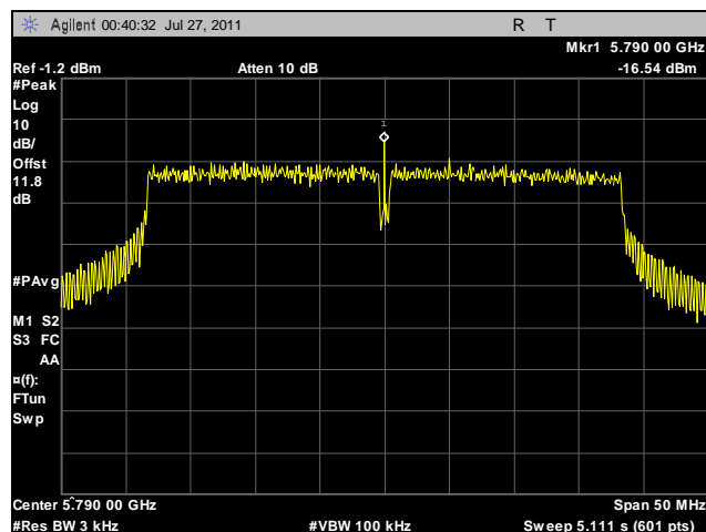
Plot 125. Peak Power Spectral Density, Mid Channel, 40 MHz, Vertical Feed, Determination
