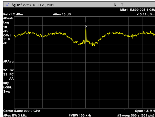
Plot 108. Peak Power Spectral Density, Mid Channel, 20 MHz, Horizontal Feed
