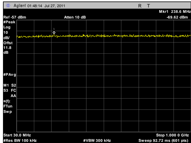
Plot 79. Conducted Spurious Emissions, Low Channel, 30 MHz – 1 GHz, 40 MHz, Horizontal Feed
