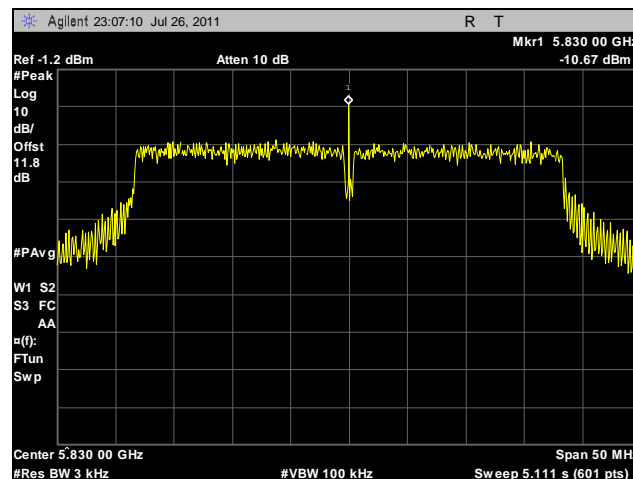
Plot 121. Peak Power Spectral Density, High Channel, 40 MHz, Horizontal Feed, Determination
