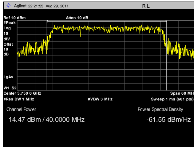
Plot 28. Peak Power Output, Low Channel, 40 MHz, Vertical Feed
