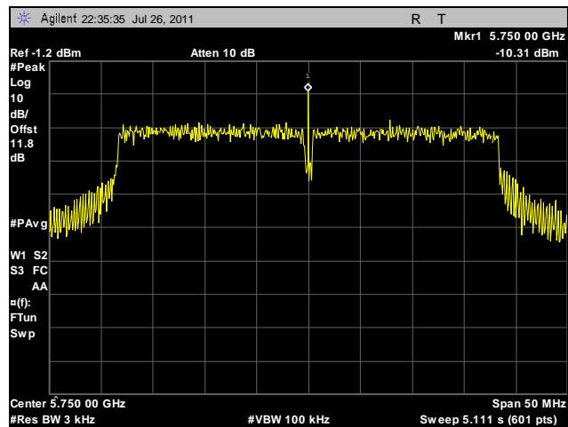
Plot 117. Peak Power Spectral Density, Low Channel, 40 MHz, Horizontal Feed, Determination
