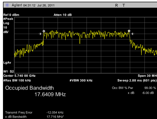
Plot 7. 6 dB Occupied Bandwidth, Low Channel, 20 MHz
