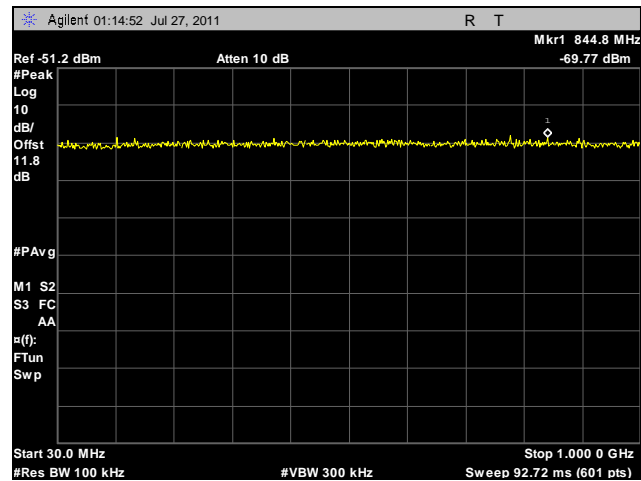
Plot 73. Conducted Spurious Emissions, Mid Channel, 30 MHz – 1 GHz, 20 MHz, Vertical Feed
