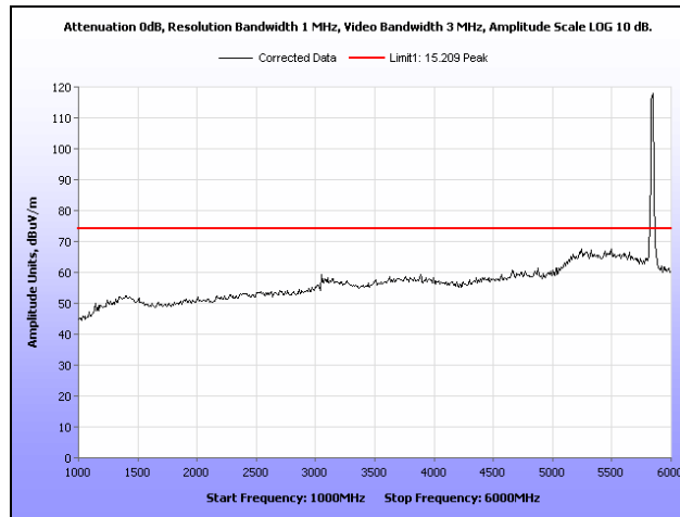
Plot 44. Radiated Spurious Emissions, High Channel, 1 GHz – 6 GHz, Peak, 20 MHz
