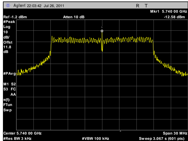
Plot 105. Peak Power Spectral Density, Low Channel, 20 MHz, Horizontal Feed, Determination
