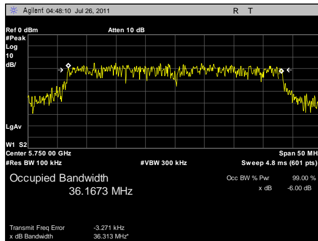
Plot 10. 6 dB Occupied Bandwidth, Low Channel, 40 MHz
