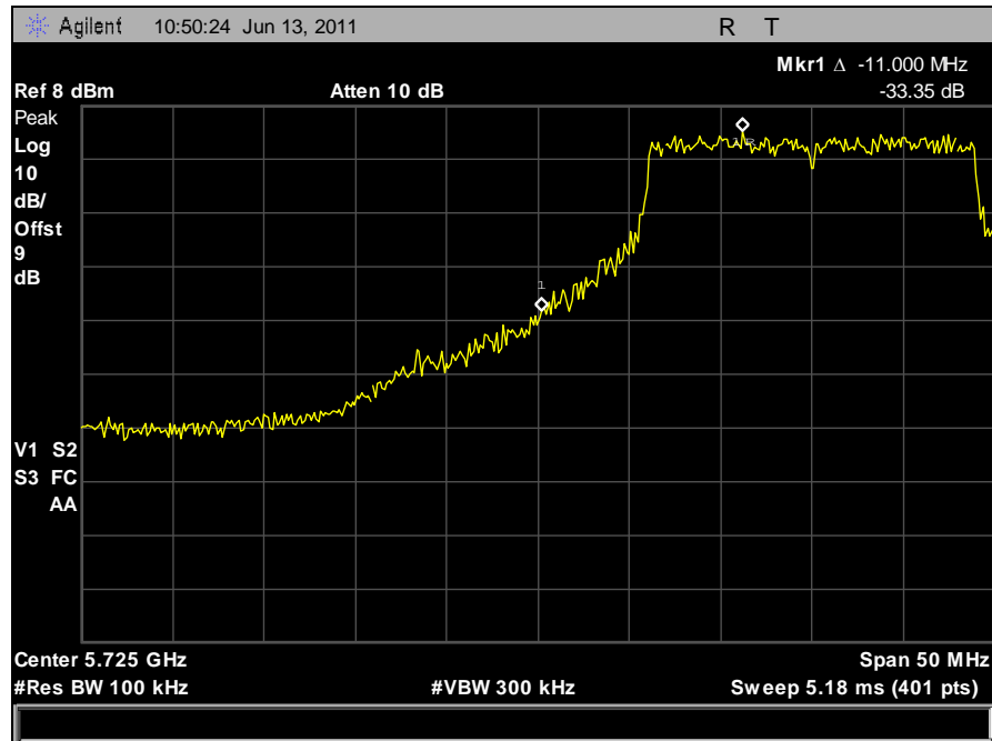
Plot 99. Conducted Band Edge, Low Channel, 20 MHz, Vertical Feed
