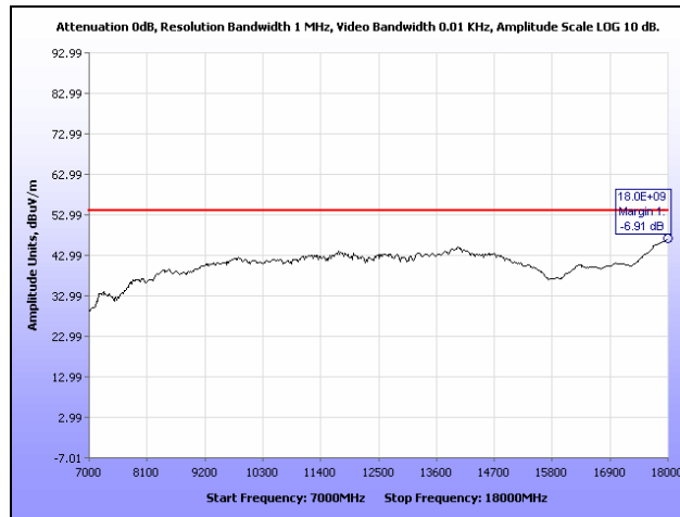
Plot 53. Radiated Spurious Emissions, Mid Channel, 7 GHz – 18 GHz, 40 MHz
