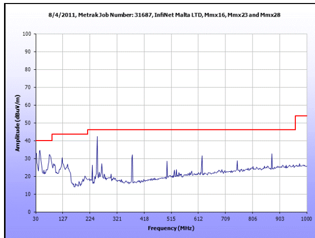
Plot 51. Radiated Spurious Emissions, Mid Channel, 30 MHz – 1 GHz, 40 MHz
