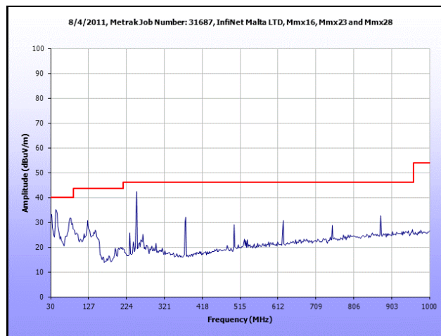
Plot 56. Radiated Spurious Emissions, High Channel, 30 MHz – 1 GHz, 40 MHz
