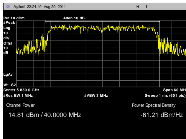
Plot 30. Peak Power Output, High Channel, 40 MHz, Vertical Feed
