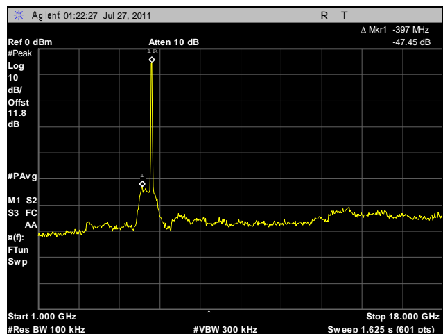
Plot 89. Conducted Spurious Emissions, Low Channel, 1 GHz – 18 GHz, 40 MHz, Vertical Feed
