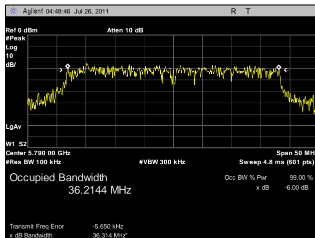
Plot 11. 6 dB Occupied Bandwidth, Mid Channel, 40 MHz
