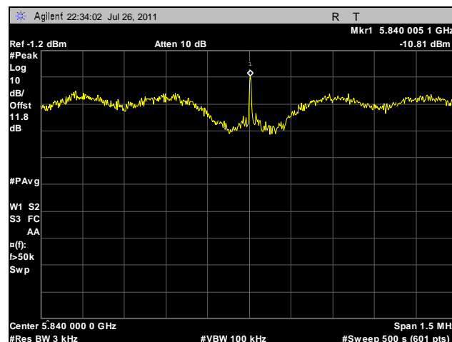
Plot 110. Peak Power Spectral Density, High Channel, 20 MHz, Horizontal Feed
