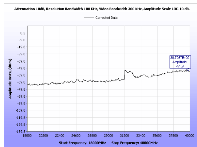
Plot 75. Conducted Spurious Emissions, Mid Channel, 18 GHz – 40 GHz, 20 MHz, Vertical Feed
