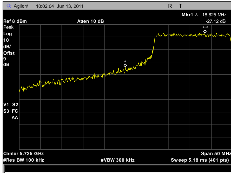
Plot 101. Conducted Band Edge, Low Channel, 40 MHz, Horizontal Feed
