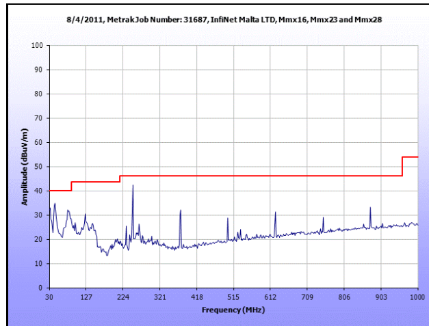
Plot 46. Radiated Spurious Emissions, Low Channel, 30 MHz – 1 GHz, 40 MHz
