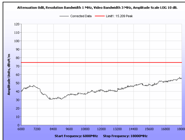
Plot 45. Radiated Spurious Emissions, High Channel, 6 GHz – 18 GHz, Peak, 20 MHz
