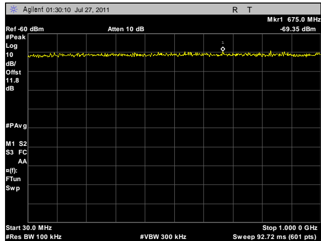
Plot 61. Conducted Spurious Emissions, Low Channel, 30 MHz – 1 GHz, 20 MHz, Horizontal Feed
