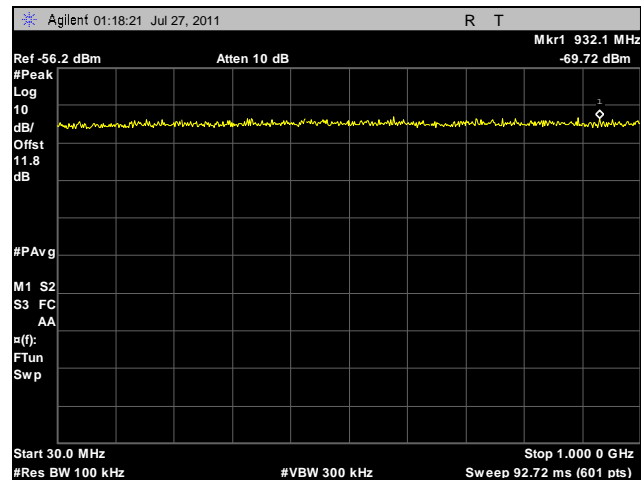
Plot 76. Conducted Spurious Emissions, High Channel, 30 MHz – 1 GHz, 20 MHz, Vertical Feed
