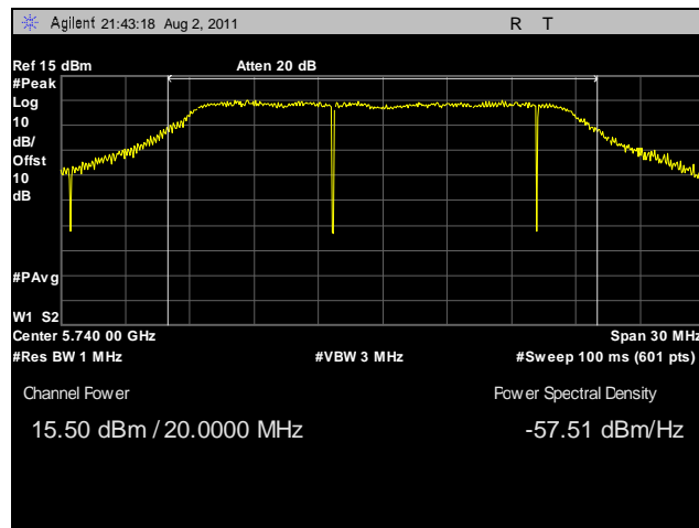
Plot 19. Peak Power Output, Low Channel, 20 MHz, Horizontal Feed
