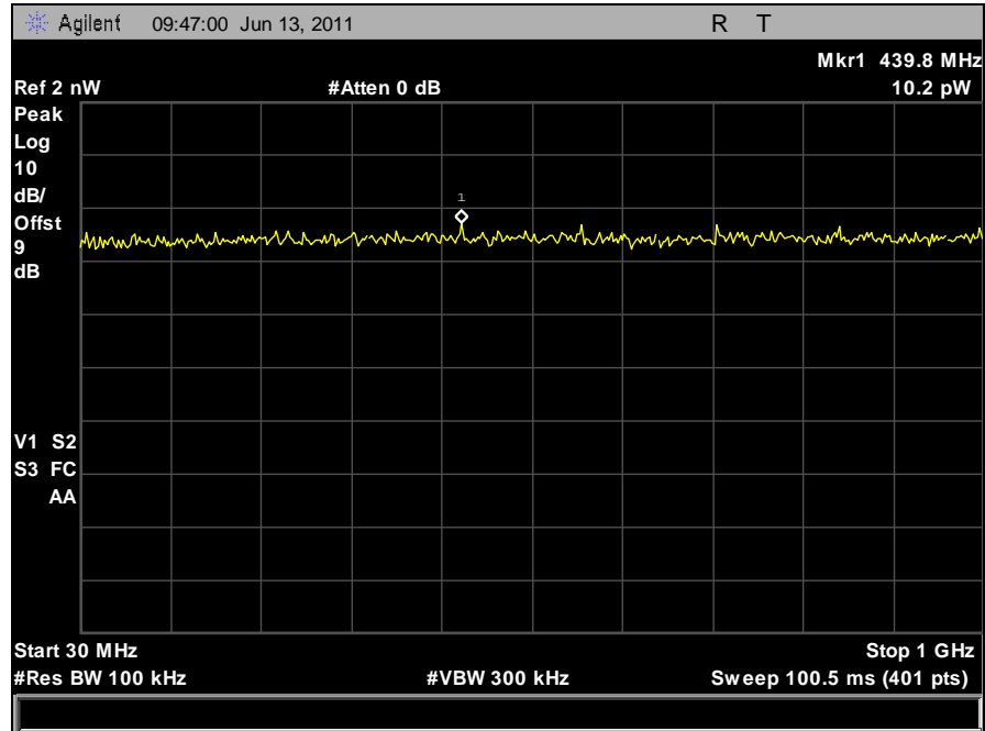
Plot 131. Conducted Receiver Spurious Emissions, Mid Channel, 30 MHz – 1 GHz, Vertical Feed
