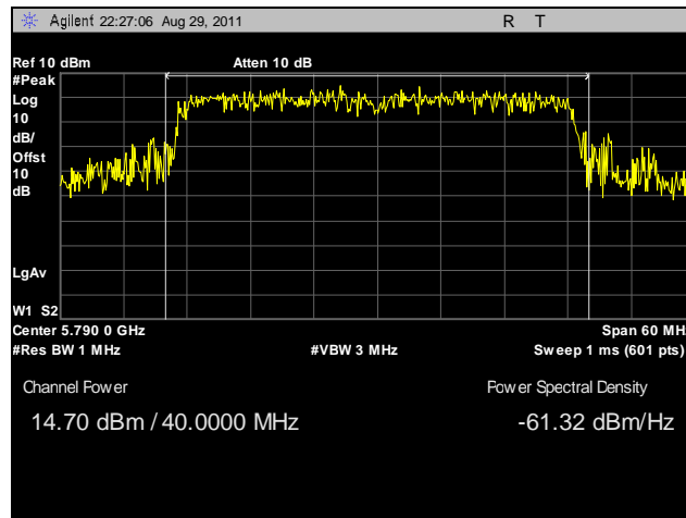
Plot 26. Peak Power Output, Mid Channel, 40 MHz, Horizontal Feed
