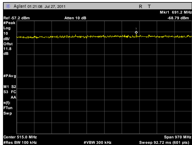
Plot 88. Conducted Spurious Emissions, Low Channel, 30 MHz – 1 GHz, 40 MHz, Vertical Feed
