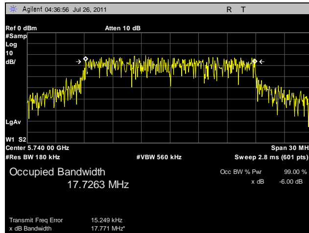
Plot 13. 99% Occupied Bandwidth, Low Channel, 20 MHz
