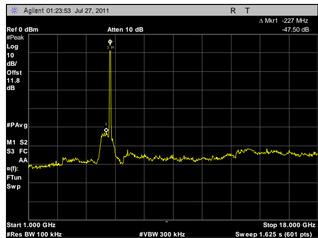
Plot 92. Conducted Spurious Emissions, Mid Channel, 1 GHz – 18 GHz, 40 MHz, Vertical Feed
