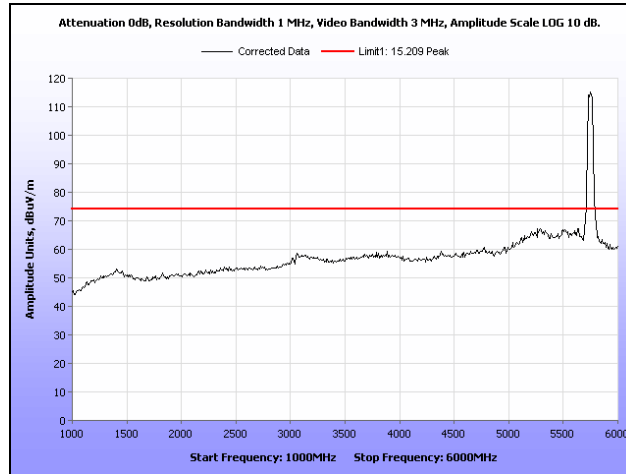
Plot 49. Radiated Spurious Emissions, Low Channel, 1 GHz – 6 GHz, Peak, 40 MHz
