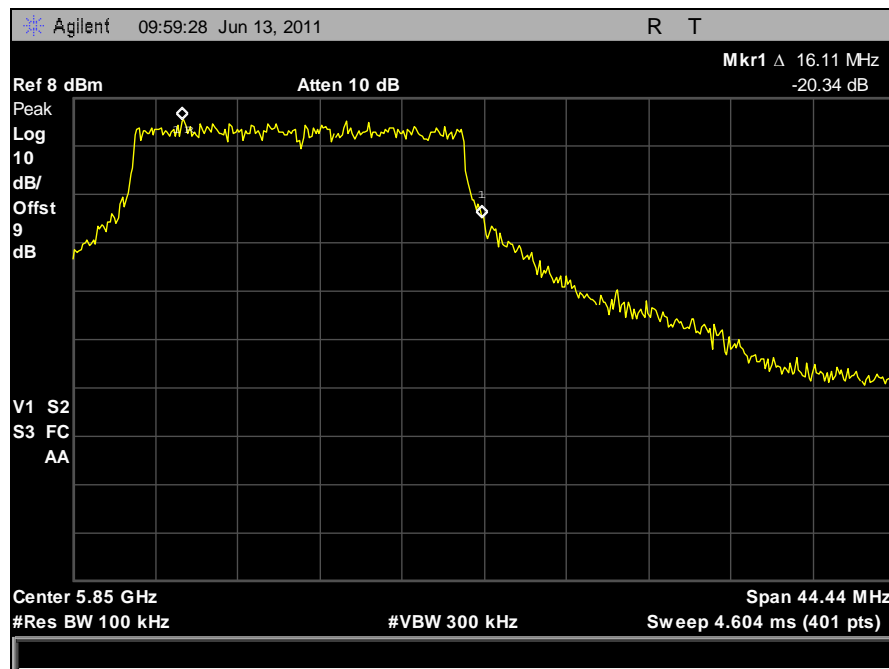
Plot 98. Conducted Band Edge, High Channel, 20 MHz, Horizontal Feed
