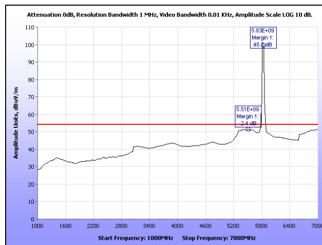
Plot 57. Radiated Spurious Emissions, High Channel, 1 GHz – 7 GHz, 40 MHz
