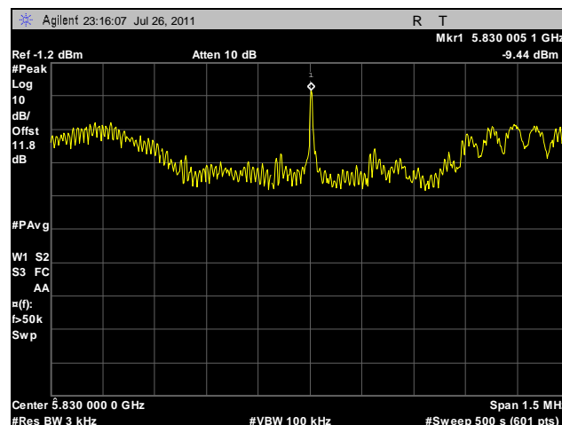
Plot 122. Peak Power Spectral Density, High Channel, 40 MHz, Horizontal Feed
