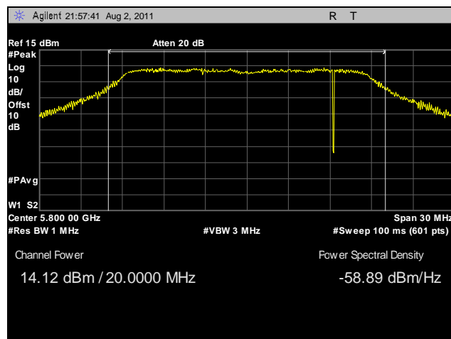
Plot 20. Peak Power Output, Mid Channel, 20 MHz, Horizontal Feed
