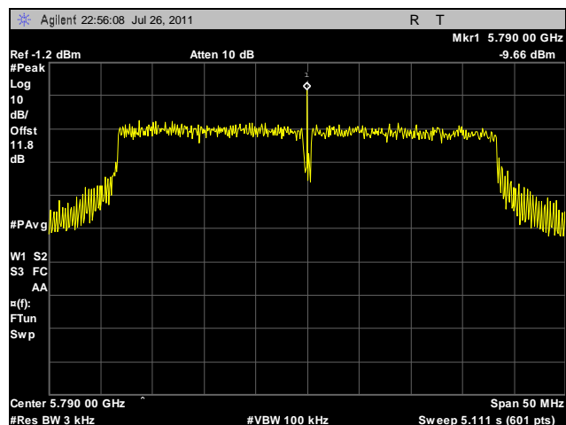
Plot 119. Peak Power Spectral Density, Mid Channel, 40 MHz, Horizontal Feed, Determination
