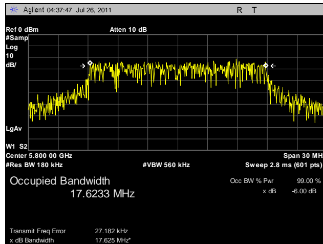
Plot 14. 99% Occupied Bandwidth, Mid Channel, 20 MHz
