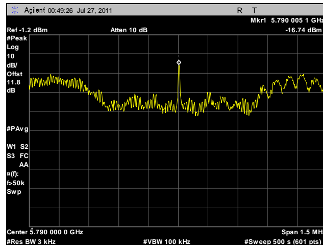
Plot 126. Peak Power Spectral Density, Mid Channel, 40 MHz, Vertical Feed
