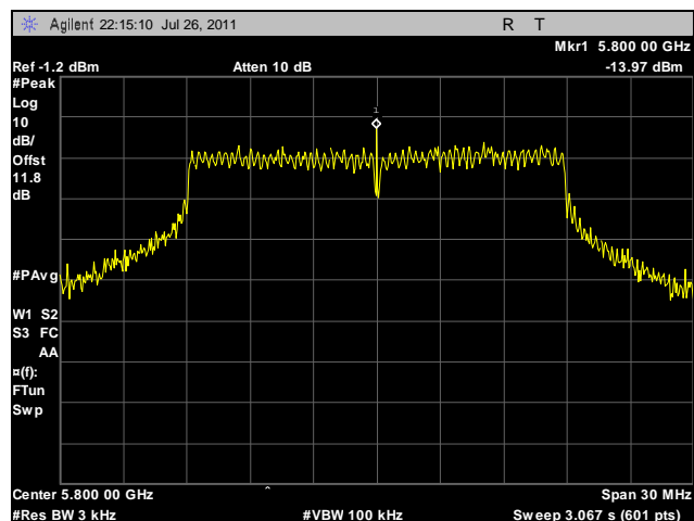
Plot 107. Peak Power Spectral Density, Mid Channel, 20 MHz, Horizontal Feed, Determination
