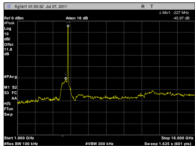
Plot 86. Conducted Spurious Emissions, High Channel, 1 GHz – 18 GHz, 40 MHz, Horizontal Feed
