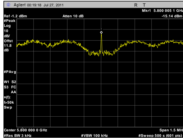
Plot 114. Peak Power Spectral Density, Mid Channel, 20 MHz, Vertical Feed
