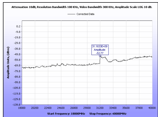
Plot 69. Conducted Spurious Emissions, High Channel, 18 GHz – 40 GHz, 20 MHz, Horizontal Feed
