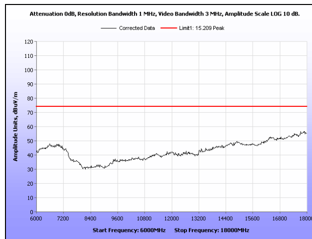
Plot 35. Radiated Spurious Emissions, Low Channel, 6 GHz – 18 GHz, Peak, 20 MHz
