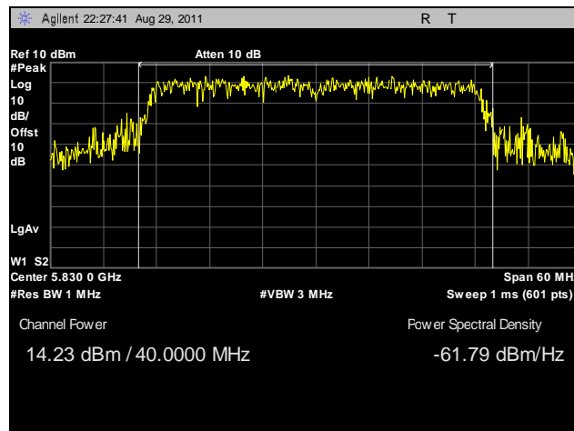
Plot 27. Peak Power Output, High Channel, 40 MHz, Horizontal Feed
