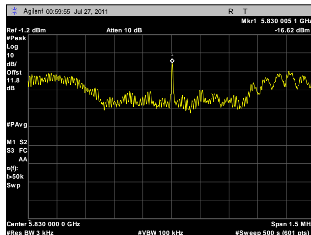
Plot 128. Peak Power Spectral Density, High Channel, 40 MHz, Vertical Feed
