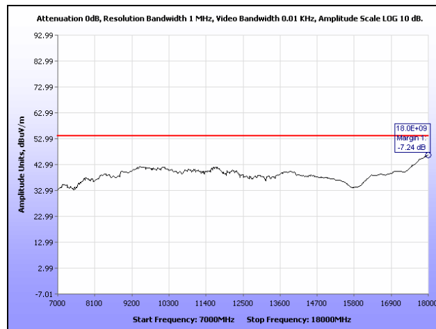
Plot 33. Radiated Spurious Emissions, Low Channel, 7 GHz – 18 GHz, 20 MHz
