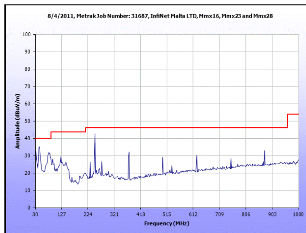
Plot 36. Radiated Spurious Emissions, Mid Channel, 30 MHz – 1 GHz, 20 MHz
