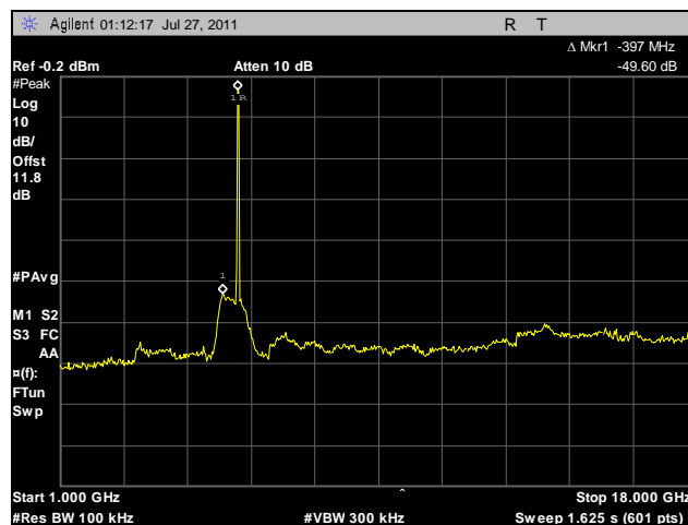
Plot 71. Conducted Spurious Emissions, Low Channel, 1 GHz – 18 GHz, 20 MHz, Vertical Feed
