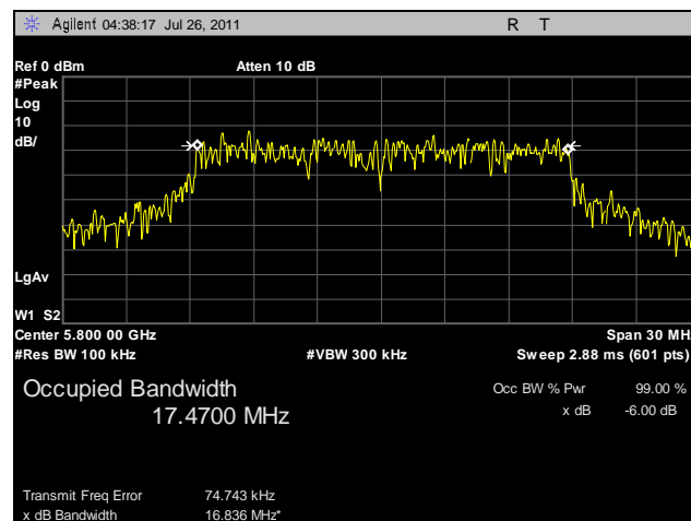
Plot 8. 6 dB Occupied Bandwidth, Mid Channel, 20 MHz
