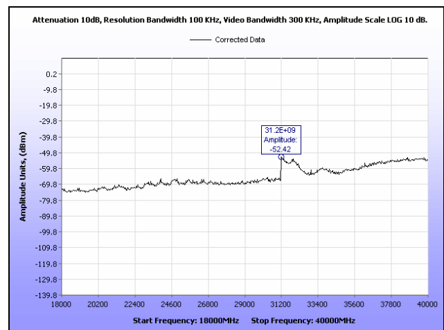
Plot 96. Conducted Spurious Emissions, High Channel, 18 GHz – 40 GHz, 40 MHz, Vertical Feed
