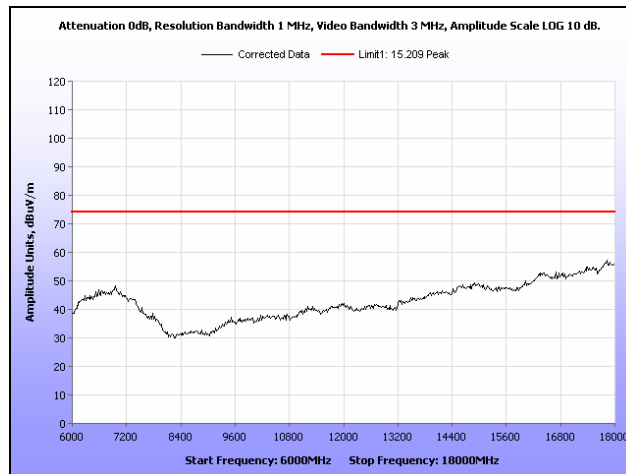
Plot 60. Radiated Spurious Emissions, High Channel, 6 GHz – 18 GHz, Peak, 40 MHz
