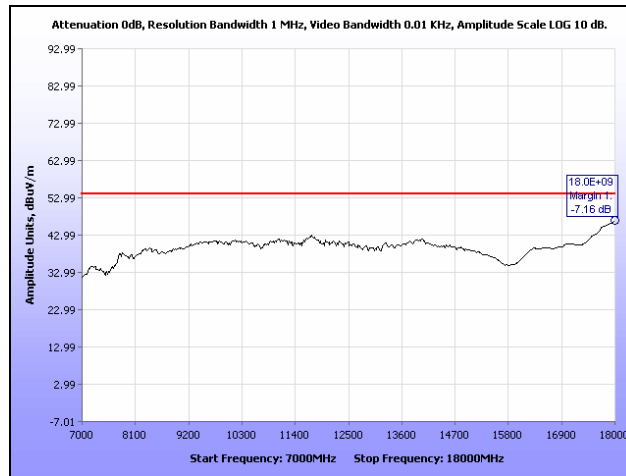
Plot 38. Radiated Spurious Emissions, Mid Channel, 7 GHz – 18 GHz, 20 MHz
