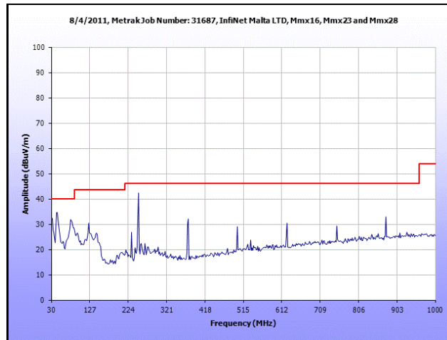
Plot 31. Radiated Spurious Emissions, Low Channel, 30 MHz – 1 GHz, 20 MHz
