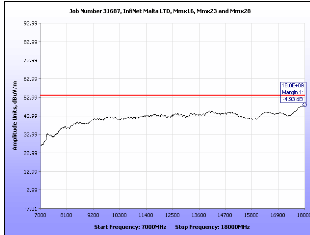
Plot 58. Radiated Spurious Emissions, High Channel, 7 GHz – 18 GHz, 40 MHz
