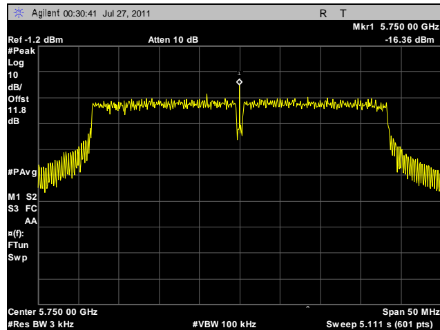
Plot 123. Peak Power Spectral Density, Low Channel, 40 MHz, Vertical Feed, Determination
