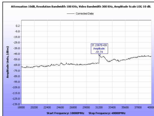
Plot 81. Conducted Spurious Emissions, Low Channel, 18 GHz – 40 GHz, 40 MHz, Horizontal Feed
