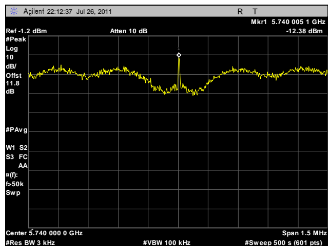
Plot 106. Peak Power Spectral Density, Low Channel, 20 MHz, Horizontal Feed
