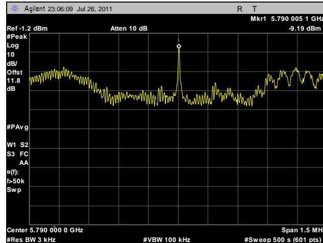
Plot 120. Peak Power Spectral Density, Mid Channel, 40 MHz, Horizontal Feed
