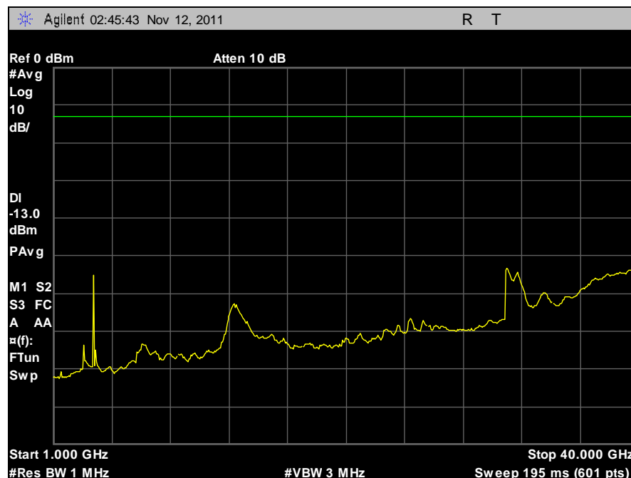
Plot 50. Conducted Spurious Emissions, 5 MHz, High Channel, Horizontal, 1 GHz – 40 GHz
