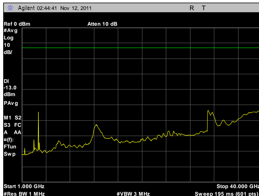
Plot 46. Conducted Spurious Emissions, 5 MHz, Low Channel, Vertical, 1 GHz – 40 GHz
