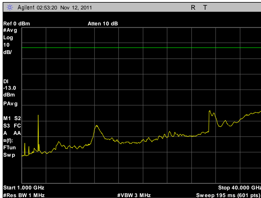
Plot 60. Conducted Spurious Emissions, 20 MHz, Low Channel, Horizontal, 1 GHz – 40 GHz
