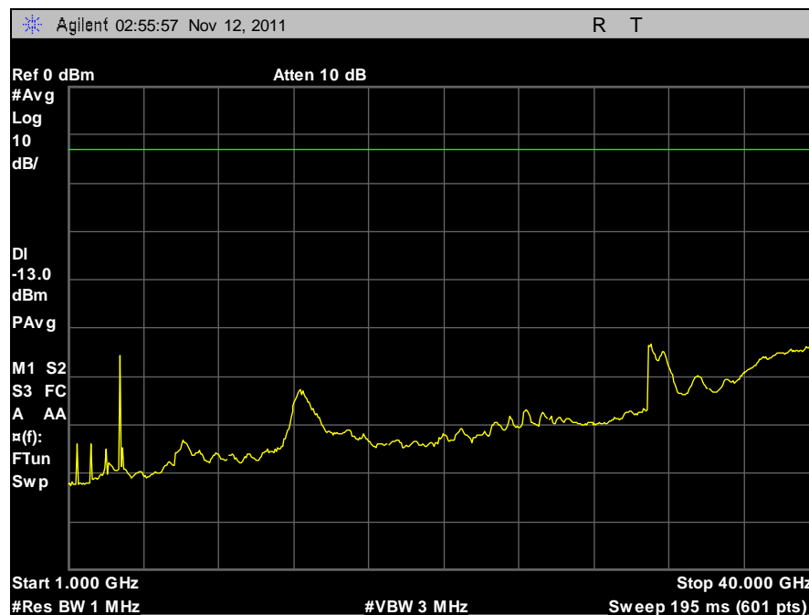
Plot 52. Conducted Spurious Emissions, 10 MHz, Low Channel, Horizontal, 1 GHz – 40 GHz
