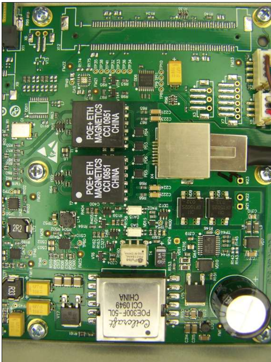
Photograph 2. Mmx2x22 board close-up
