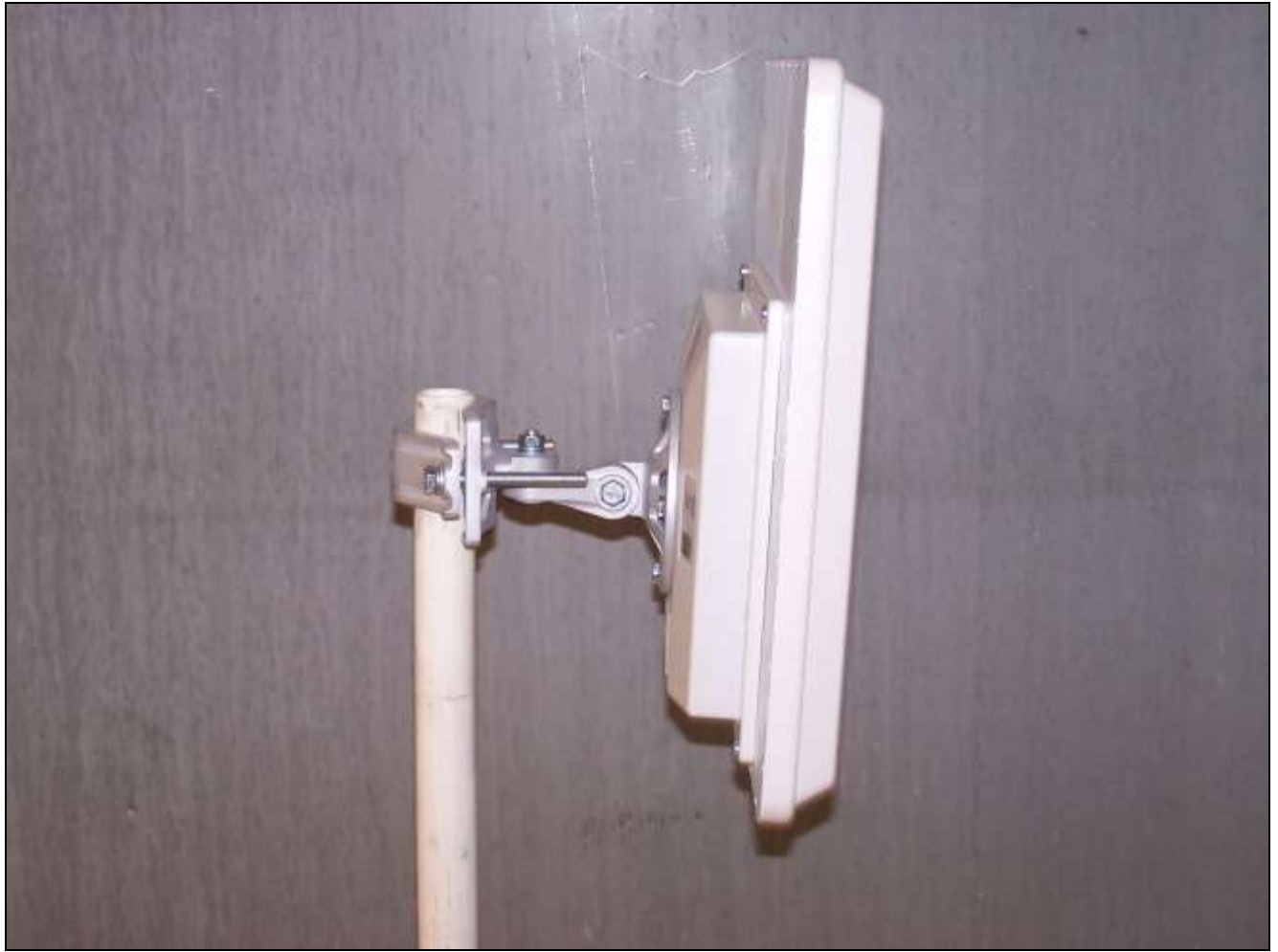
Photograph 5. Mmx2x22 mount side
