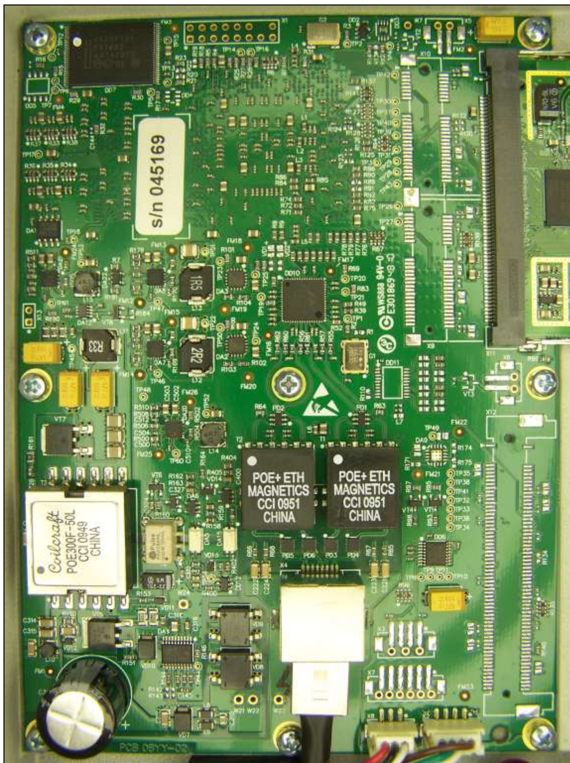
Photograph 3. Mmx2x22 board uncovered
