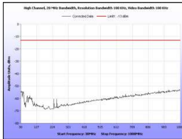
Plot 80. Radiated Spurious Emissions, 20 MHz, High Channel, 30 MHz – 1 GHz
