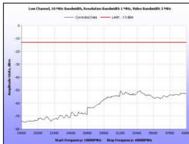
Plot 73. Radiated Spurious Emissions, 10 MHz, Low Channel, 18 GHz – 40 GHz
