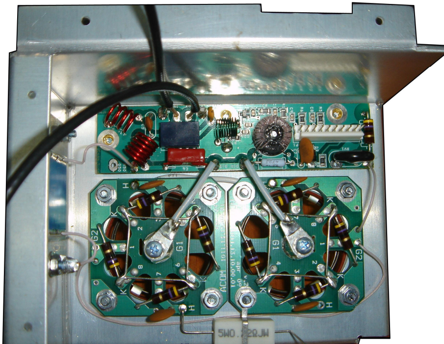
Fig.6 Bottom View – Tube Deck (screen cover removed)
