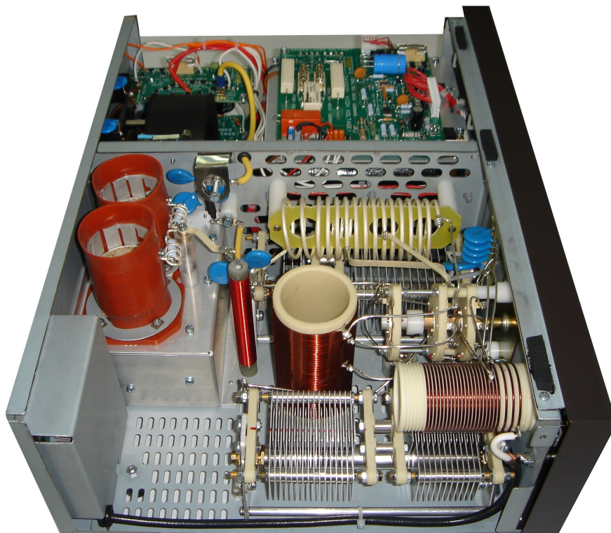
Fig.1 Right side View
