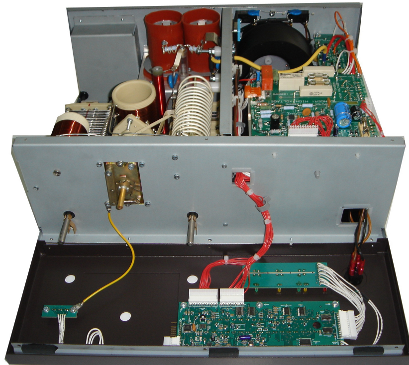
Fig.3 Front panel lay down
