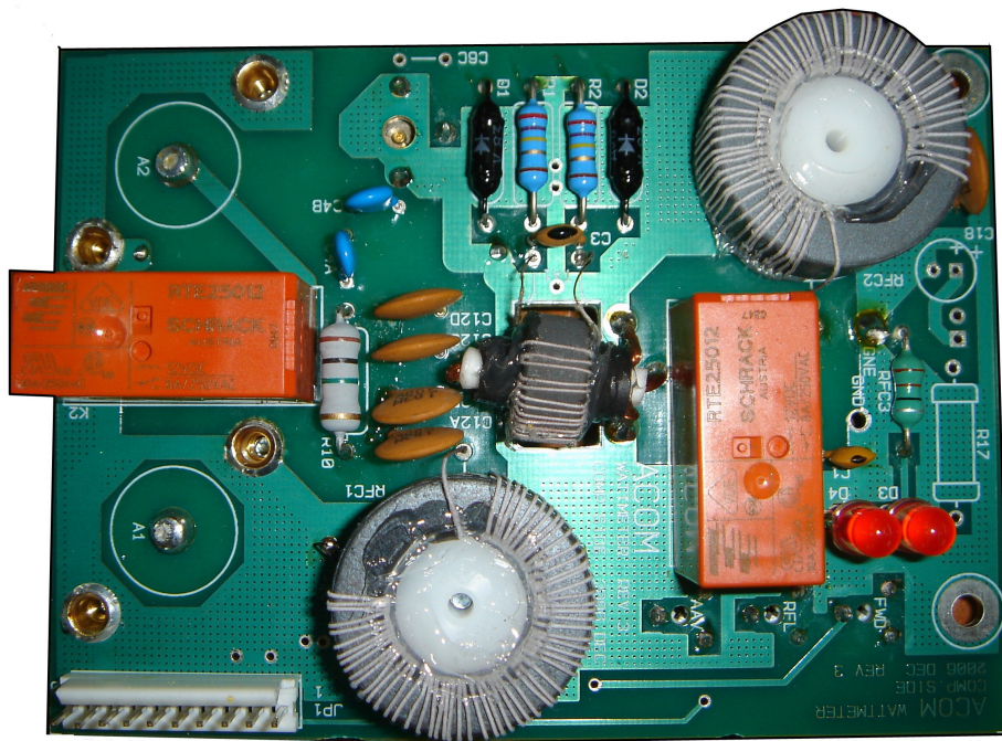
Fig.5 Wattmeter & ant.selection (screen cover removed)
