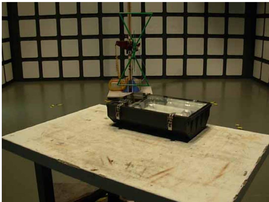
SETUP WITH MAXIMUM DETECTED EMISSION AT VERTICAL POLARIZATION (M/N: SP779#)
