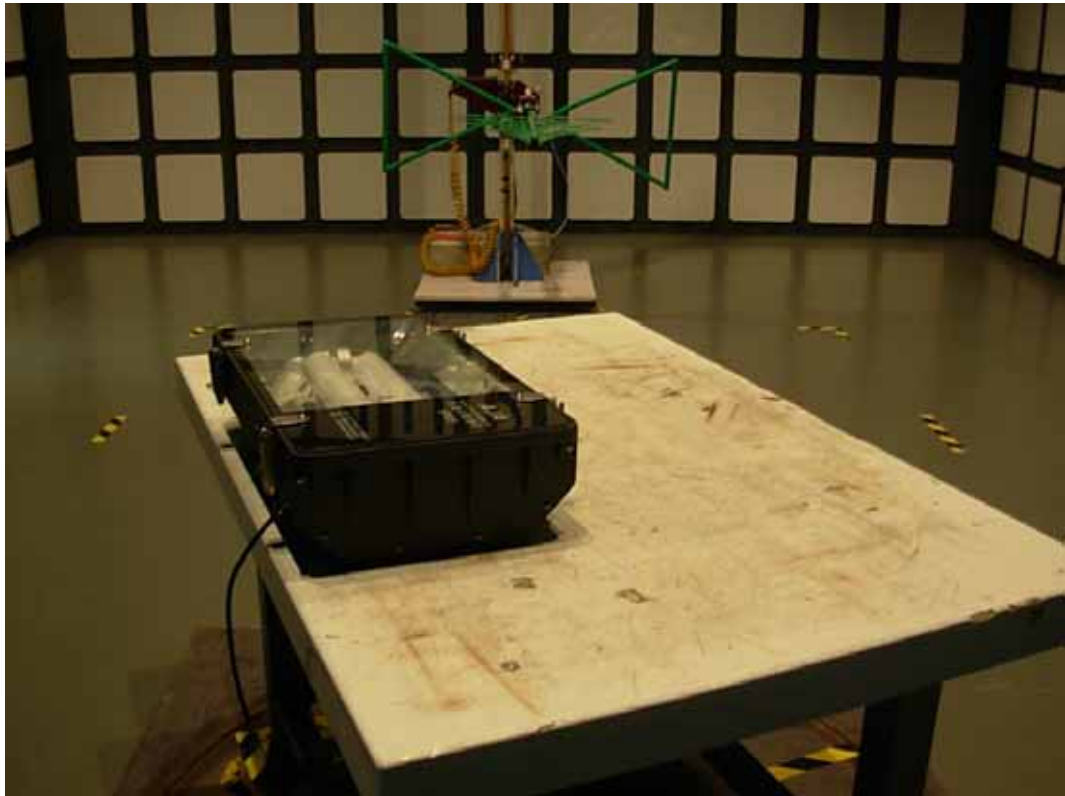
SETUP WITH MAXIMUM DETECTED EMISSION AT HORIZONTAL POLARIZATION (M/N: SP779#)
