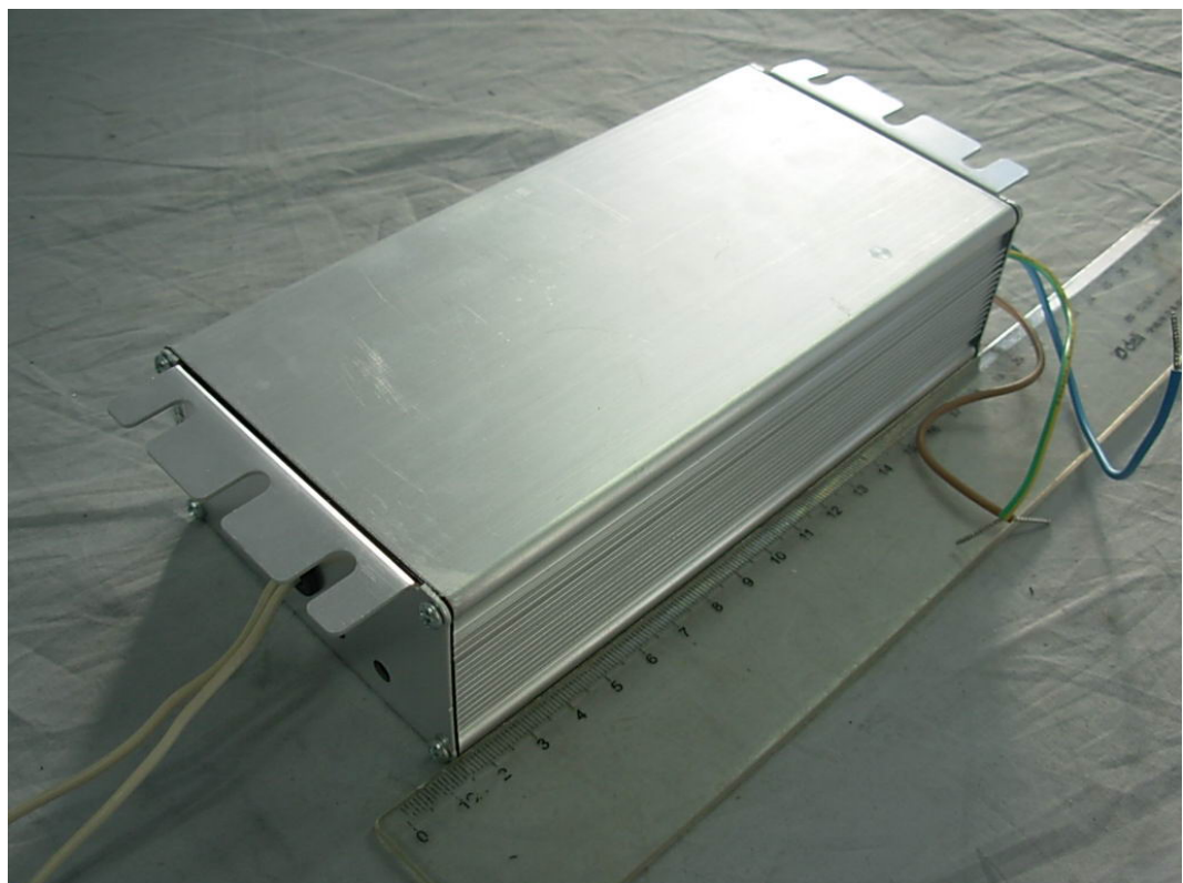
FIGURE 5 ELECTRIC DISCHARGE LAMP CONTROL EQUIPMENT (M/N: SP780#) GENERAL APPEARANCE (BACK VIEW)
