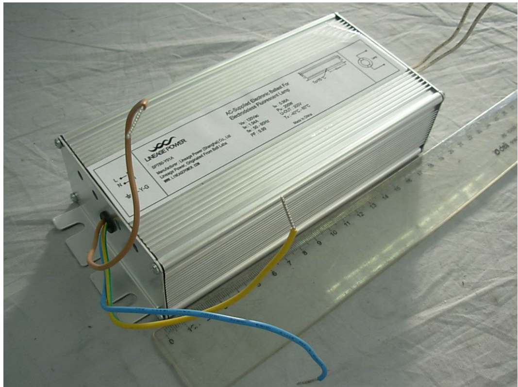
FIGURE 4 ELECTRIC DISCHARGE LAMP CONTROL EQUIPMENT (M/N: SP780#) GENERAL APPEARANCE (FRONT VIEW)
