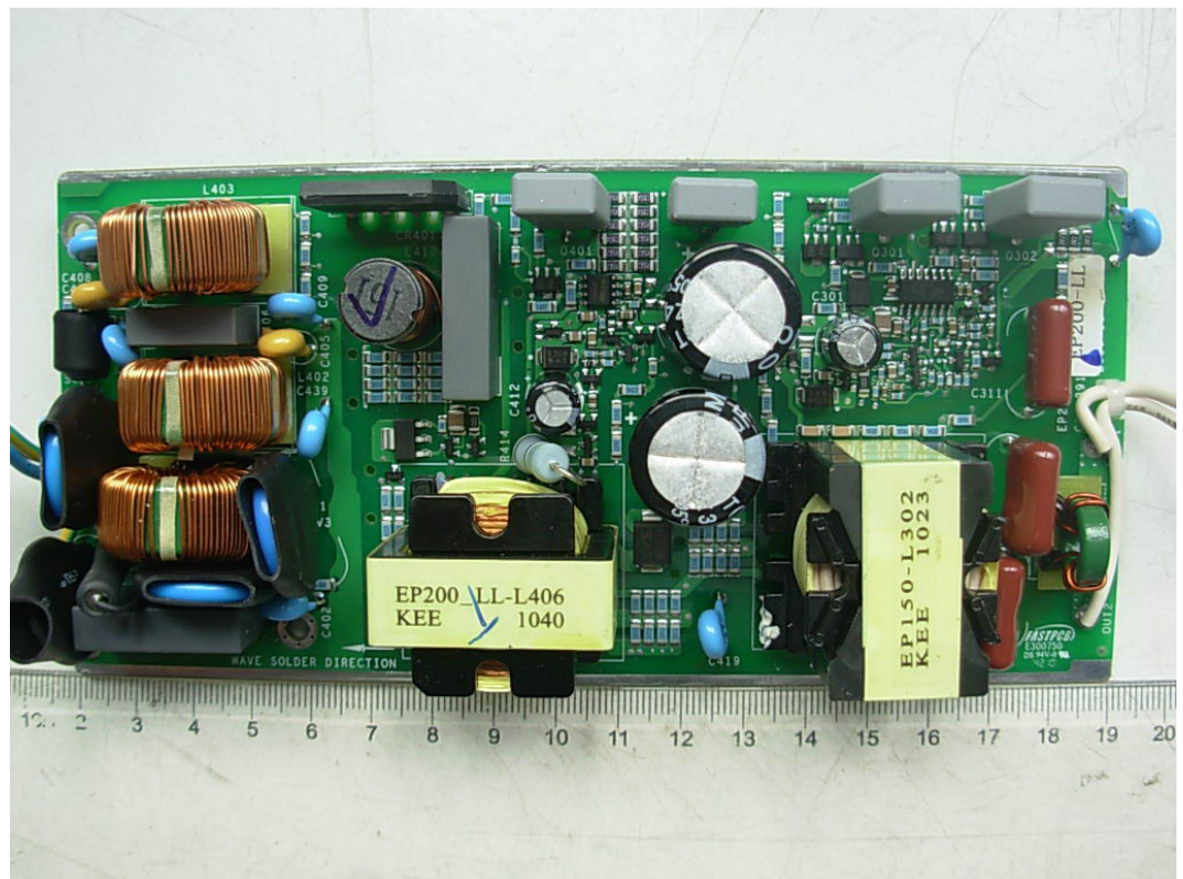
FIGURE 3 ELECTRIC DISCHARGE LAMP CONTROL EQUIPMENT (M/N: SP779#) MAIN BOARD (COMPONENT SIDE)
