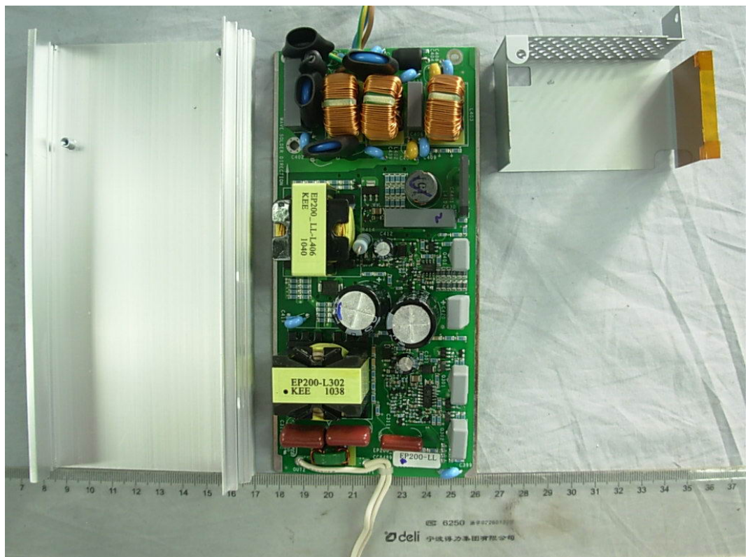
FIGURE 6 ELECTRIC DISCHARGE LAMP CONTROL EQUIPMENT (M/N: SP780#) MAIN BOARD REMOVED
