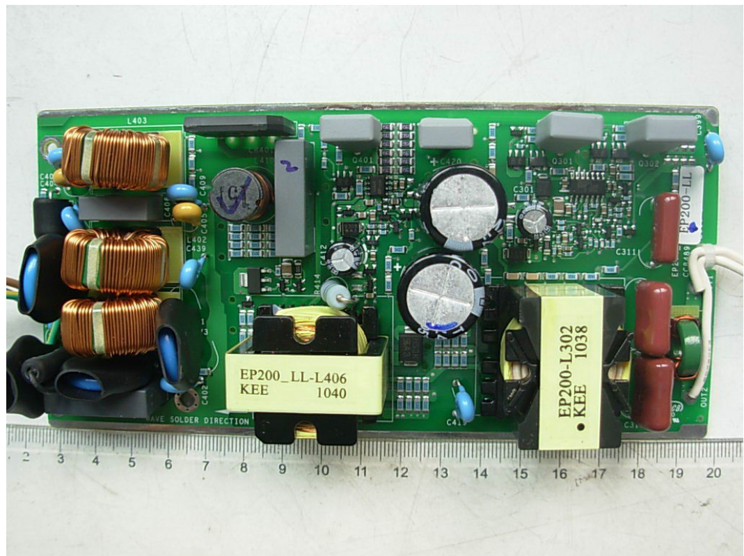
FIGURE 7 ELECTRIC DISCHARGE LAMP CONTROL EQUIPMENT (M/N: SP780#) MAIN BOARD (COMPONENT SIDE)
