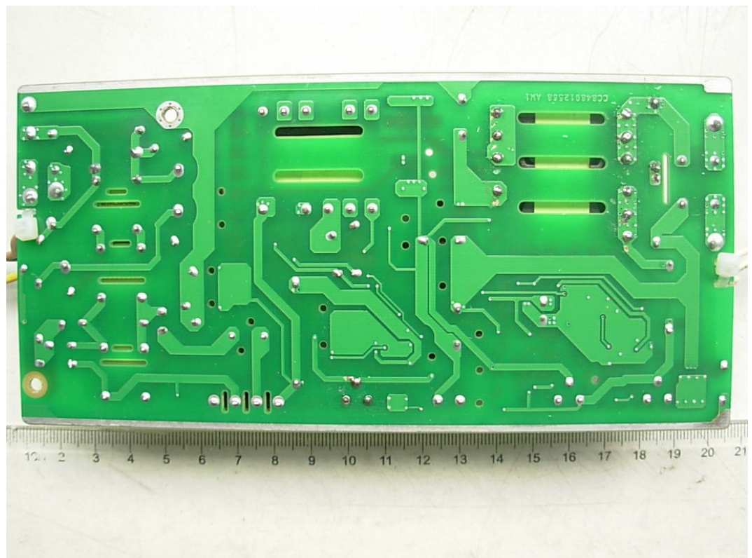
FIGURE 4 ELECTRIC DISCHARGE LAMP CONTROL EQUIPMENT (M/N: SP779#) MAIN BOARD (SOLDERED SIDE)
