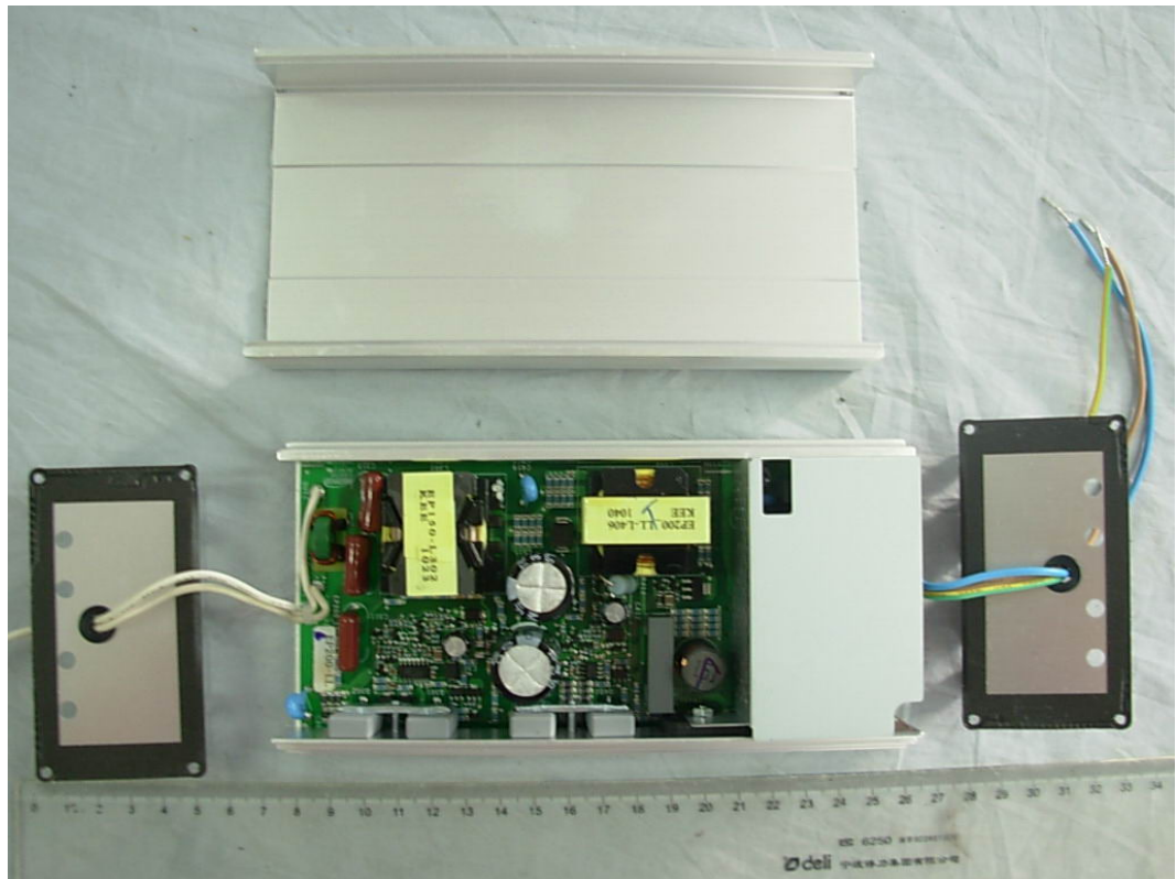
FIGURE 1 ELECTRIC DISCHARGE LAMP CONTROL EQUIPMENT (M/N: SP779#) COVER REMOVED
