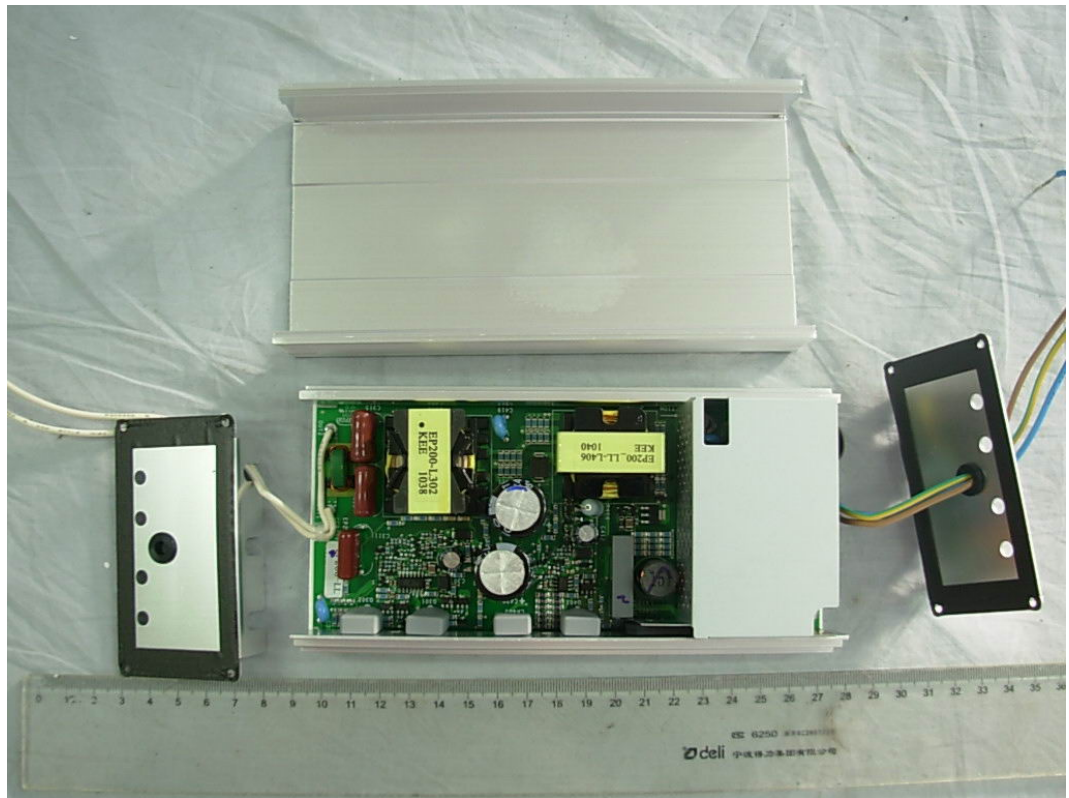
FIGURE 5 ELECTRIC DISCHARGE LAMP CONTROL EQUIPMENT (M/N: SP780#) COVER REMOVED
