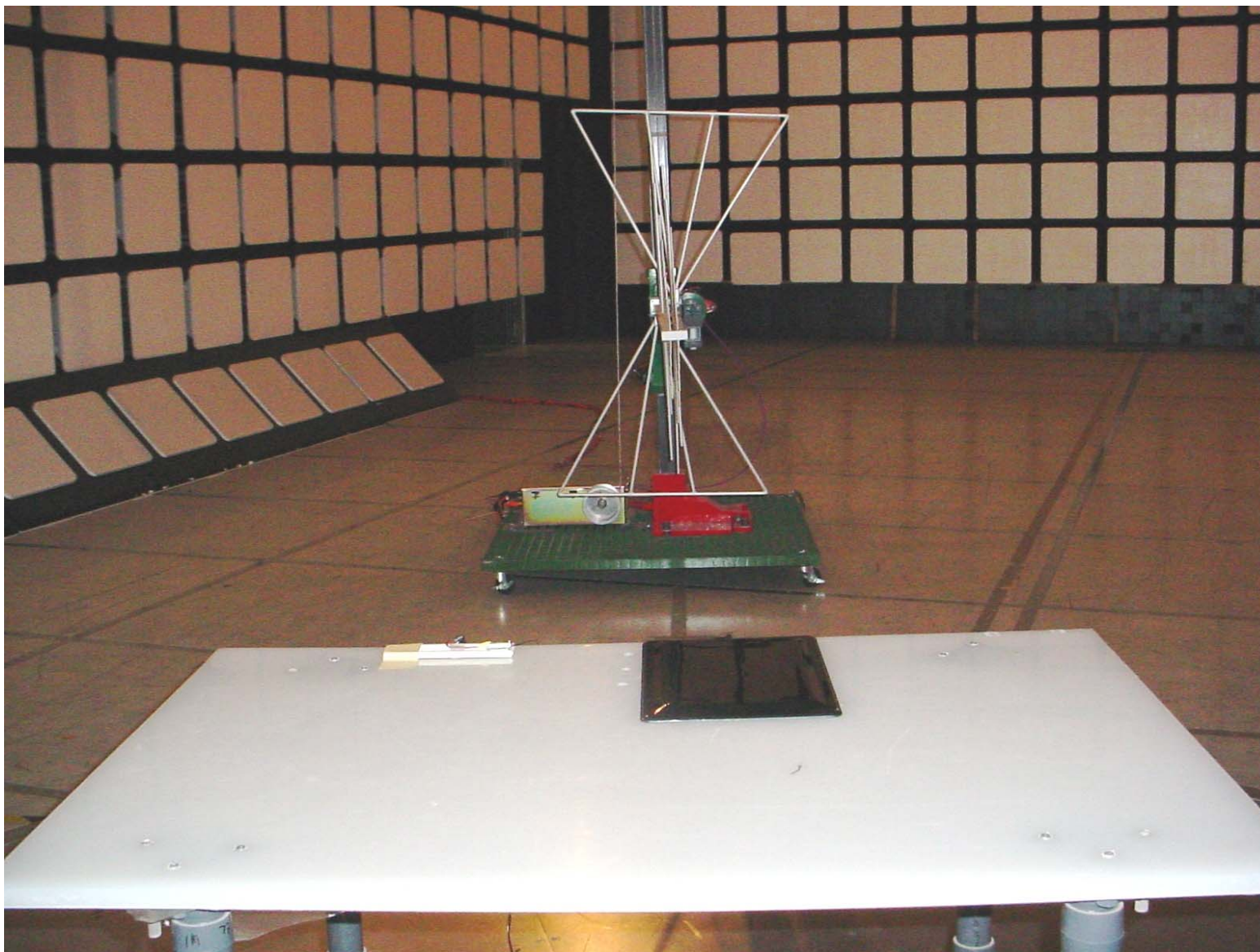
Photo #1: Radiated Emissions, Orthogonal Position #1, Desktop Antenna
