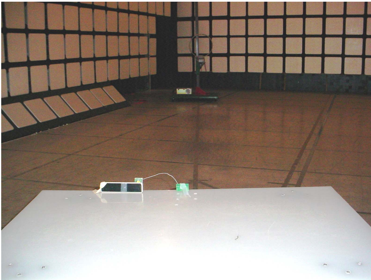
Photo #11: Radiated Emissions, Orthogonal Position #2, Embedded Loop Antenna
