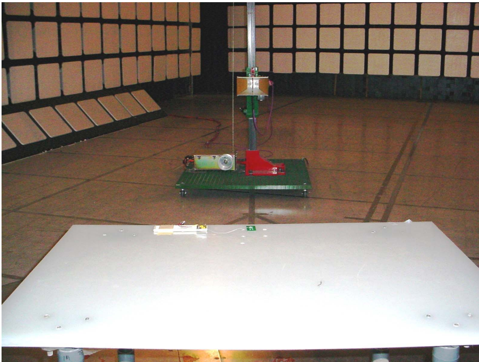
Photo #9: Radiated Emissions, Orthogonal Position #1, Embedded Loop Antenna
