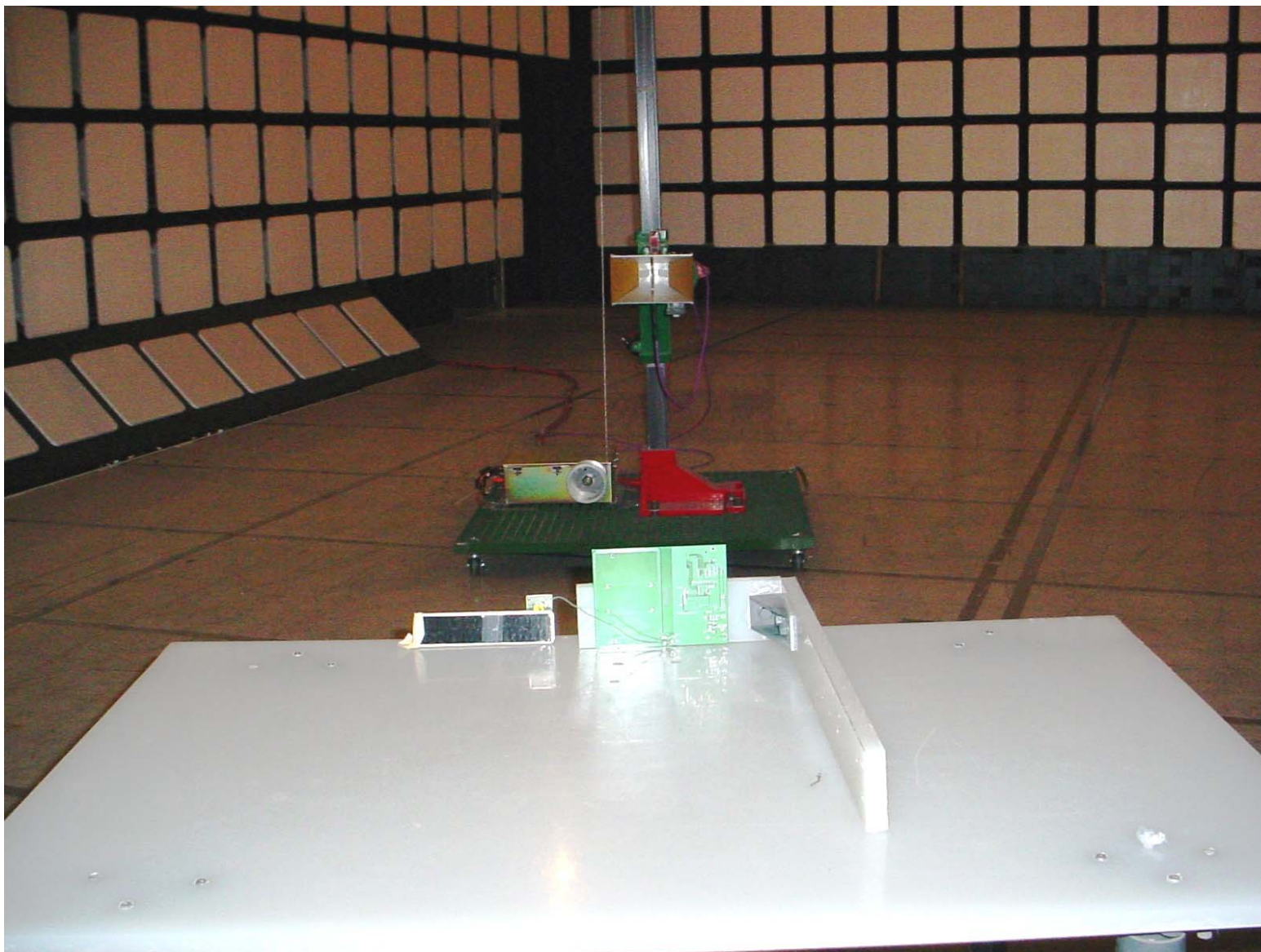
Photo #8: Radiated Emissions, Orthogonal Position #3, Embedded PCB Antenna
