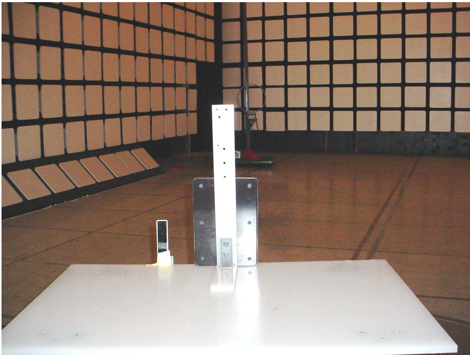
Photo #3: Radiated Emissions, Orthogonal Position #2, Desktop Antenna
