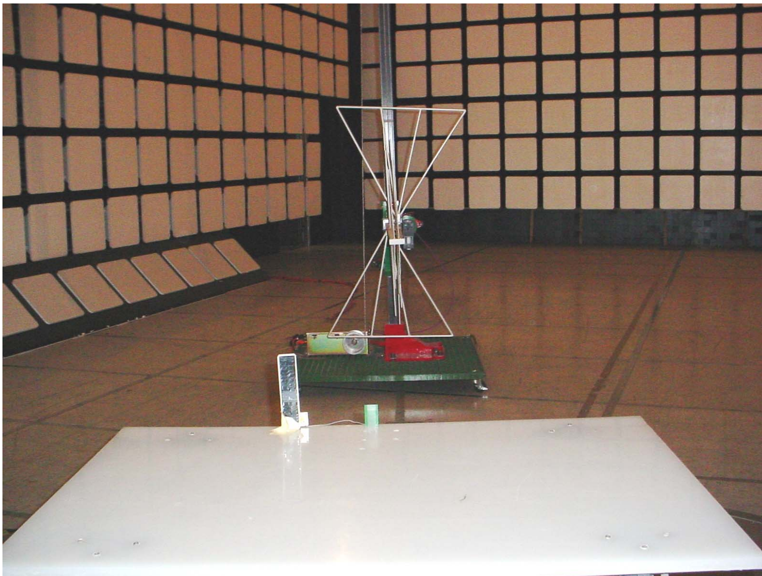
Photo #12: Radiated Emissions, Orthogonal Position #3, Embedded Loop Antenna
