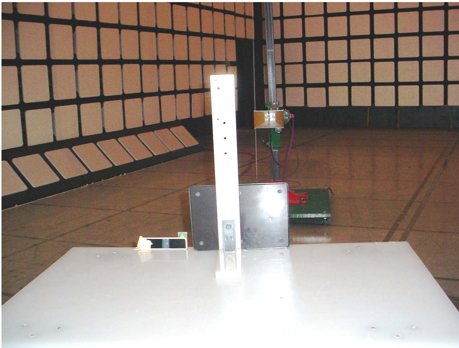
Photo #4: Radiated Emissions, Orthogonal Position #3, Desktop Antenna
