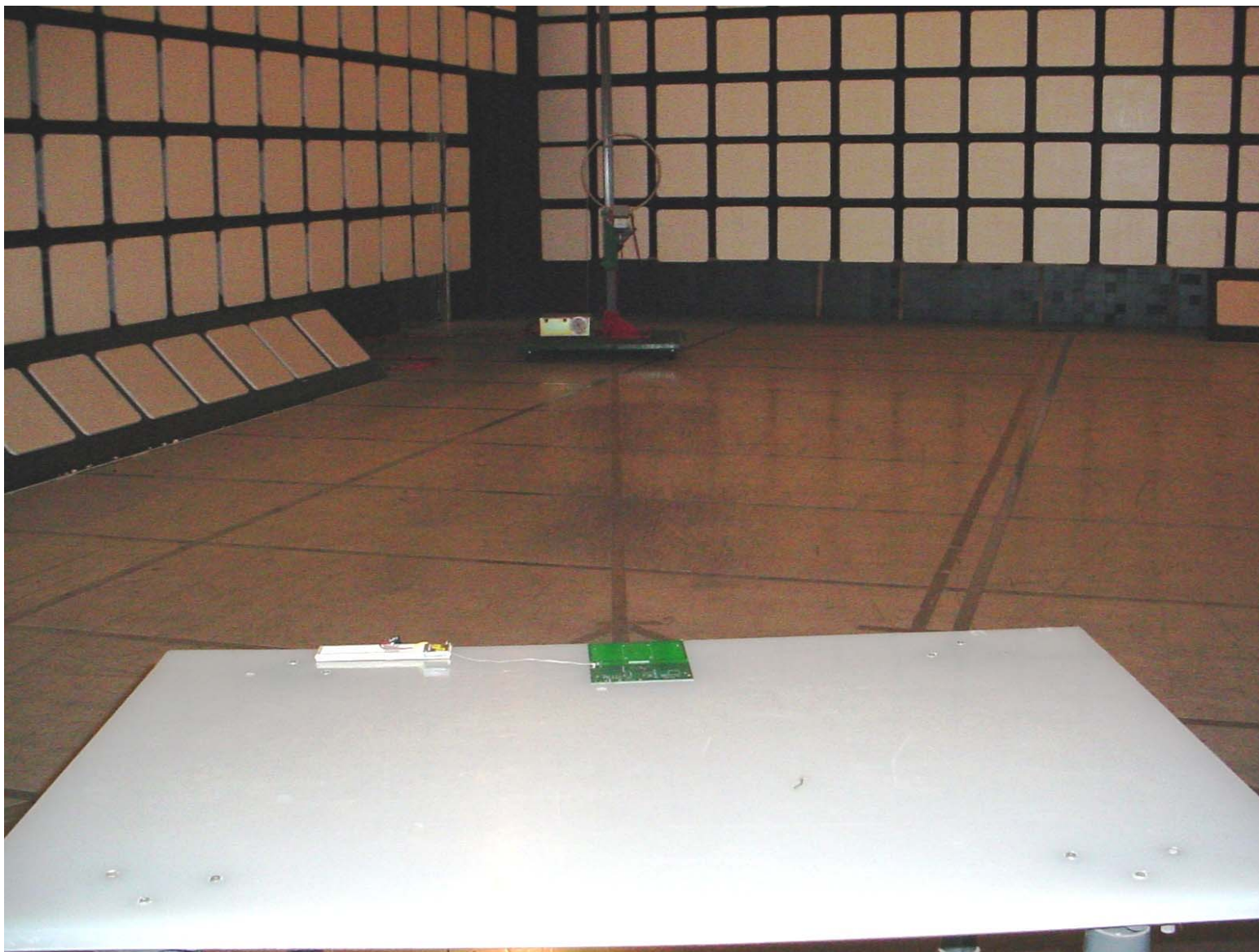
Photo #5: Radiated Emissions, Orthogonal Position #1, Embedded PCB Antenna
