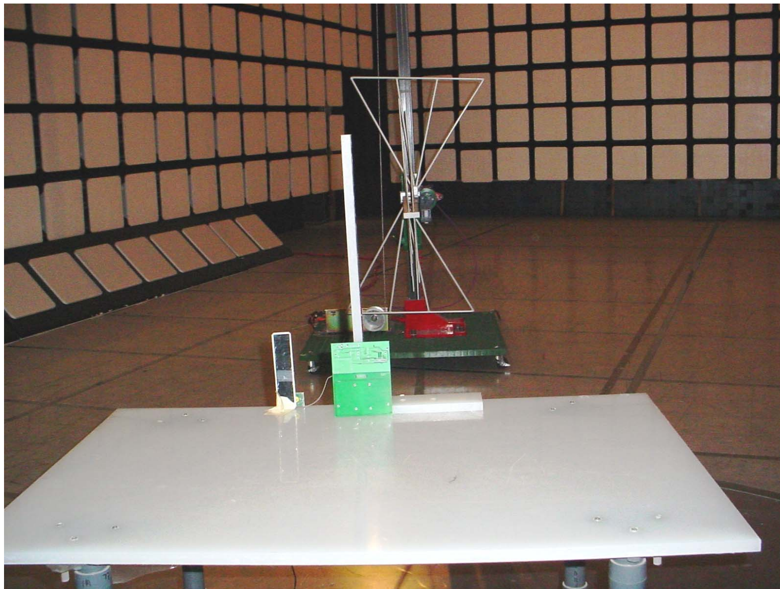
Photo #7: Radiated Emissions, Orthogonal Position #2, Embedded PCB Antenna
