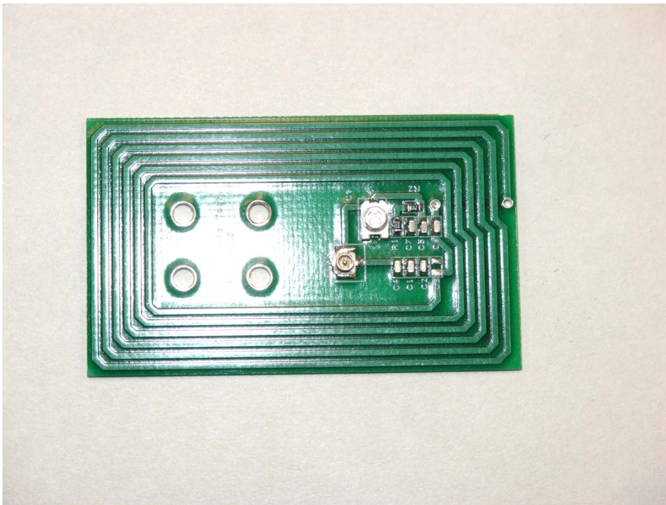
(PCB Loop Antenna ANTH2)
