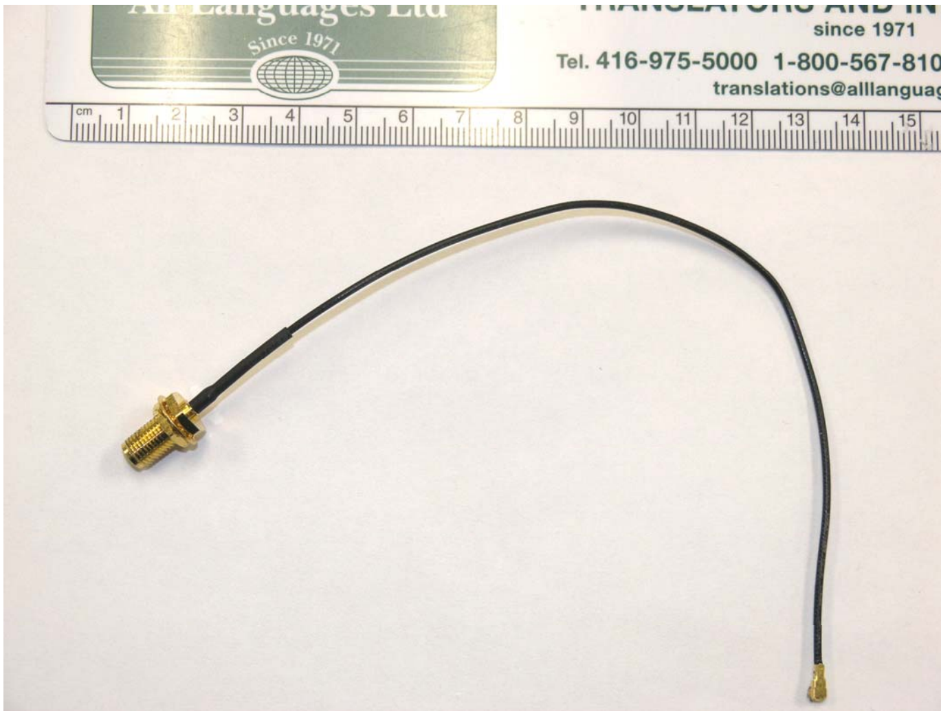
(U.FL to RPSMA connector with a co-axial cable)
