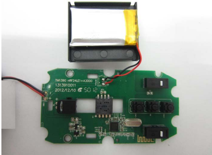
INTERNAL PHOTO OF TX SAMPLE – 3
