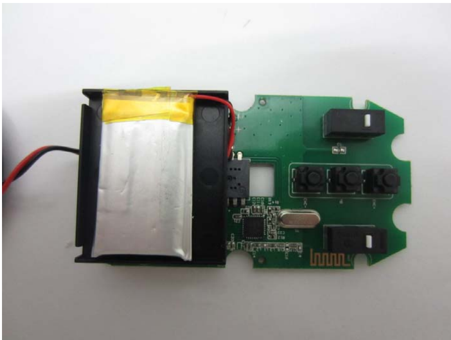
INTERNAL PHOTO OF TX SAMPLE – 2
