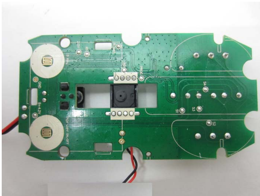
INTERNAL PHOTO OF TX SAMPLE – 4
