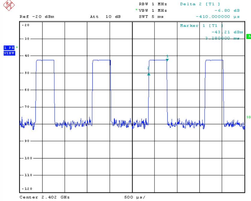
2402 MHz_DH1
