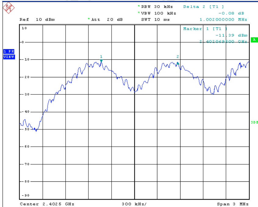
2402 MHz
