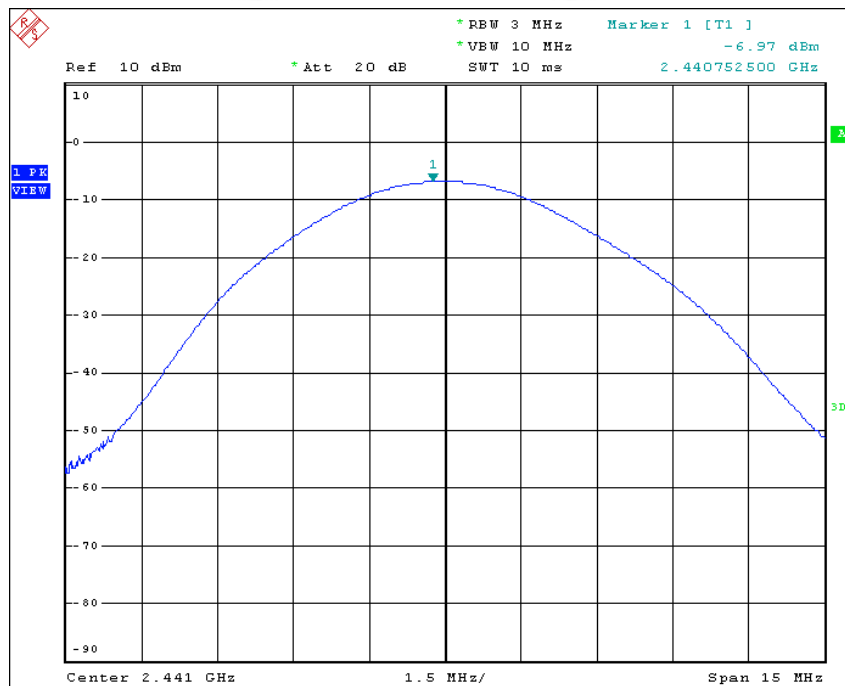
2441MHz
