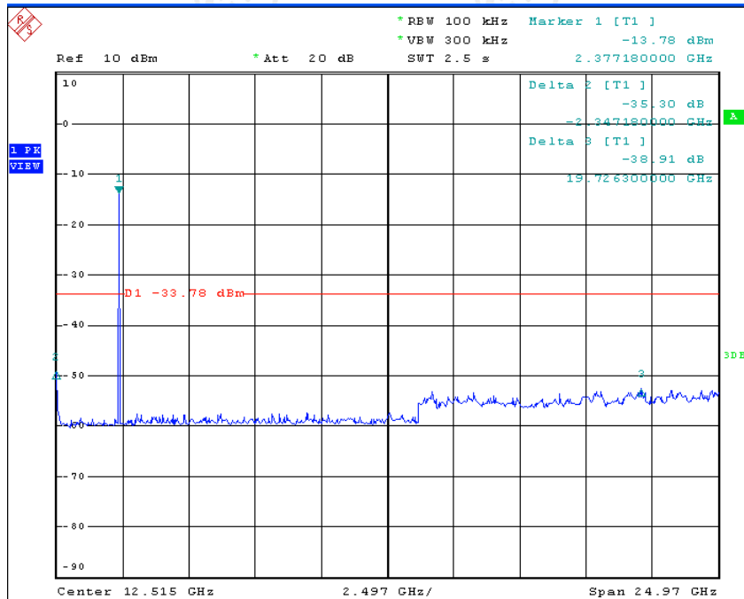
2441MHz
