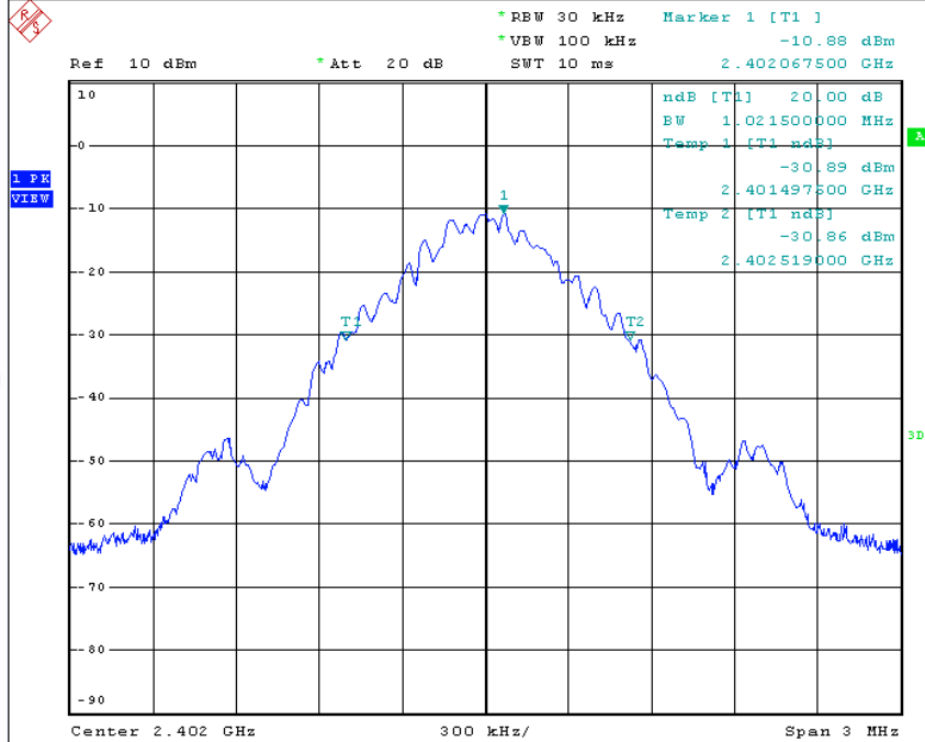
2402 MHz
