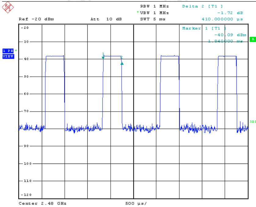
2480 MHz_DH1
